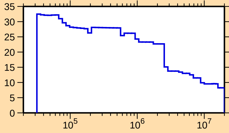
\Delta\sigma/\sigma vs. E for ^{153}\text{Pm}(n,\text{nonel.})
