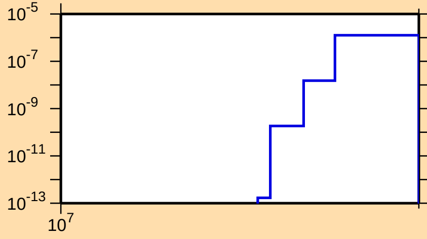
\sigma vs. E for ^{153}\text{Pm}(n,nt)
