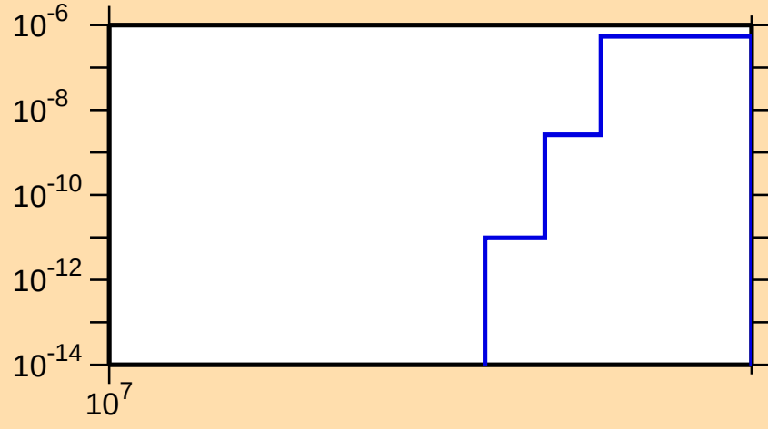
\sigma vs. E for ^{153}\text{Pm}(n,\text{nd})
