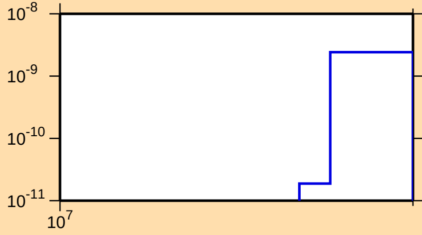
\sigma vs. E for ^{153}\text{Pm}(n,2n\alpha)
