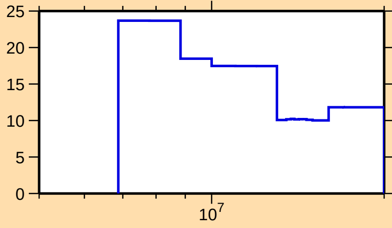
\Delta\sigma/\sigma vs. E for ^{153}\text{Pm}(n,\text{el.})
