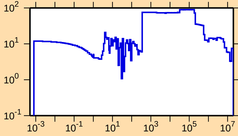
\Delta\sigma/\sigma vs. E for ^{153}\text{Pm}(n,\text{tot.})
