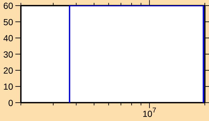
\Delta\sigma/\sigma vs. E for ^{153}\text{Pm}(n,p)
