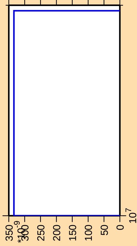
\Delta\sigma/\sigma vs. E for ^{153}\text{Pm} (mt 11)
