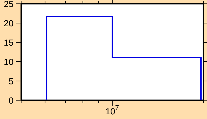
\Delta\sigma/\sigma vs. E for ^{153}\text{Pm}(n,\text{el.})
