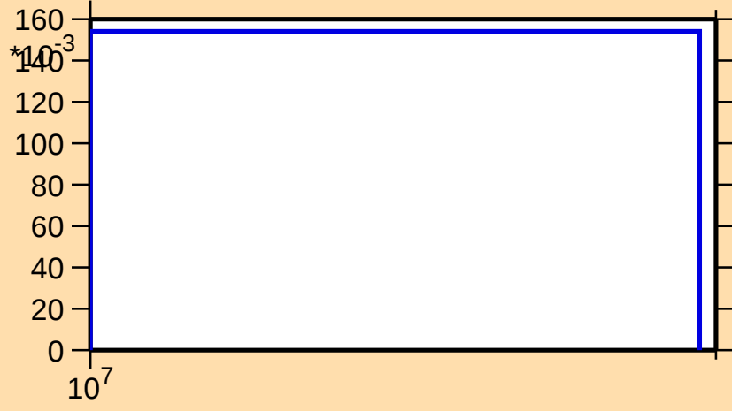
\sigma vs. E for ^{153}\text{Pm}(n,3n)
