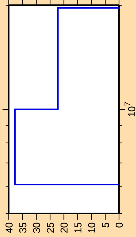
\Delta\sigma/\sigma vs. E for ^{153}\text{Pm}(n,2n)
