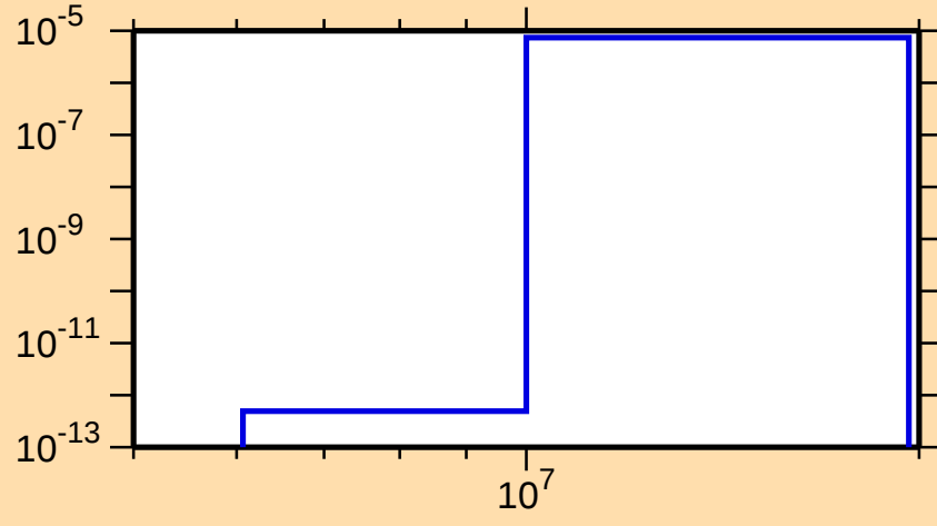
\sigma vs. E for ^{153}\text{Pm}(n,n\alpha)
