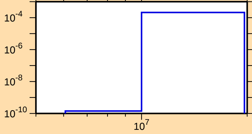
\sigma vs. E for ^{153}\text{Pm}(n,d)
