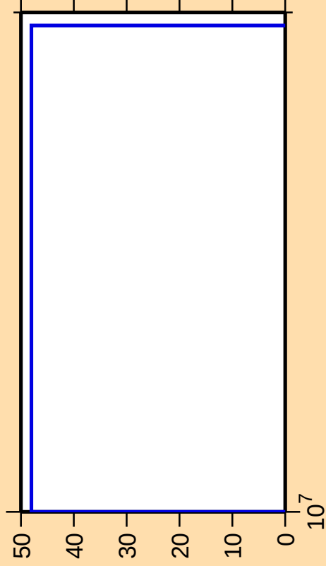
\Delta\sigma/\sigma vs. E for ^{153}\text{Pm}(n,3n)
