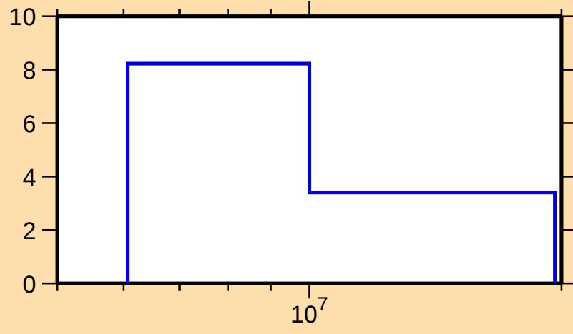
\Delta\sigma/\sigma vs. E for ^{153}\text{Pm}(n,\text{tot.})
