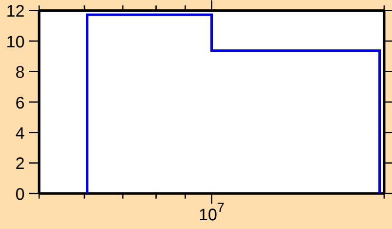
\Delta\sigma/\sigma vs. E for ^{153}\text{Pm}(n,\text{nonel.})
