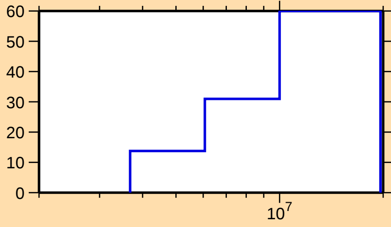
\Delta\sigma/\sigma vs. E for ^{153}\text{Pm}(n,n\text{cont.})
