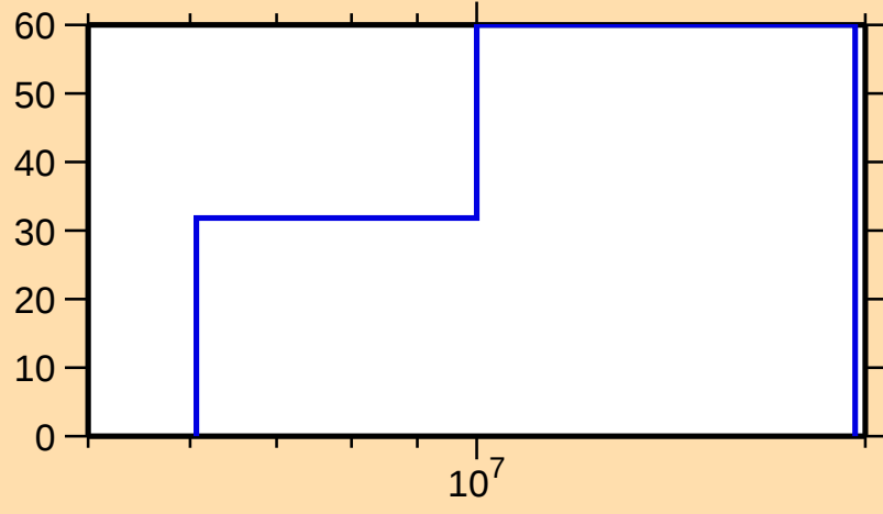
\Delta\sigma/\sigma vs. E for ^{153}\text{Pm}(n,\text{inel.})
