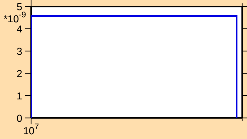
\sigma vs. E for ^{153}\text{Pm}(n,\text{nd})
