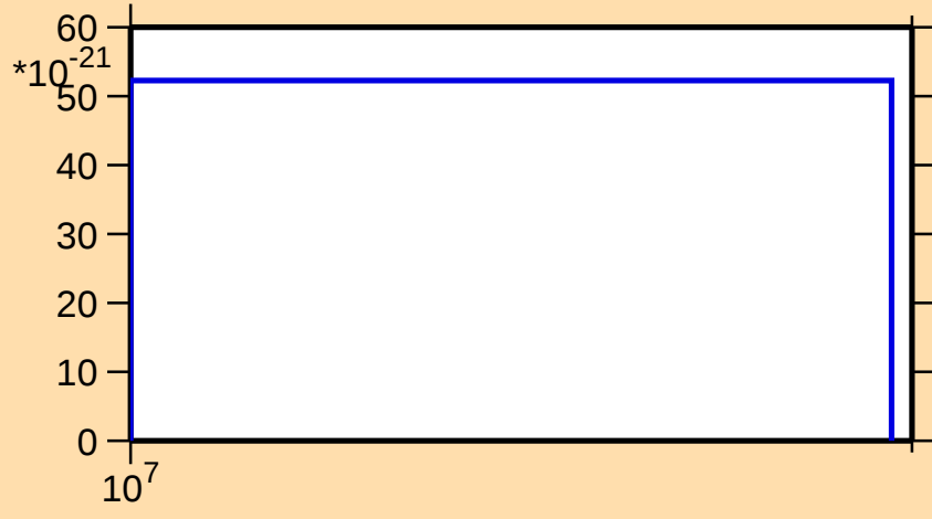
\sigma vs. E for ^{153}\text{Pm} (mt 11)
