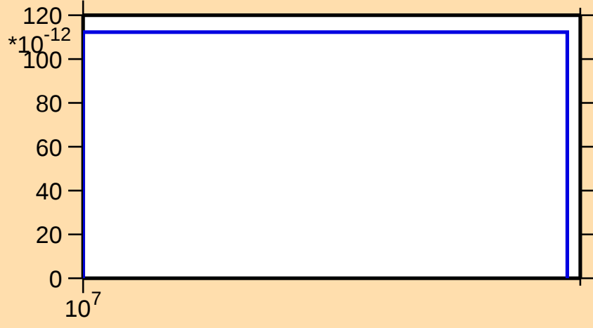
\sigma vs. E for ^{153}\text{Pm}(n,2np)
