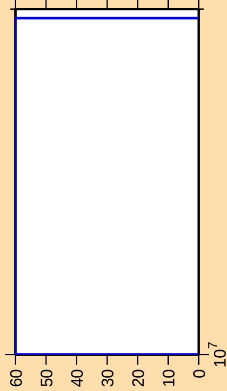
\Delta\sigma/\sigma vs. E for ^{153}\text{Pm}(n,\text{nd})
