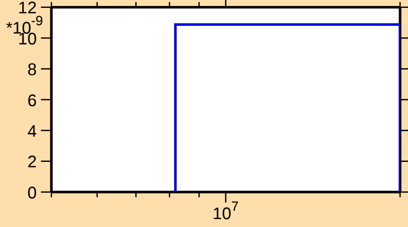
\sigma vs. E for ^{153}\text{Pm}(n,nt)
