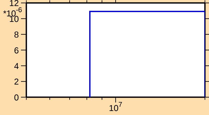
\sigma vs. E for ^{153}\text{Pm}(n,t)
