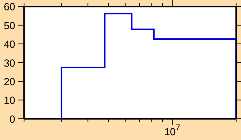
\Delta\sigma/\sigma vs. E for ^{153}\text{Pm}(n,n_1)
