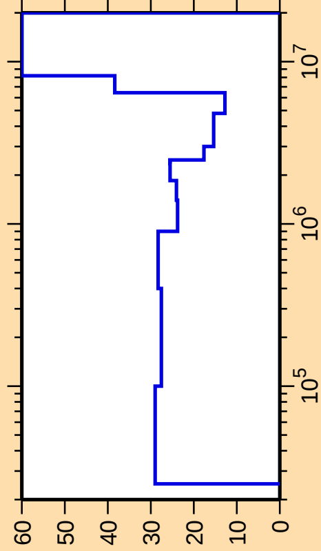
\Delta\sigma/\sigma vs. E for ^{153}\text{Pm}(n,\text{inel.})
