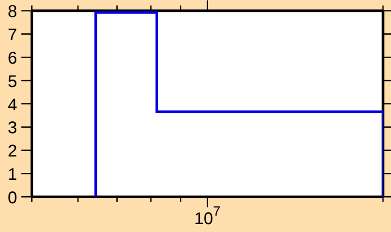
\Delta\sigma/\sigma vs. E for ^{153}\text{Pm}(n,\text{tot.})
