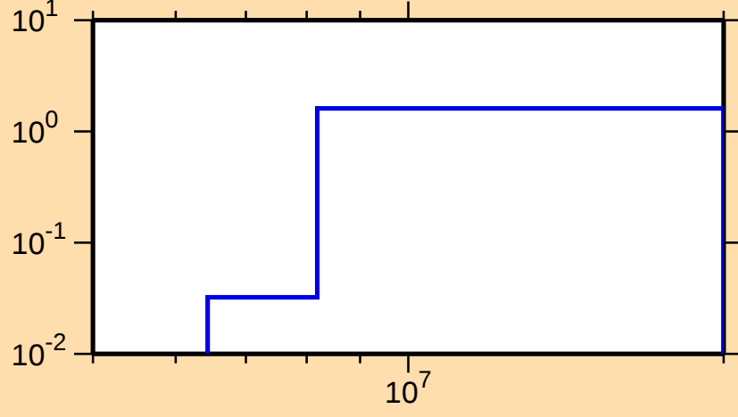
\sigma vs. E for ^{153}\text{Pm}(n,2n)
