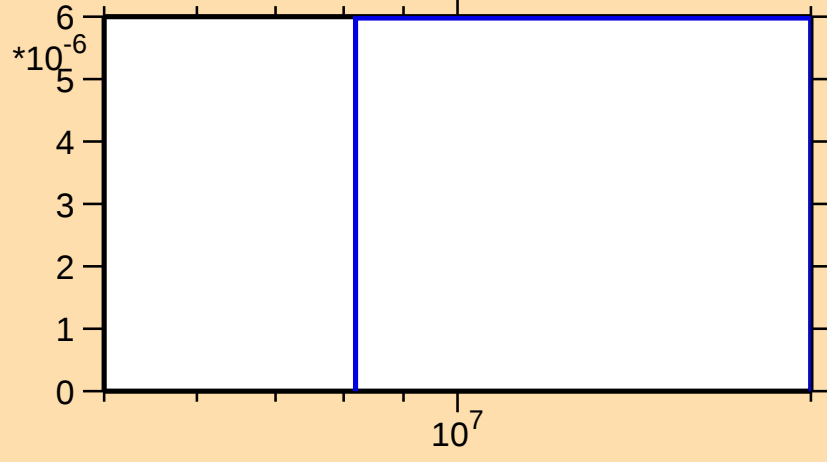
\sigma vs. E for ^{153}\text{Pm}(n,n\alpha)
