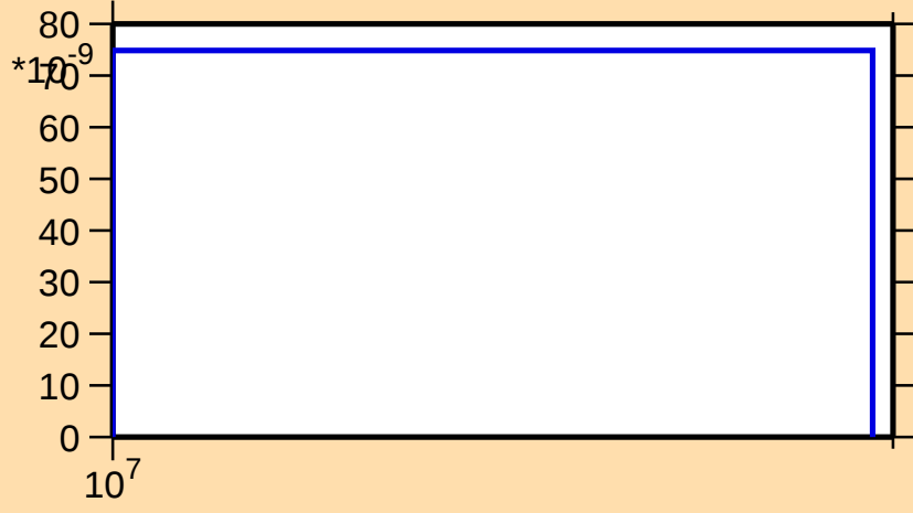
\sigma vs. E for ^{154}\text{Pm}(n,\text{nd})
