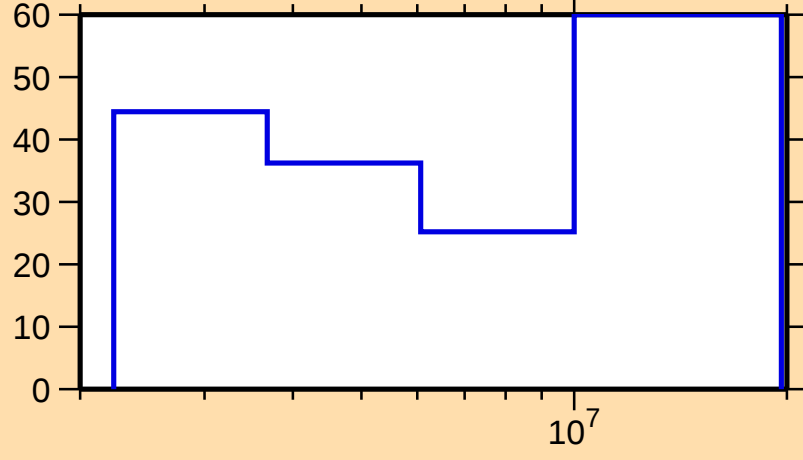
\Delta\sigma/\sigma vs. E for ^{154}\text{Pm}(n,n\text{cont.})
