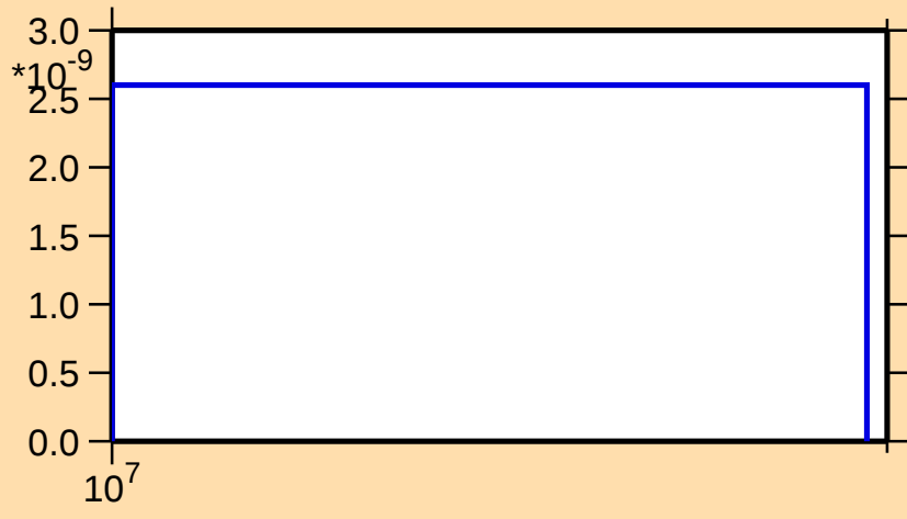
\sigma vs. E for ^{154}\text{Pm}(n,2np)
