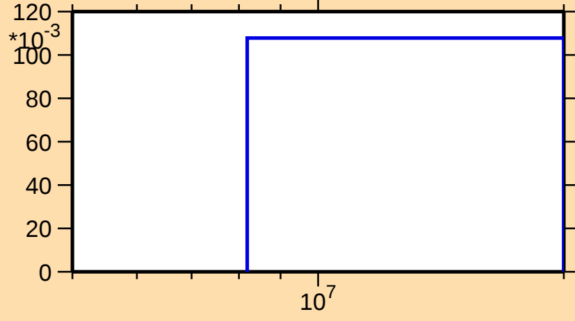
\sigma vs. E for ^{154}\text{Pm}(n,3n)
