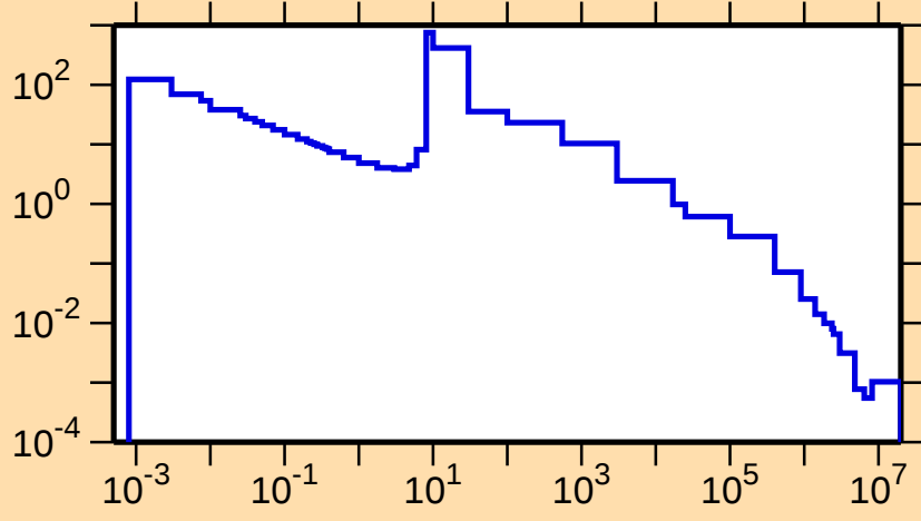
\sigma vs. E for ^{154}\text{Pm}(n,\gamma)
