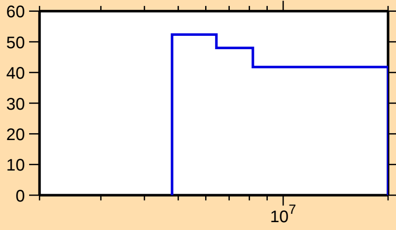
\Delta\sigma/\sigma vs. E for ^{154}\text{Pm}(n,2n)
