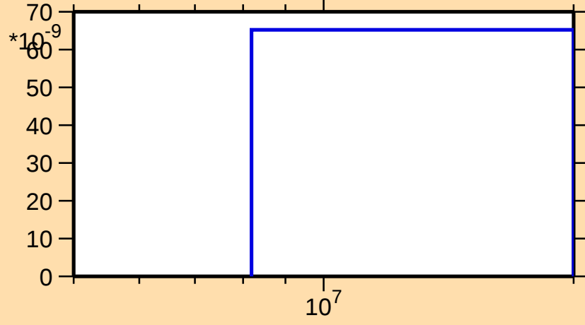
\sigma vs. E for ^{154}\text{Pm}(n,\text{nd})
