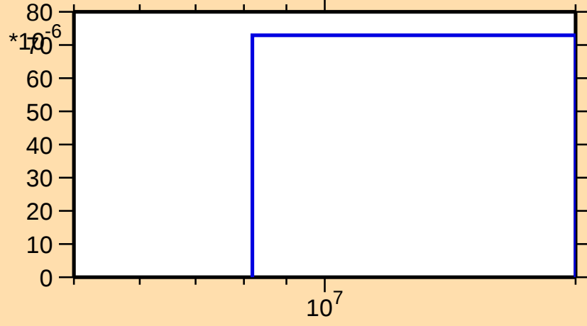
\sigma vs. E for ^{154}\text{Pm}(n,np)
