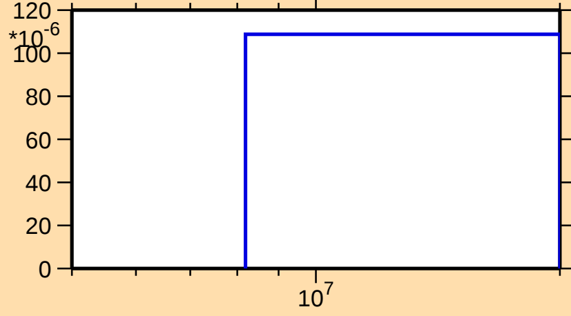
\sigma vs. E for ^{154}\text{Pm}(n,d)
