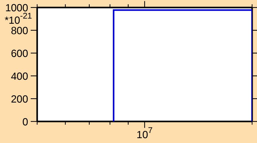
\sigma vs. E for ^{154}\text{Pm}(\text{mt } 11)
