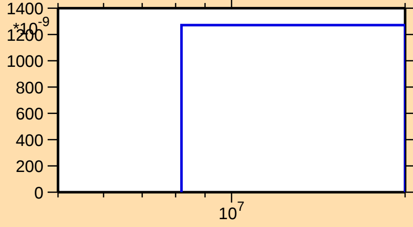
\sigma vs. E for ^{154}\text{Pm}(n,n\alpha)
