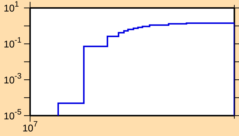
\sigma vs. E for ^{156}\text{Pm}(n,3n)
