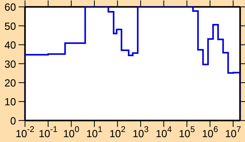
\Delta\sigma/\sigma vs. E for ^{156}\text{Pm}(n,\text{el.})
