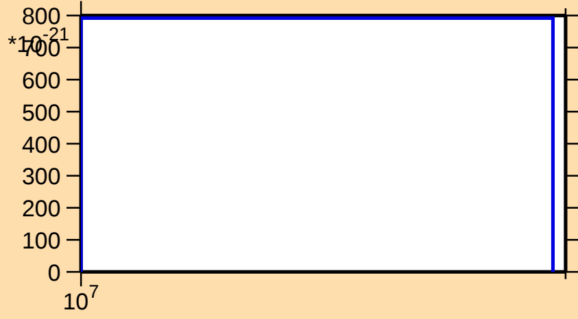
\sigma vs. E for ^{156}\text{Pm}(\text{mt } 11)
