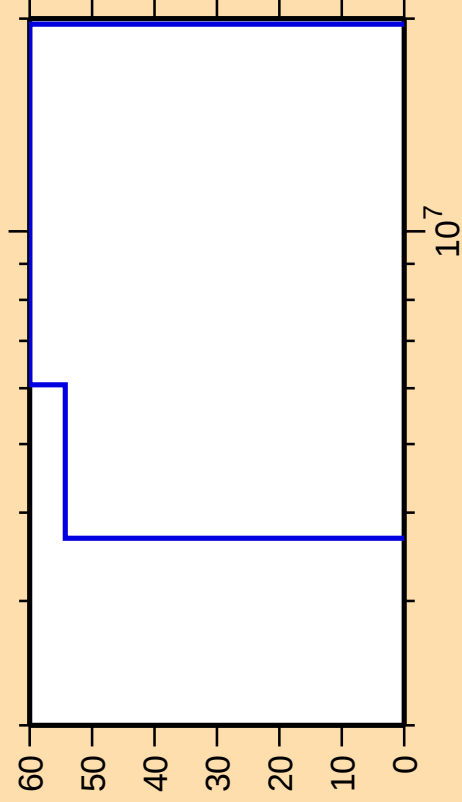
\Delta\sigma/\sigma vs. E for ^{156}\text{Pm}(n,n\text{cont.})
