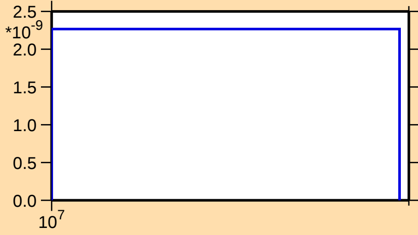
\sigma vs. E for ^{156}\text{Pm}(n,2np)
