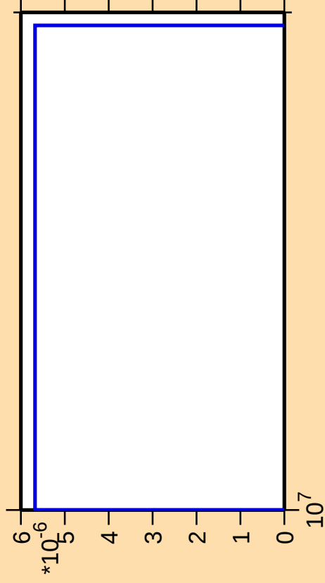
\Delta\sigma/\sigma vs. E for ^{156}\text{Pm}(\text{mt } 11)
