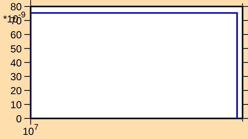
\sigma vs. E for ^{156}\text{Pm}(n,\text{nd})
