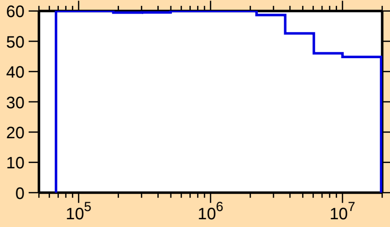
\Delta\sigma/\sigma vs. E for ^{156}\text{Pm}(n,\text{nonel.})
