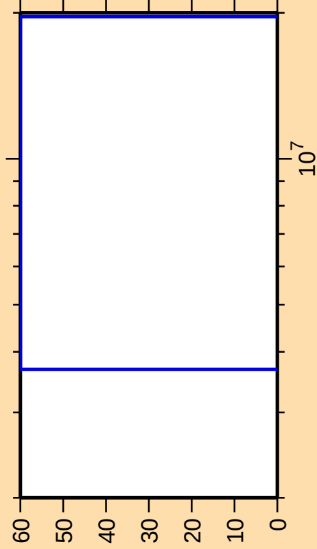
\Delta\sigma/\sigma vs. E for ^{156}\text{Pm}(n,n_1)
