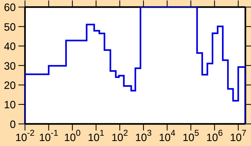
\Delta\sigma/\sigma vs. E for ^{156}\text{Pm}(n,\text{tot.})
