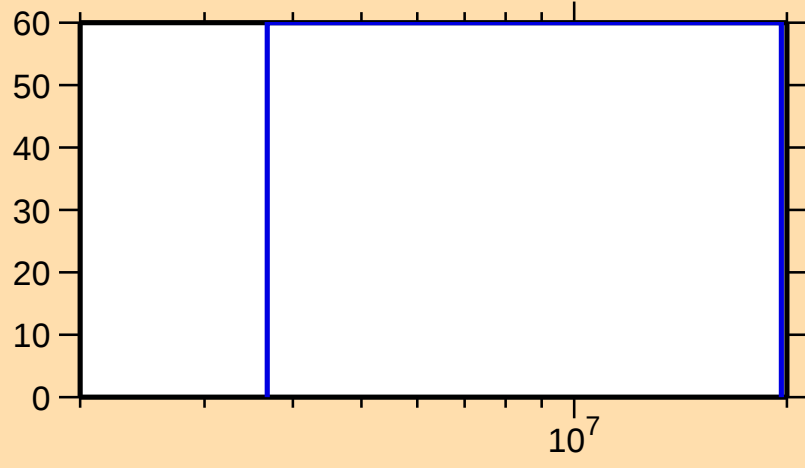
\Delta\sigma/\sigma vs. E for ^{156}\text{Pm}(n,2n)
