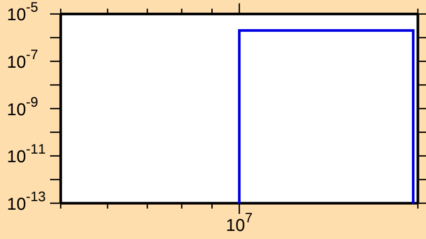
\sigma vs. E for ^{156}\text{Pm}(n,n\alpha)
