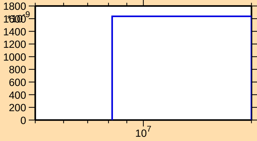
\sigma vs. E for ^{156}\text{Pm}(n,n\alpha)
