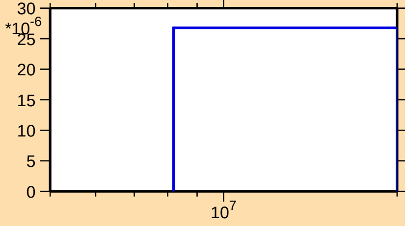
\sigma vs. E for ^{156}\text{Pm}(n,np)
