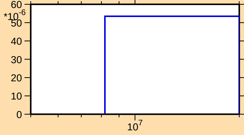
\sigma vs. E for ^{156}\text{Pm}(n,d)
