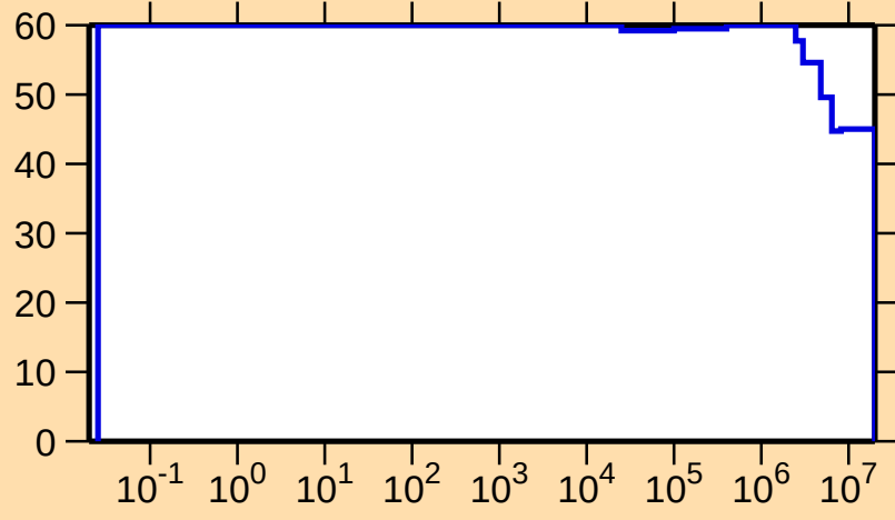
\Delta\sigma/\sigma vs. E for ^{156}\text{Pm}(n,\text{nonel.})
