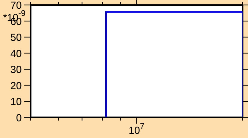
\sigma vs. E for ^{156}\text{Pm}(n,nd)
