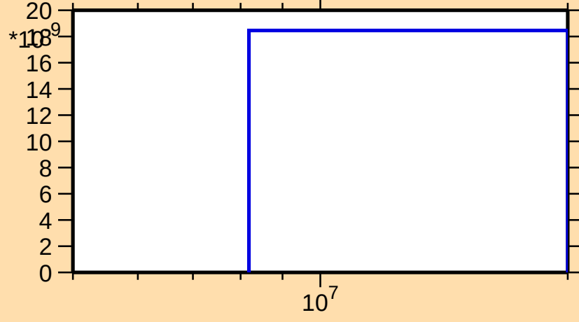
\sigma vs. E for ^{156}\text{Pm}(n,nt)
