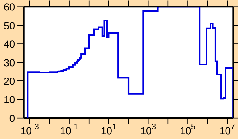
\Delta\sigma/\sigma vs. E for ^{156}\text{Pm}(n,\text{tot.})
