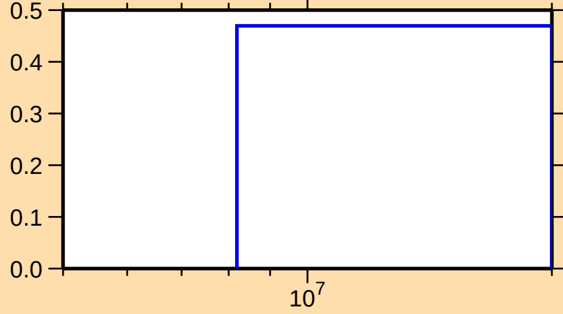
\sigma vs. E for ^{156}\text{Pm}(n,3n)
