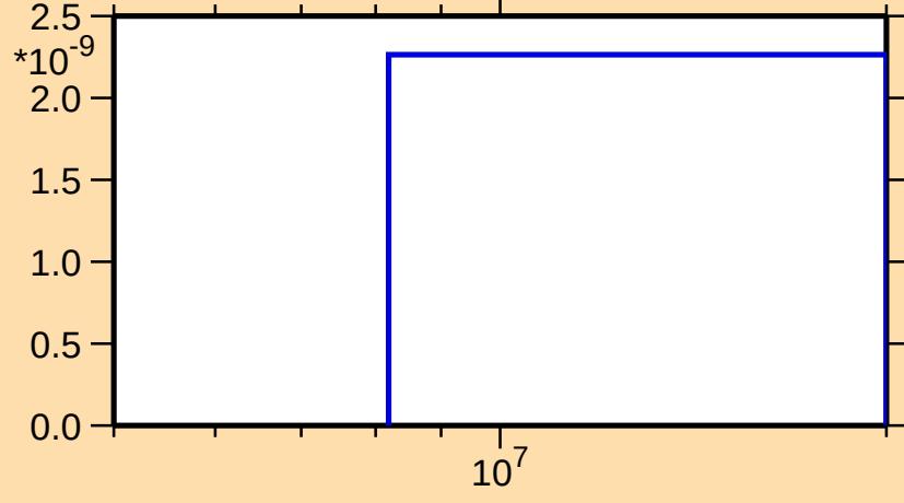
\sigma vs. E for ^{156}\text{Pm}(n,2np)
