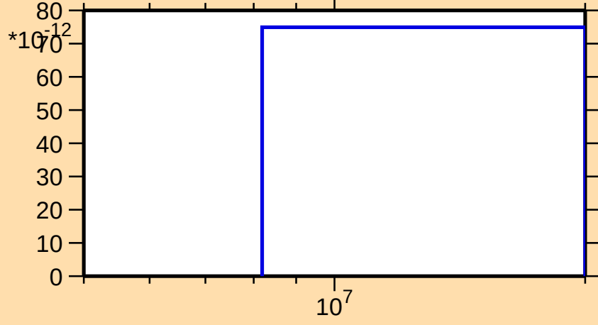
\sigma vs. E for ^{156}\text{Pm}(n,2n\alpha)
