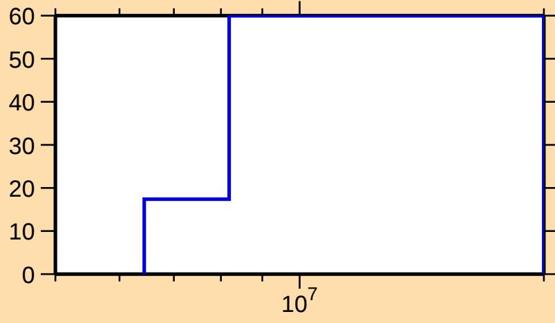
\Delta\sigma/\sigma vs. E for ^{160}\text{Pm}(n,2n)
