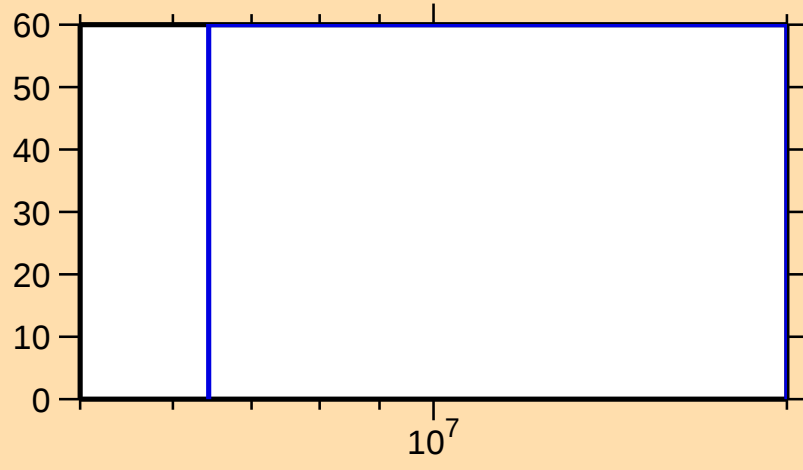
\Delta\sigma/\sigma vs. E for ^{160}\text{Pm}(n,ncont.)
