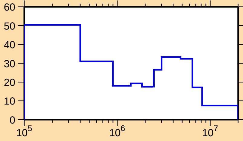
\Delta\sigma/\sigma vs. E for ^{160}\text{Pm}(n,\text{el.})
