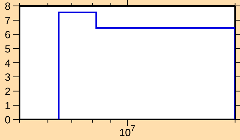
\Delta\sigma/\sigma vs. E for ^{160}\text{Pm}(n,\text{nonel.})
