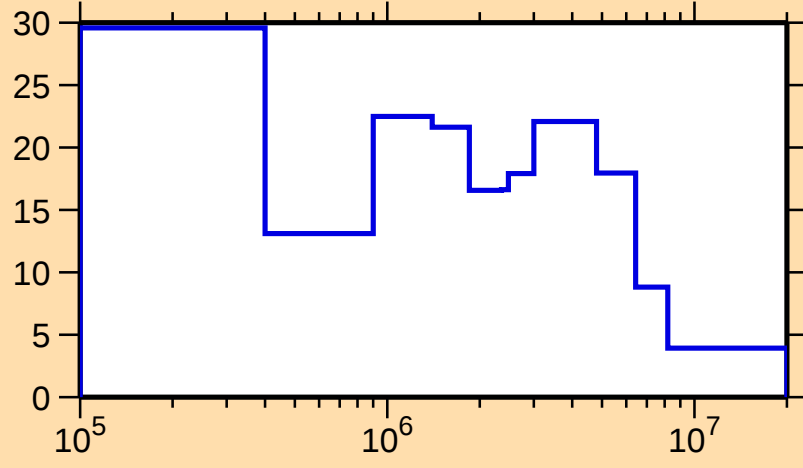
\Delta\sigma/\sigma vs. E for ^{160}\text{Pm}(n,\text{tot.})
