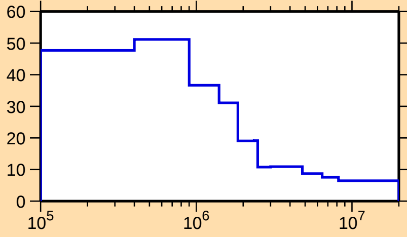
\Delta\sigma/\sigma vs. E for ^{160}\text{Pm}(n,\text{nonel.})
