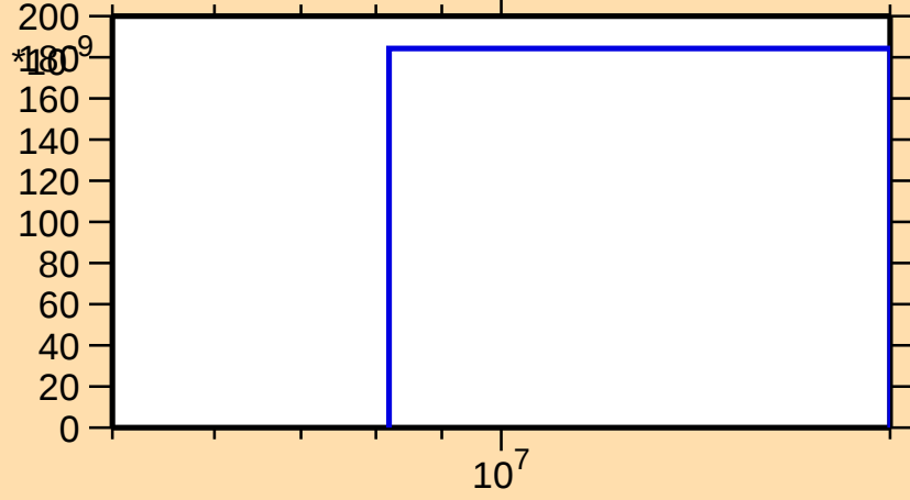
\sigma vs. E for ^{160}\text{Pm}(n,n\alpha)
