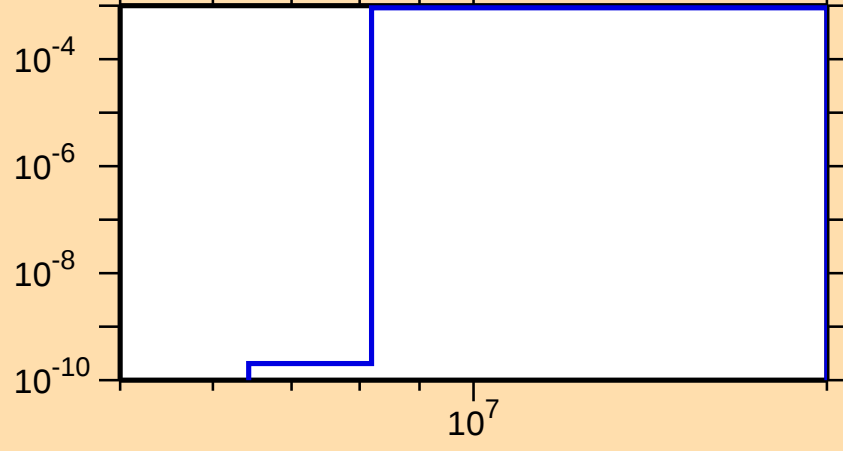
\sigma vs. E for ^{160}\text{Pm}(n,p)
