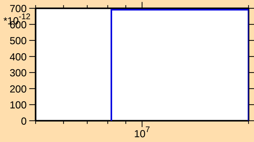
\sigma vs. E for ^{160}\text{Pm}(n,2np)
