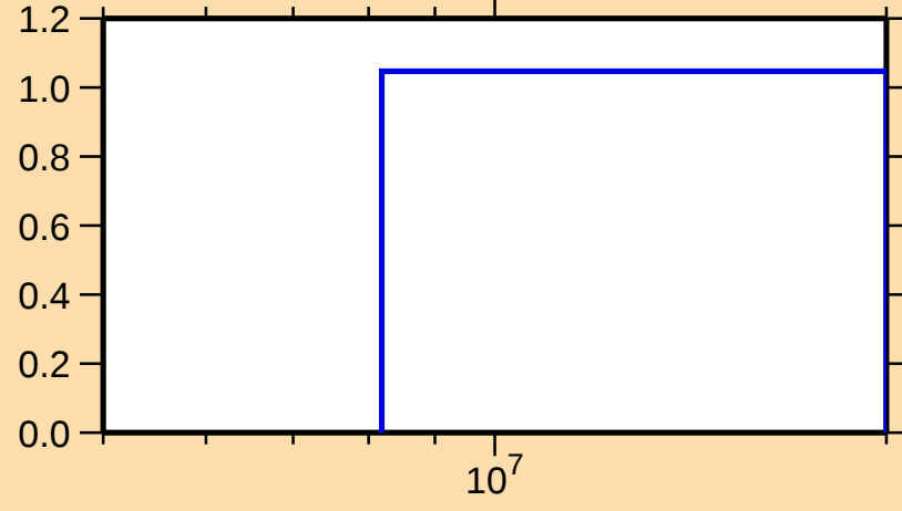
\sigma vs. E for ^{160}\text{Pm}(n,3n)
