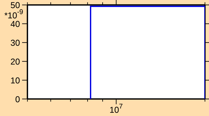
\sigma vs. E for ^{160}\text{Pm}(n,nt)
