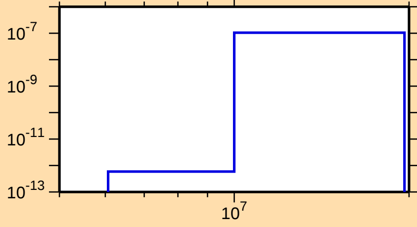
\sigma vs. E for ^{196}\text{Po}(\text{mt117})
