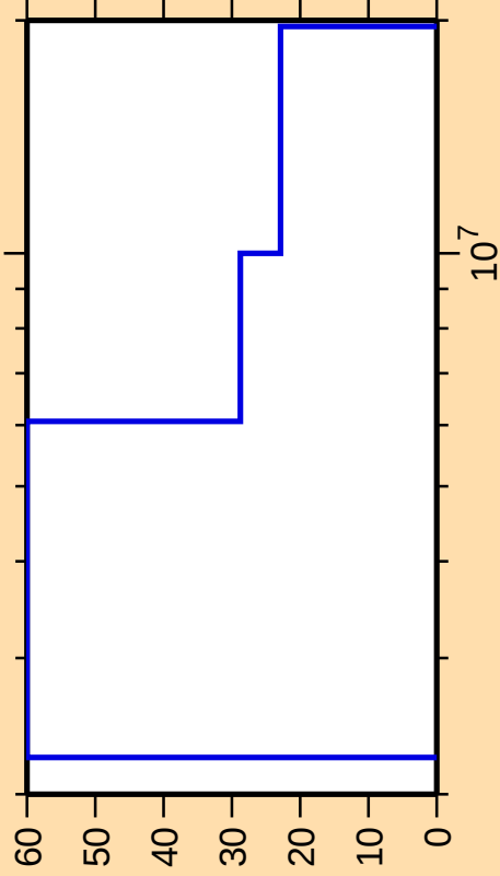
\Delta\sigma/\sigma vs. E for ^{196}\text{Po}(n,\text{ncont.})
