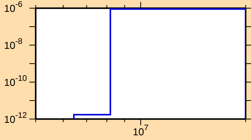
\sigma vs. E for ^{196}\text{Po}(n,\text{He}3)
