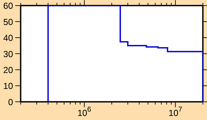
\Delta\sigma/\sigma vs. E for ^{196}\text{Po}(n,n_1)
