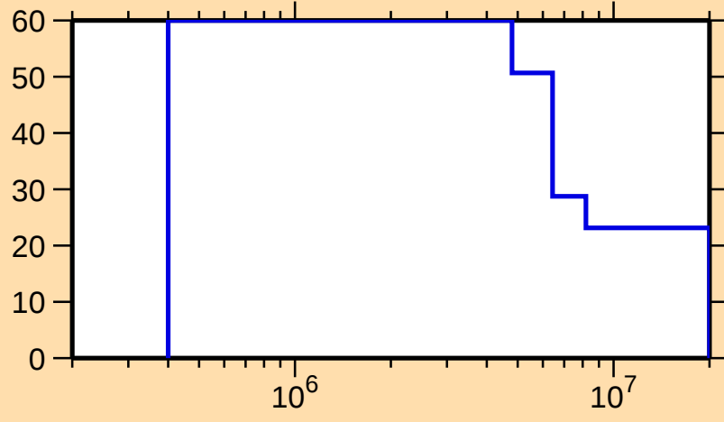
\Delta\sigma/\sigma vs. E for ^{196}\text{Po}(n,\text{inel.})
