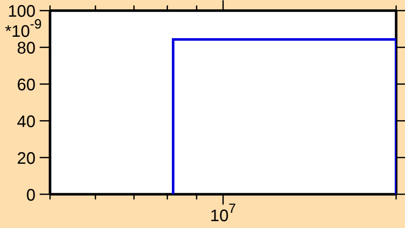
\sigma vs. E for ^{196}\text{Po}(\text{mt117})
