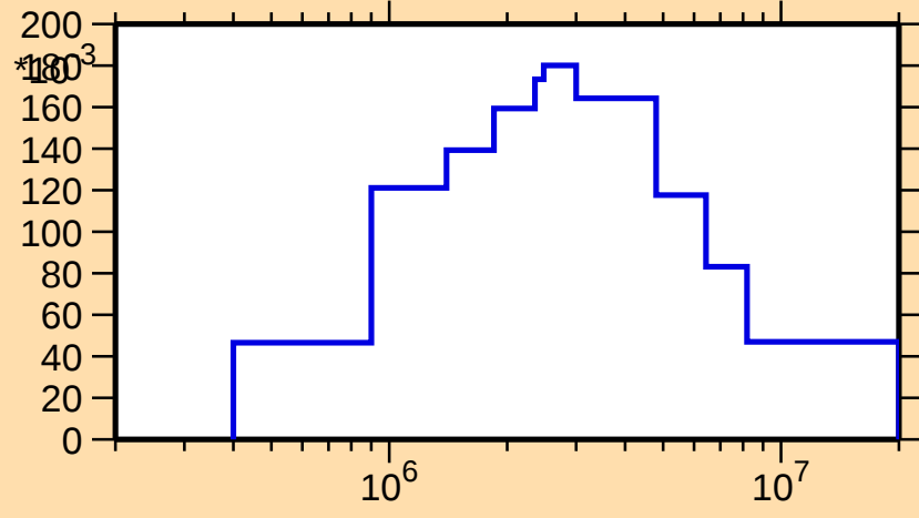
\sigma vs. E for ^{196}\text{Po}(n,n_1)
