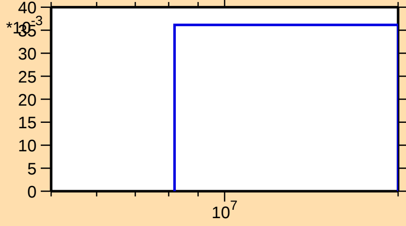
\sigma vs. E for ^{196}\text{Po}(n,2n)
