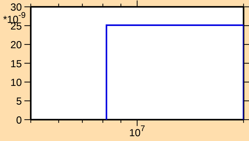
\sigma vs. E for ^{196}\text{Po}(n,3n)
