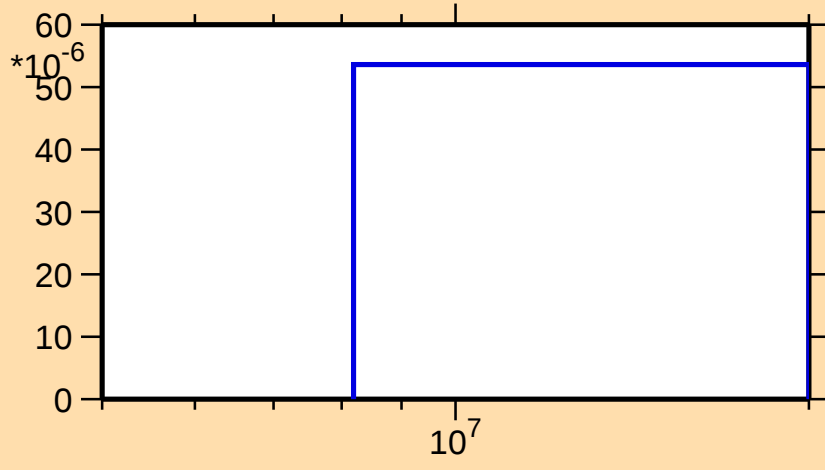
\sigma vs. E for ^{196}\text{Po}(n,t)
