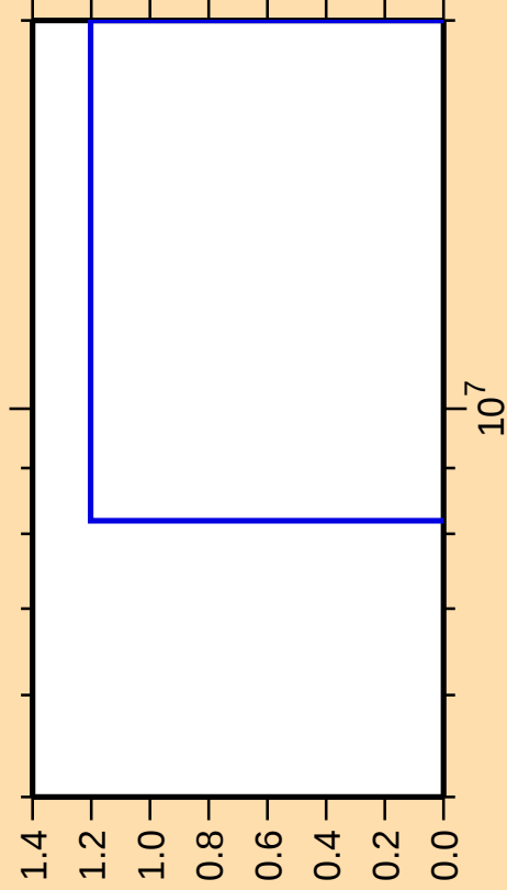
\Delta\sigma/\sigma vs. E for ^{196}\text{Po}(\text{mt } 34)
