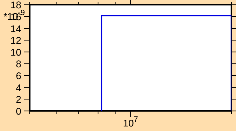
\sigma vs. E for ^{196}\text{Po}(n,\text{pd})
