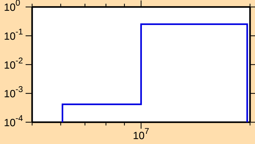
\sigma vs. E for ^{197}\text{Po}(n,2n)
