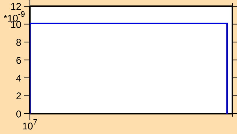
\sigma vs. E for ^{197}\text{Po}(n,\text{nd})
