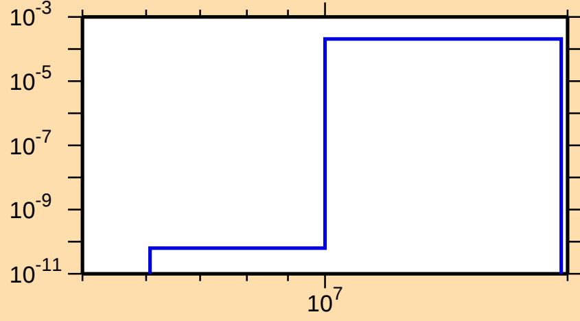
\sigma vs. E for ^{197}\text{Po}(n,t)
