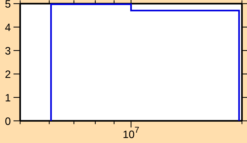
\Delta\sigma/\sigma vs. E for ^{197}\text{Po}(n,\text{nonel.})
