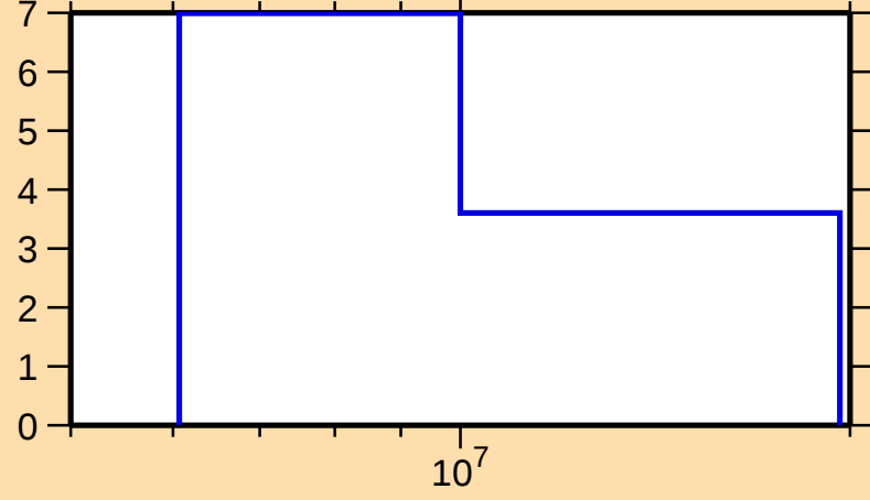
\Delta\sigma/\sigma vs. E for ^{197}\text{Po}(n,\text{tot.})
