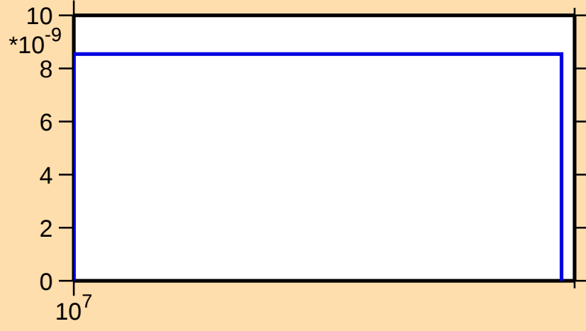
\sigma vs. E for ^{197}\text{Po}(n,3n)
