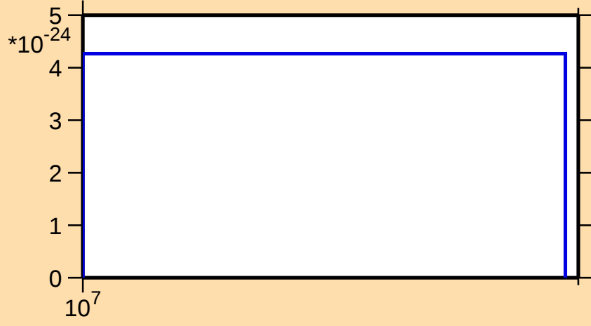
\sigma vs. E for ^{197}\text{Po}(\text{mt 11})
