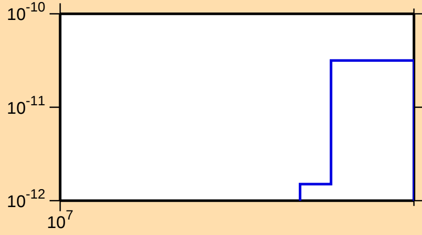
\sigma vs. E for ^{201}\text{Po}(\text{mt } 34)
