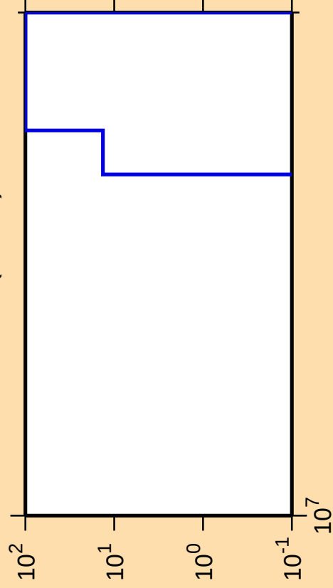
\Delta\sigma/\sigma vs. E for ^{201}\text{Po}(\text{mt } 34)
