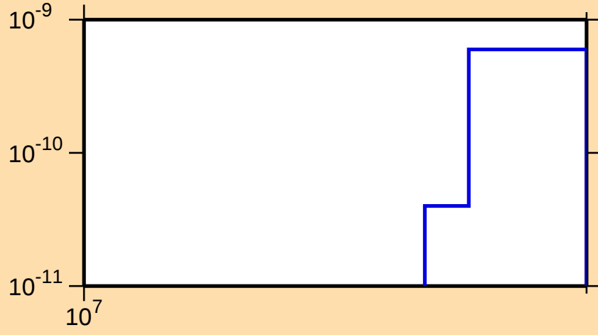
\sigma vs. E for ^{201}\text{Po}(n,\text{pt})
