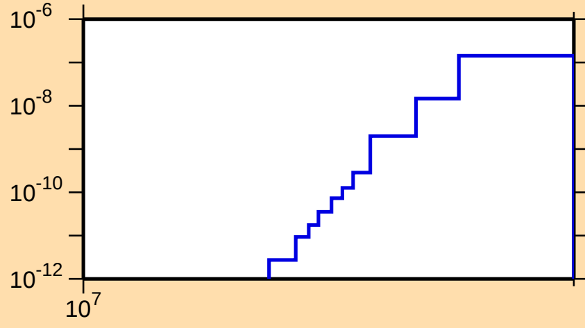
\sigma vs. E for ^{201}\text{Po}(n,\text{pd})
