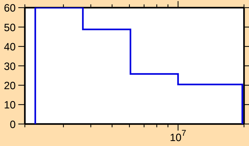
\Delta\sigma/\sigma vs. E for ^{201}\text{Po}(n,n\text{cont.})
