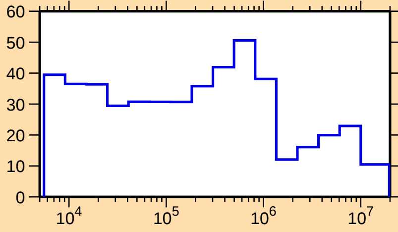
\Delta\sigma/\sigma vs. E for ^{201}\text{Po}(n,\text{tot.})
