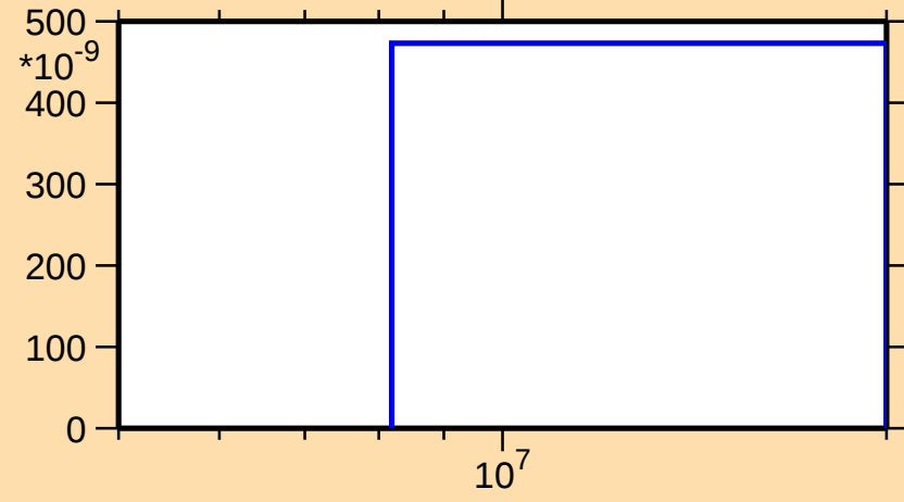
\sigma vs. E for ^{201}\text{Po}(n,3n)
