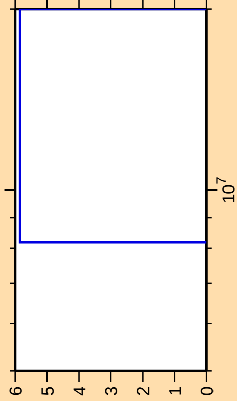
\Delta\sigma/\sigma vs. E for ^{201}\text{Po}(n,\text{pt})
