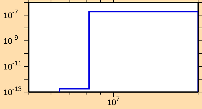
\sigma vs. E for ^{201}\text{Po}(n,\text{He3})
