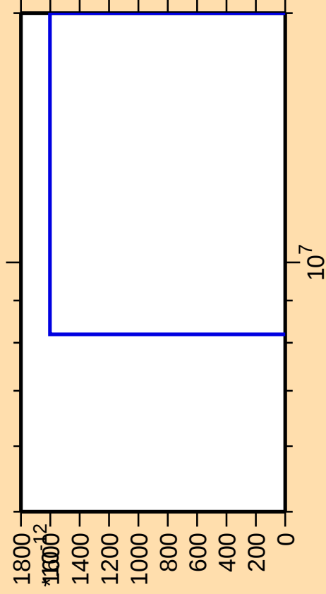
\Delta\sigma/\sigma vs. E for ^{201}\text{Po}(\text{mt } 11)
