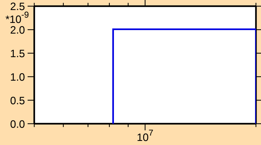
\sigma vs. E for ^{201}\text{Po}(n,\text{pd})
