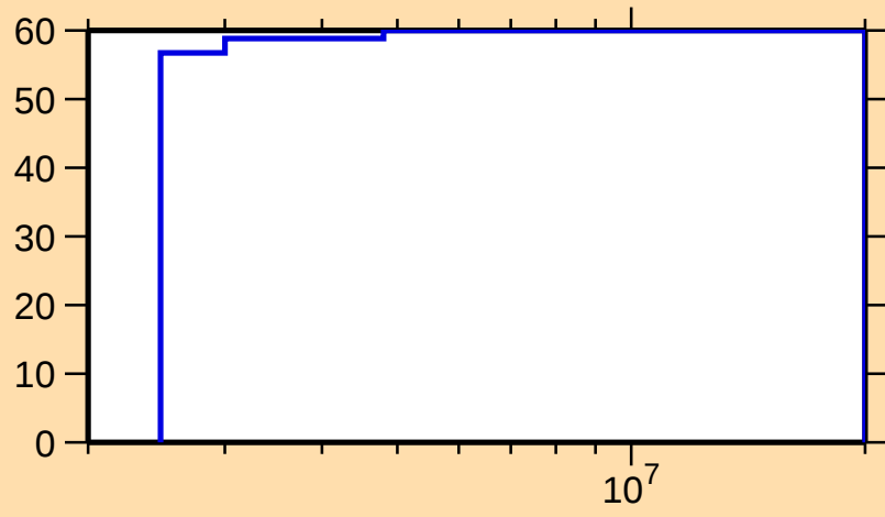
\Delta\sigma/\sigma vs. E for ^{201}\text{Po}(n,n_1)
