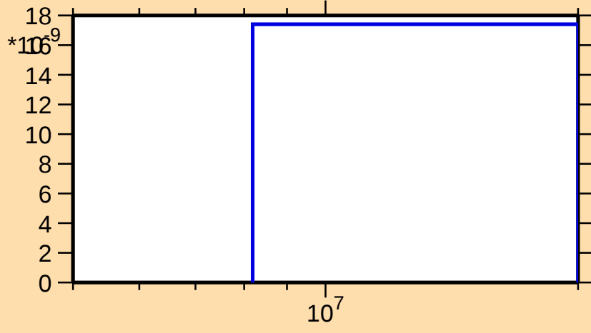
\sigma vs. E for ^{201}\text{Po}(n,\text{nd})
