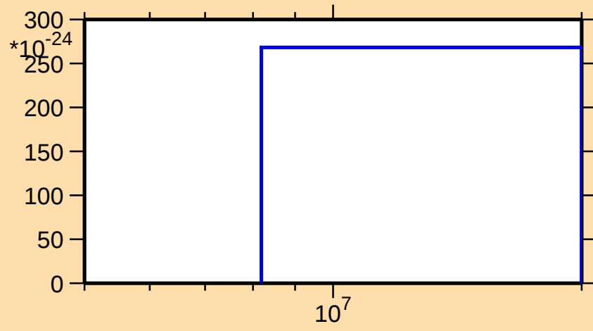
\sigma vs. E for ^{201}\text{Po}(\text{mt } 11)
