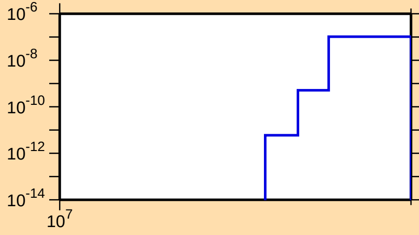
\sigma vs. E for ^{208}\text{Po}(n,nt)
