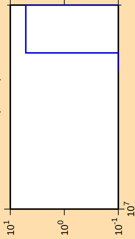
\Delta\sigma/\sigma vs. E for ^{208}\text{Po}(\text{mt } 34)
