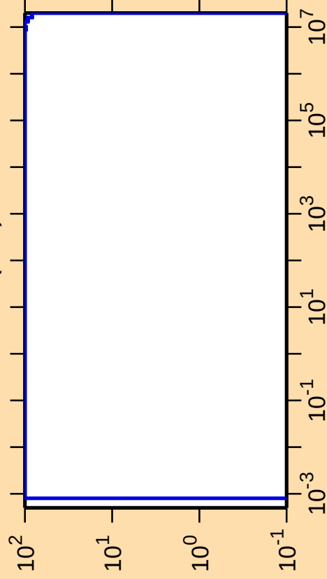
\Delta\sigma/\sigma vs. E for ^{208}\text{Po}(n,\alpha)
