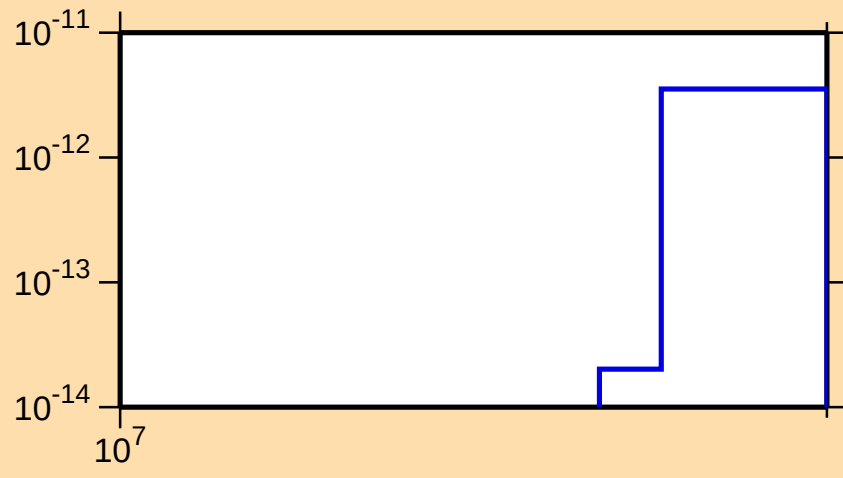
\sigma vs. E for ^{208}\text{Po}(n,\text{pt})
