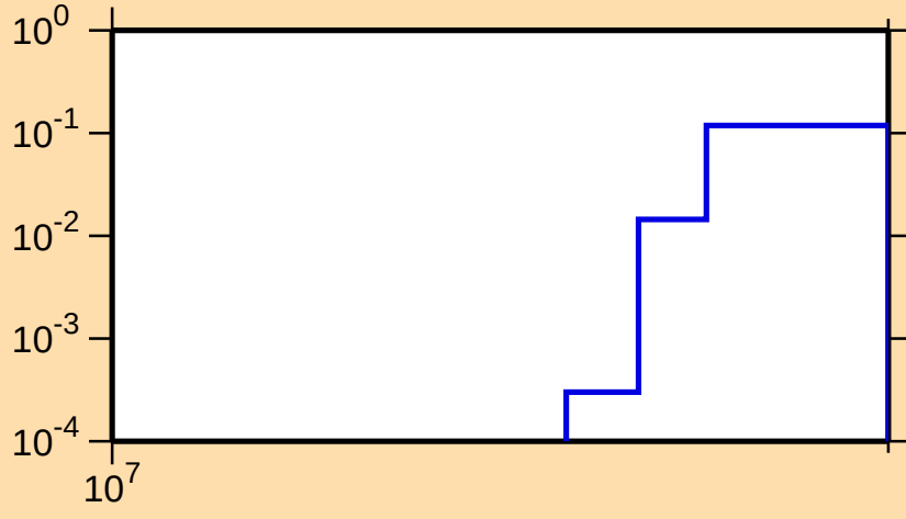
\sigma vs. E for ^{208}\text{Po}(n,3n)
