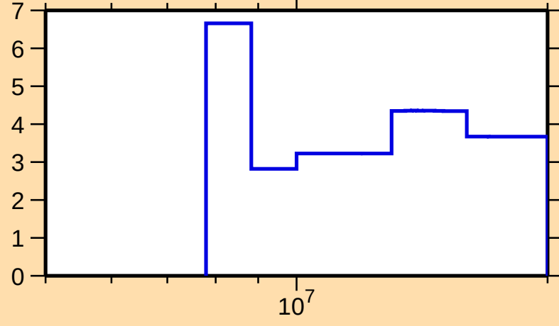
\Delta\sigma/\sigma vs. E for ^{208}\text{Po}(n,\text{tot.})
