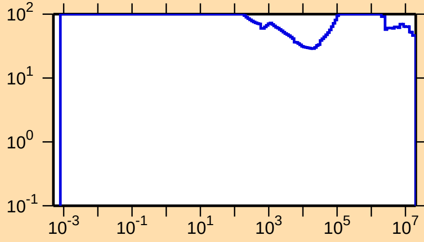
\Delta\sigma/\sigma vs. E for ^{208}\text{Po}(n,p)
