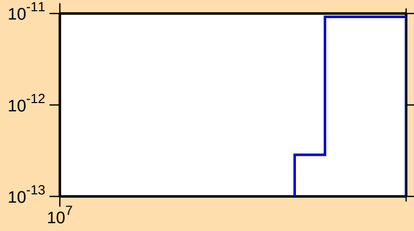
\sigma vs. E for ^{208}\text{Po}(n,3n\alpha)
