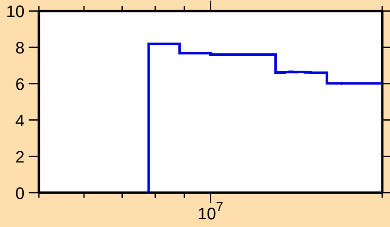
\Delta\sigma/\sigma vs. E for ^{208}\text{Po}(n,\text{nonel.})
