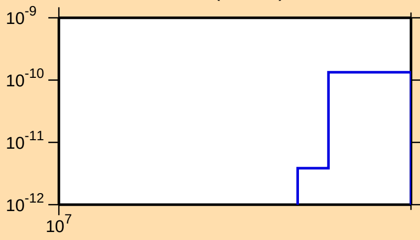
\sigma vs. E for ^{208}\text{Po}(\text{mt117})
