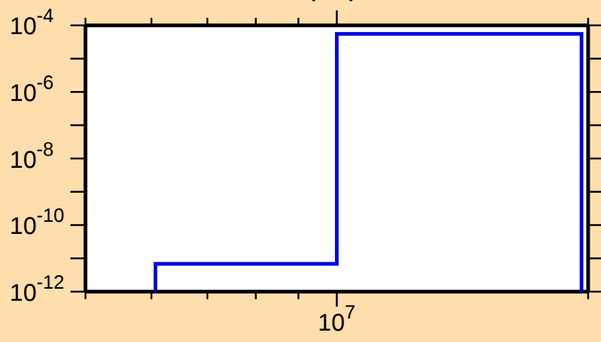
\sigma vs. E for ^{208}\text{Po}(n,t)
