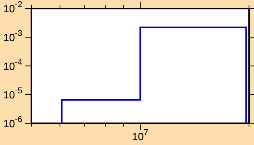
\sigma vs. E for ^{208}\text{Po}(n,np)
