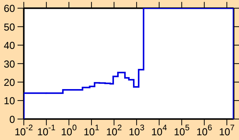
\Delta\sigma/\sigma vs. E for ^{208}\text{Po}(n,\gamma)
