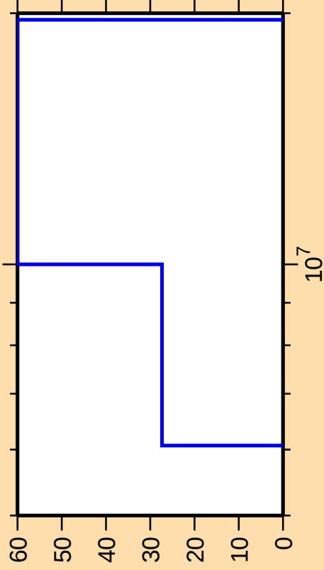
\Delta\sigma/\sigma vs. E for ^{208}\text{Po}(n,t)
