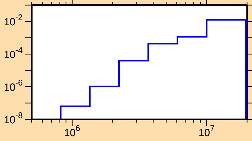
\sigma vs. E for ^{208}\text{Po}(n,p)
