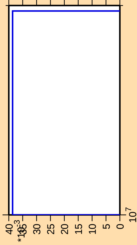
\Delta\sigma/\sigma vs. E for ^{208}\text{Po}(\text{mt } 34)
