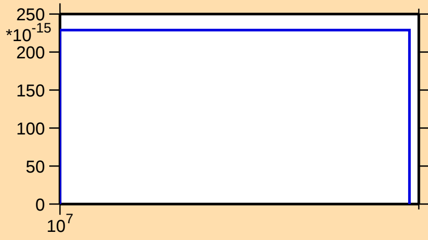
\sigma vs. E for ^{208}\text{Po}(n,3n\alpha)
