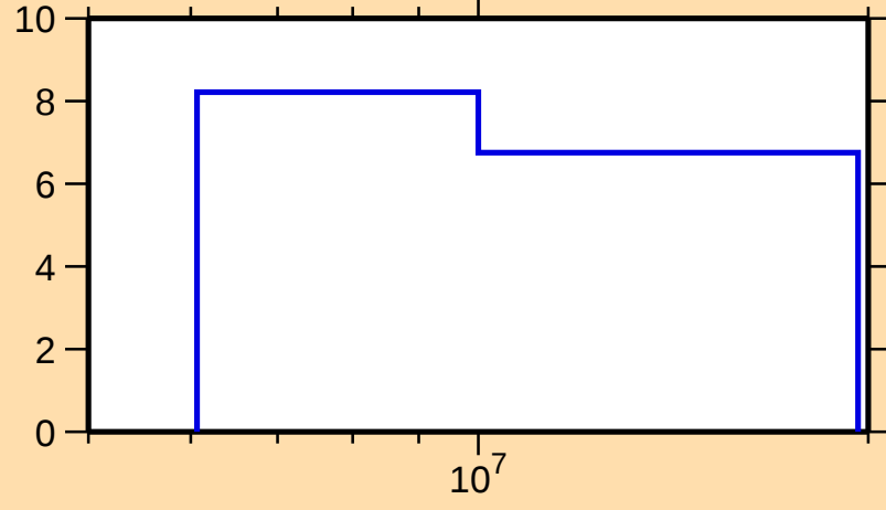
\Delta\sigma/\sigma vs. E for ^{208}\text{Po}(n,\text{nonel.})
