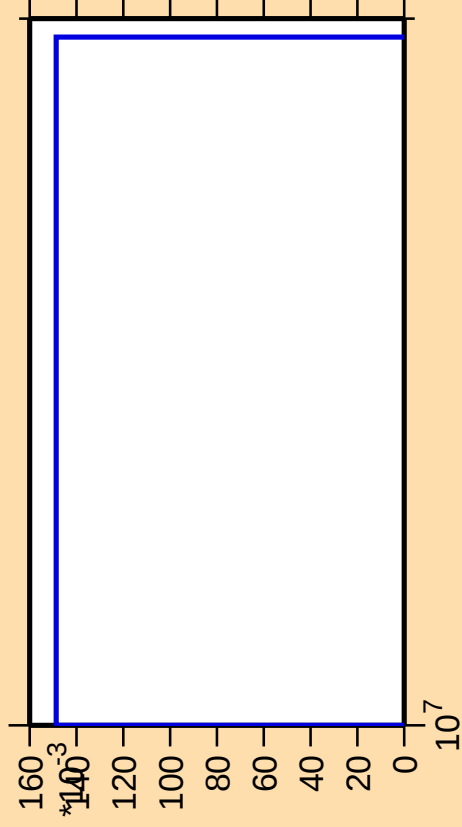
\Delta\sigma/\sigma vs. E for ^{208}\text{Po}(n,\text{pt})
