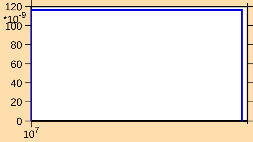
\sigma vs. E for ^{208}\text{Po}(n,2np)
