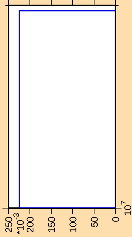
\Delta\sigma/\sigma vs. E for ^{208}\text{Po}(n,3n\alpha)
