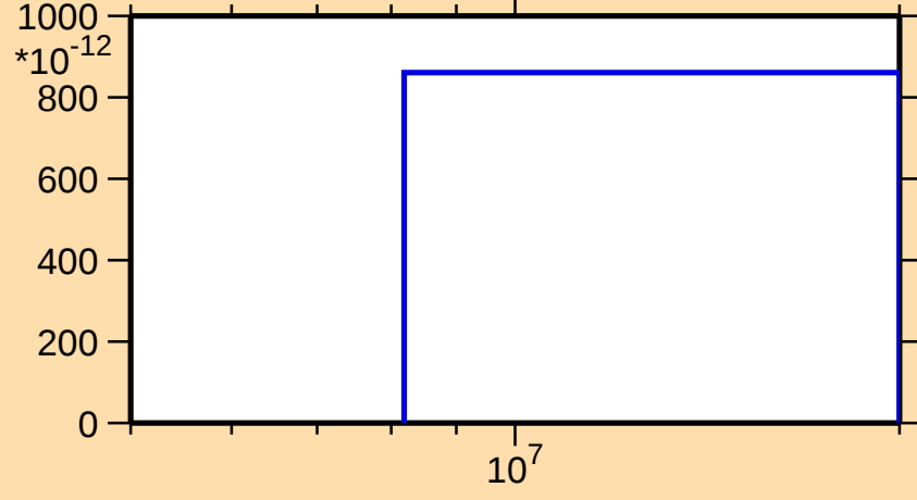
\sigma vs. E for ^{208}\text{Po}(n,nt)
