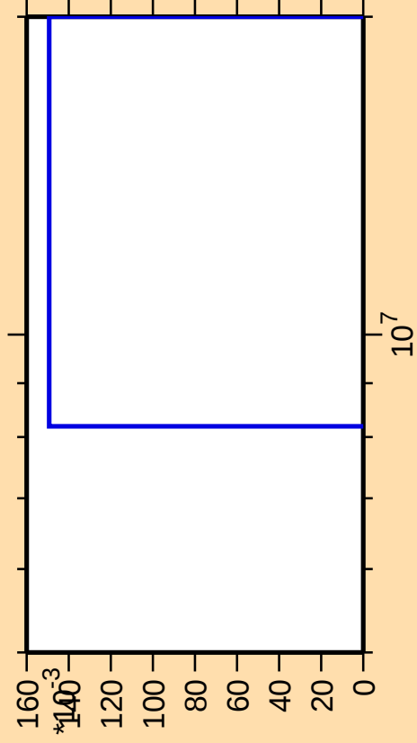
\Delta\sigma/\sigma vs. E for ^{208}\text{Po}(n,\text{pt})
