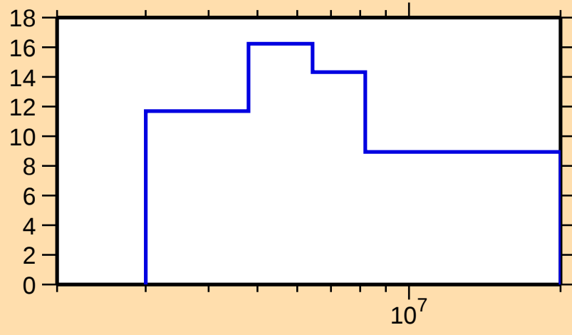
\Delta\sigma/\sigma vs. E for ^{208}\text{Po}(n,\text{el.})
