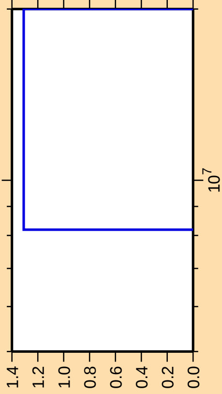
\Delta\sigma/\sigma vs. E for ^{208}\text{Po}(\text{mt117})
