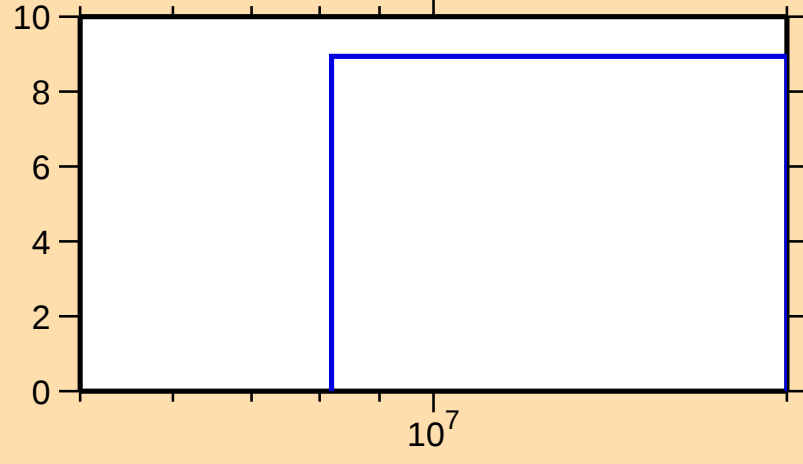
\Delta\sigma/\sigma vs. E for ^{208}\text{Po}(n,\text{el.})
