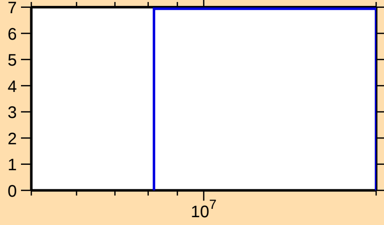
\Delta\sigma/\sigma vs. E for ^{208}\text{Po}(n,\text{nonel.})
