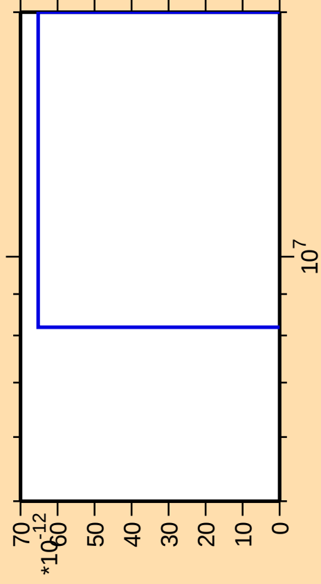
\Delta\sigma/\sigma vs. E for ^{208}\text{Po}(\text{mt } 42)
