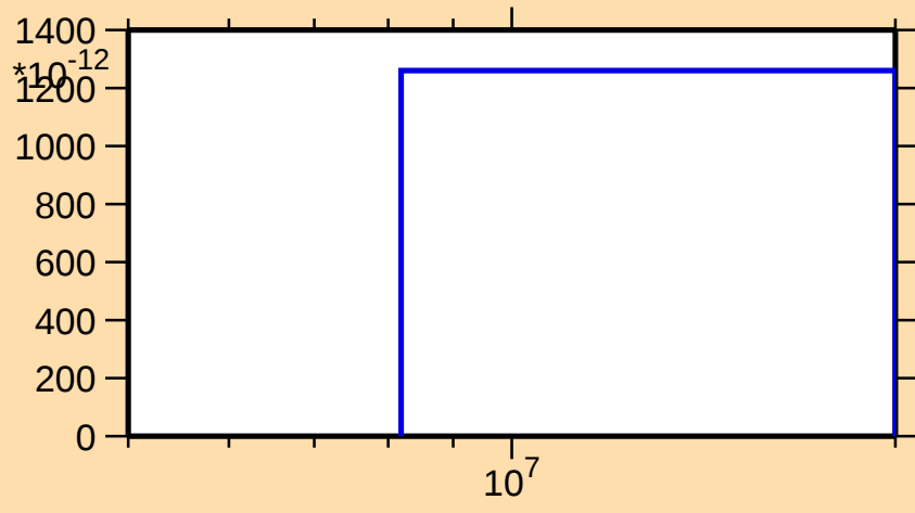
\sigma vs. E for ^{208}\text{Po}(n,\text{He}3)
