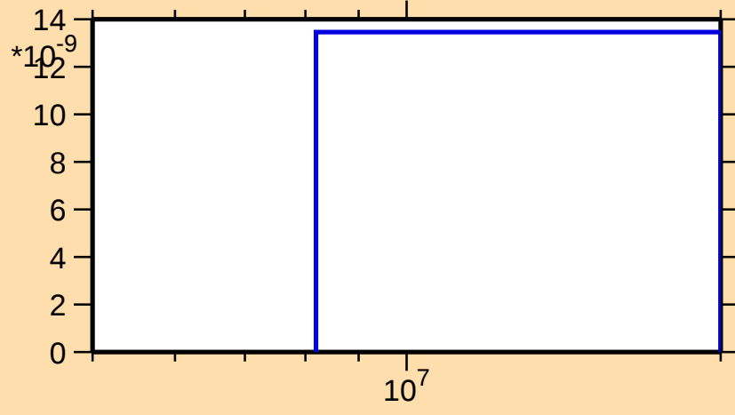
\sigma vs. E for ^{208}\text{Po}(n,\text{nd})
