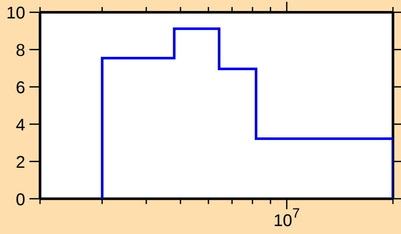
\Delta\sigma/\sigma vs. E for ^{208}\text{Po}(n,\text{tot.})
