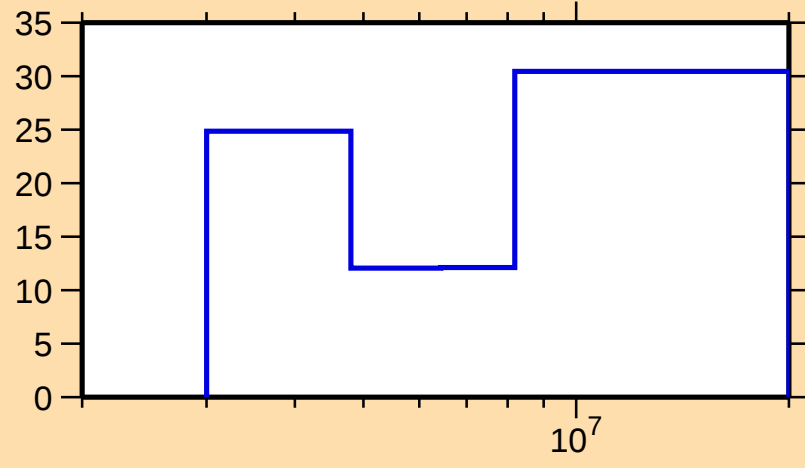
\Delta\sigma/\sigma vs. E for ^{208}\text{Po}(n,n\text{cont.})
