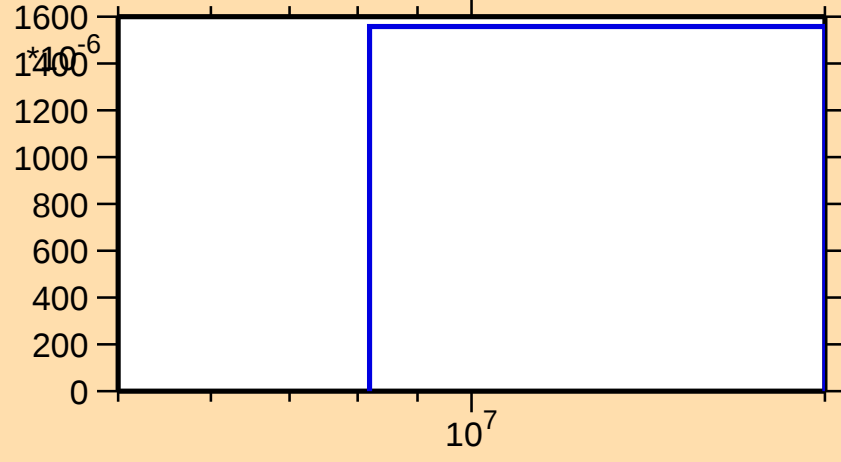
\sigma vs. E for ^{208}\text{Po}(n,3n)
