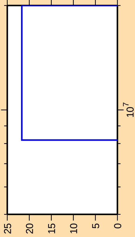
\Delta\sigma/\sigma vs. E for ^{208}\text{Po}(n,\text{pd})
