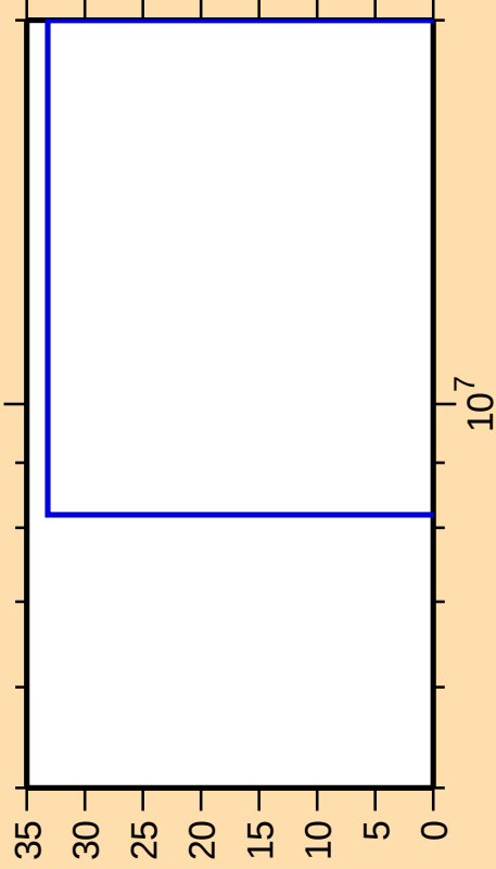
\Delta\sigma/\sigma vs. E for ^{208}\text{Po}(n,3n)
