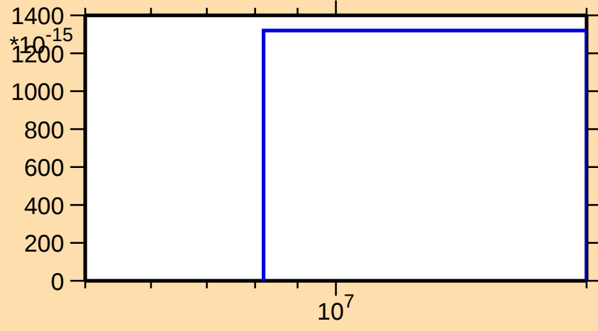
\sigma vs. E for ^{208}\text{Po}(\text{mt117})
