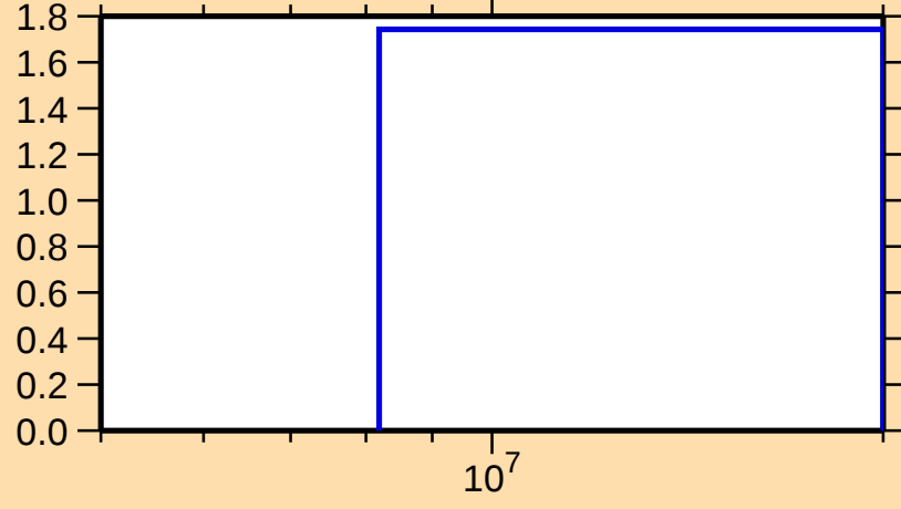
\sigma vs. E for ^{208}\text{Po}(n,2n)
