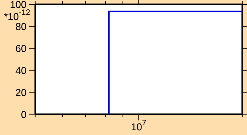
\sigma vs. E for ^{208}\text{Po}(n,p\alpha)
