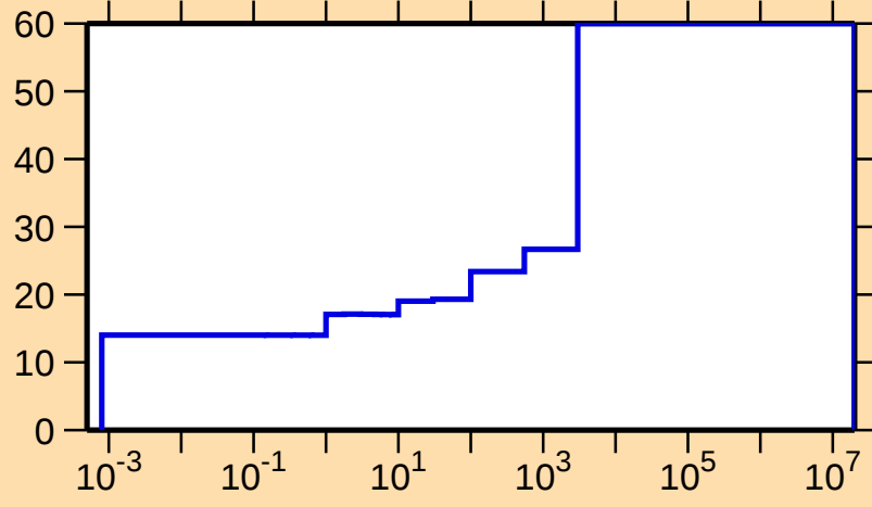
\Delta\sigma/\sigma vs. E for ^{208}\text{Po}(n,\gamma)
