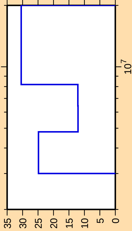
\Delta\sigma/\sigma vs. E for ^{208}\text{Po}(n,n_{\text{cont}})
