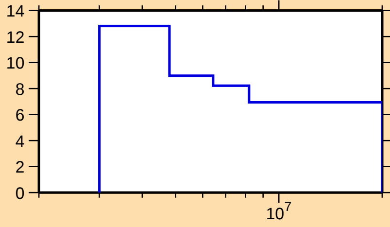
\Delta\sigma/\sigma vs. E for ^{208}\text{Po}(n,n\text{onel.})
