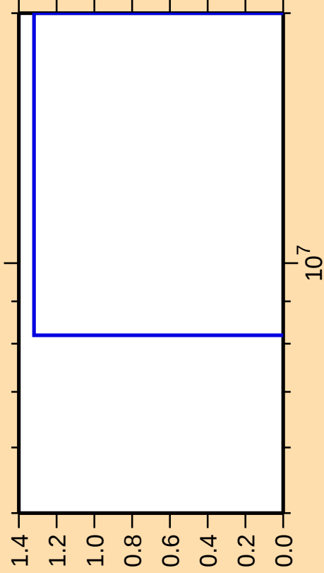
\Delta\sigma/\sigma vs. E for ^{208}\text{Po}(\text{mt } 45)
