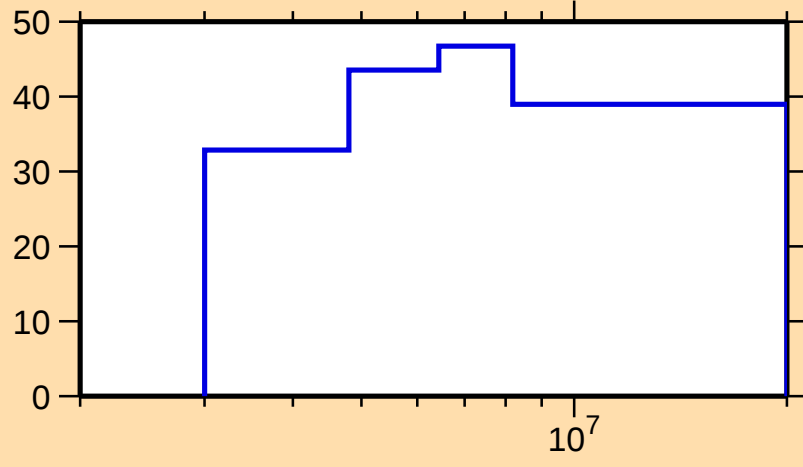
\Delta\sigma/\sigma vs. E for ^{208}\text{Po}(n,n_1)
