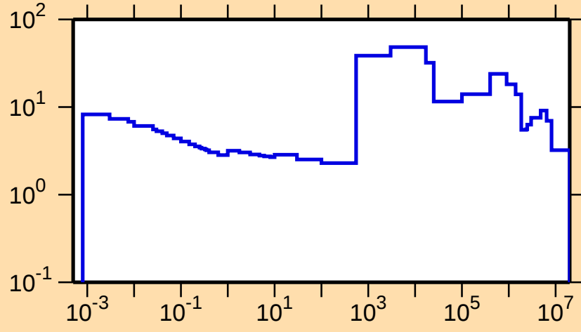
\Delta\sigma/\sigma vs. E for ^{208}\text{Po}(n,\text{tot.})
