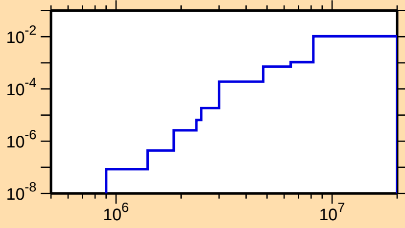
\sigma vs. E for ^{208}\text{Po}(n,p)
