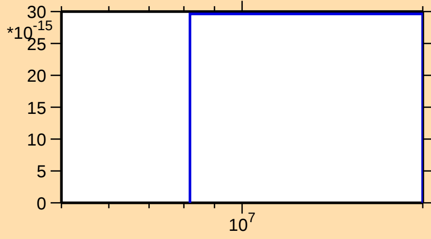
\sigma vs. E for ^{208}\text{Po}(n,\text{pt})
