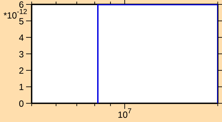
\sigma vs. E for ^{208}\text{Po}(n,\text{pd})
