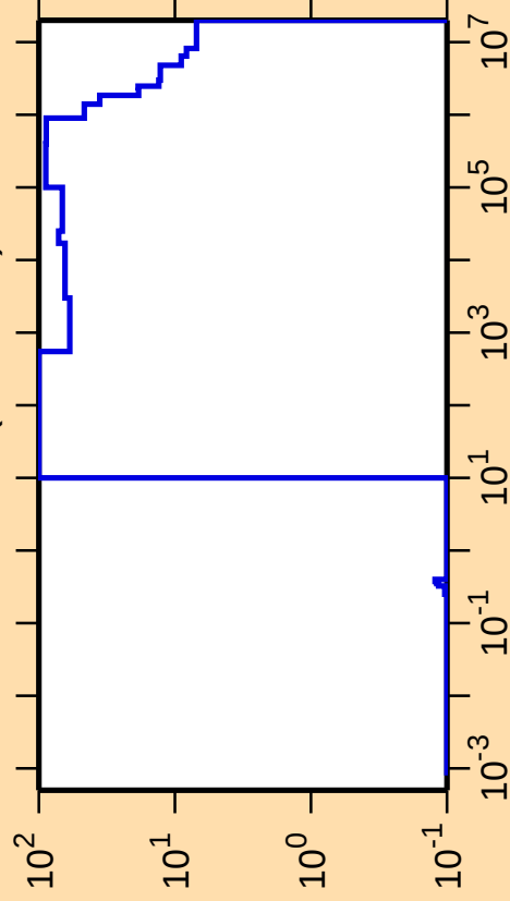
\Delta\sigma/\sigma vs. E for ^{208}\text{Po}(n,\text{nonel.})
