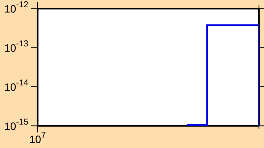
\sigma vs. E for ^{210}\text{Po}(\text{mt } 34)
