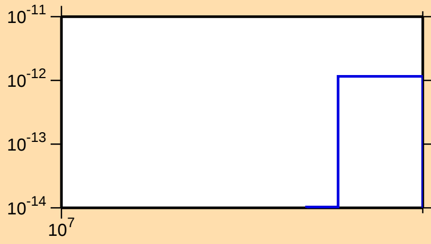
\sigma vs. E for ^{210}\text{Po}(n,\text{pt})
