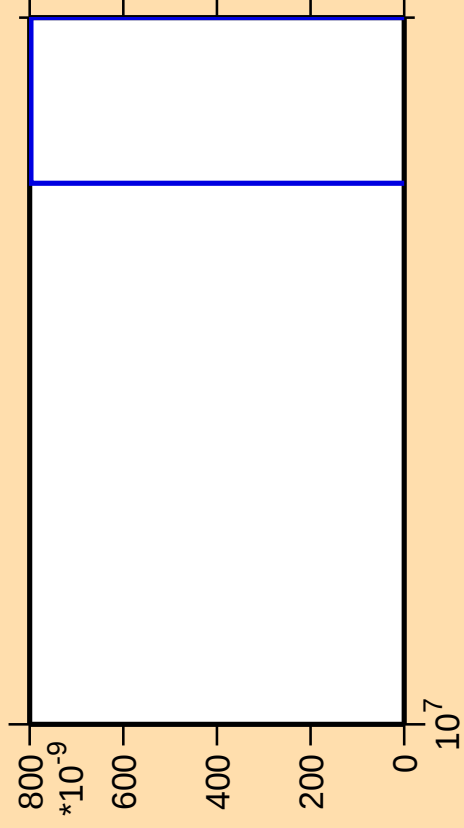
\Delta\sigma/\sigma vs. E for ^{210}\text{Po} (mt 42)
