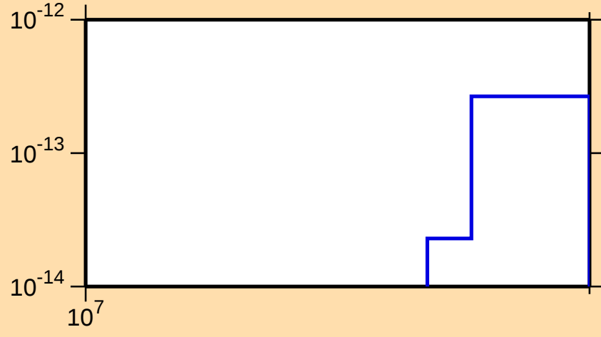
\sigma vs. E for ^{210}\text{Po}(\text{mt117})
