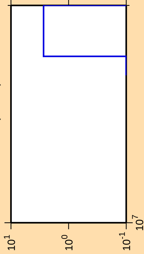
\Delta\sigma/\sigma vs. E for ^{210}\text{Po}(\text{mt } 34)
