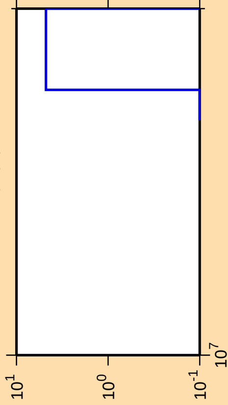
\Delta\sigma/\sigma vs. E for ^{210}\text{Po}(n,\text{pt})
