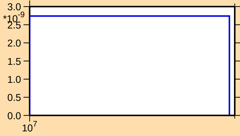
\sigma vs. E for ^{210}\text{Po}(n,\text{nt})
