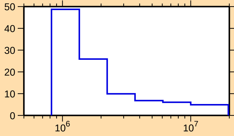
\Delta\sigma/\sigma vs. E for ^{210}\text{Po}(\text{n,nonel.})
