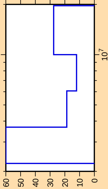
\Delta\sigma/\sigma vs. E for ^{210}\text{Po}(n,\text{ncont.})
