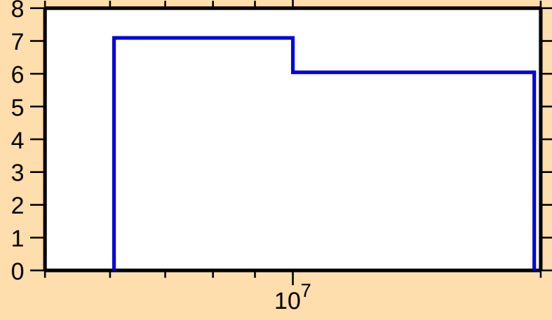
\Delta\sigma/\sigma vs. E for ^{210}\text{Po}(n,2n)
