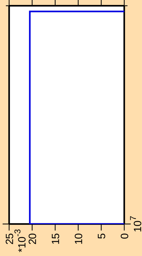
\Delta\sigma/\sigma vs. E for ^{210}\text{Po}(\text{mt117})
