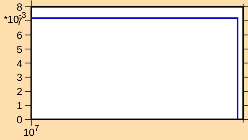
\sigma vs. E for ^{210}\text{Po}(n,3n)
