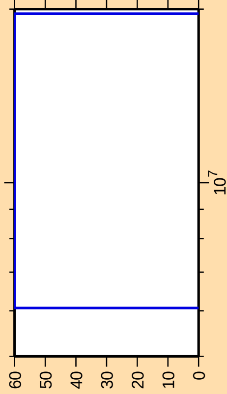
\Delta\sigma/\sigma vs. E for ^{210}\text{Po}(n,\text{np})
