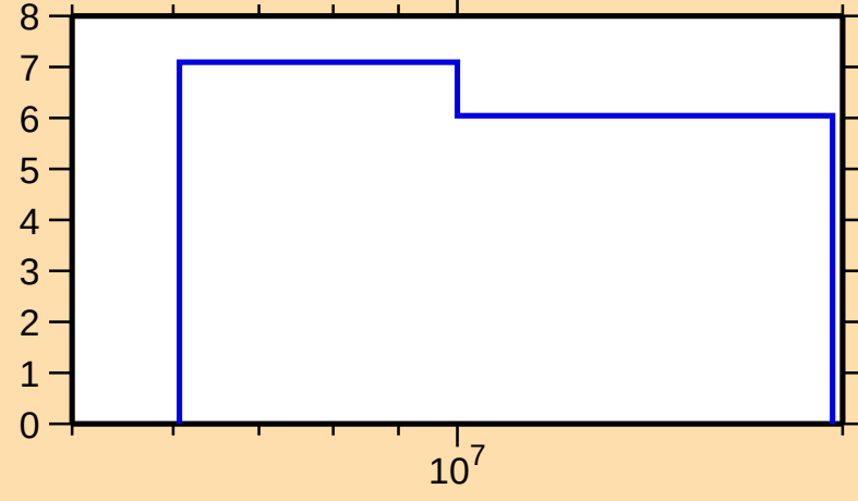
\Delta\sigma/\sigma vs. E for ^{210}\text{Po}(n,2n)
