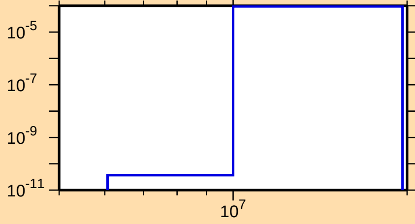
\sigma vs. E for ^{210}\text{Po}(n,t)
