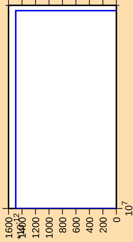
\Delta\sigma/\sigma vs. E for ^{210}\text{Po}(\text{mt } 42)
