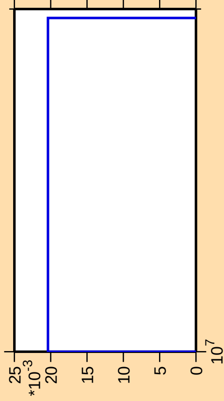
\Delta\sigma/\sigma vs. E for ^{210}\text{Po}(\text{mt } 34)
