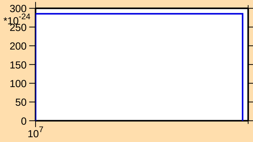
\sigma vs. E for ^{210}\text{Po}(\text{mt } 42)
