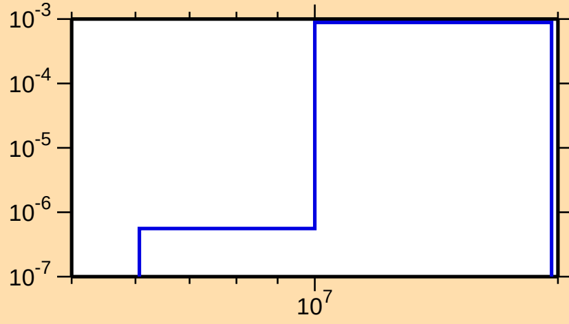
\sigma vs. E for ^{210}\text{Po}(n,\text{np})
