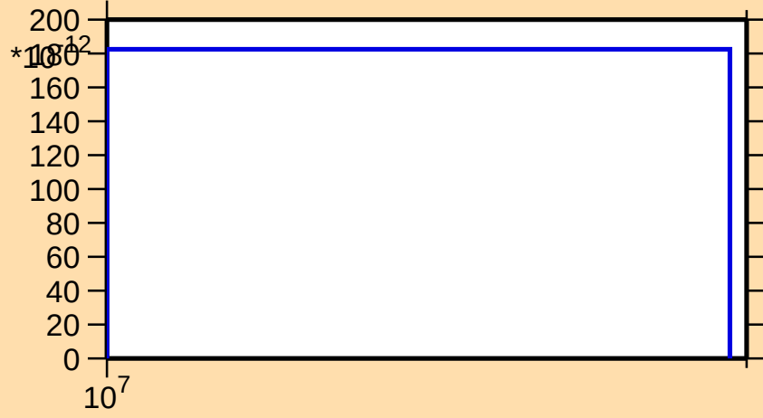
\sigma vs. E for ^{210}\text{Po}(n,\text{He3})
