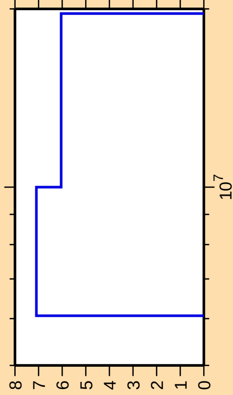
\Delta\sigma/\sigma vs. E for ^{210}\text{Po}(n,2n)
