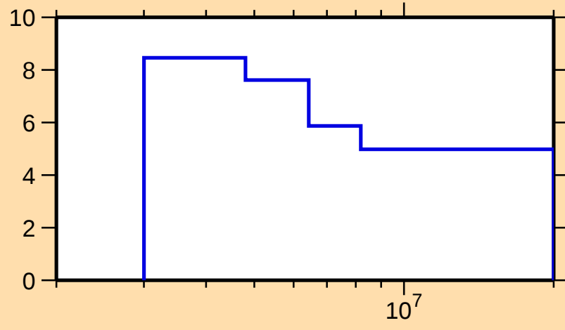
\Delta\sigma/\sigma vs. E for ^{210}\text{Po}(\text{n},\text{nonel.})
