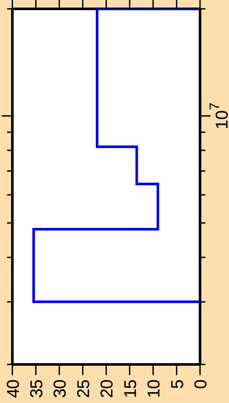
\Delta\sigma/\sigma vs. E for ^{210}\text{Po}(\text{n},\text{ncont.})
