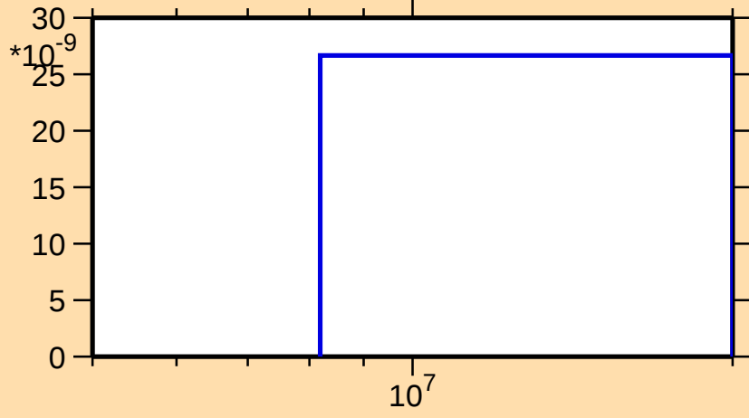
\sigma vs. E for ^{210}\text{Po}(n,\text{nd})
