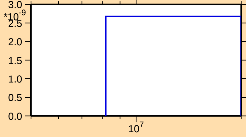
\sigma vs. E for ^{210}\text{Po}(n,\text{nt})
