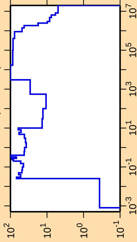
\Delta\sigma/\sigma vs. E for ^{210}\text{Po}(n,\text{nonel.})
