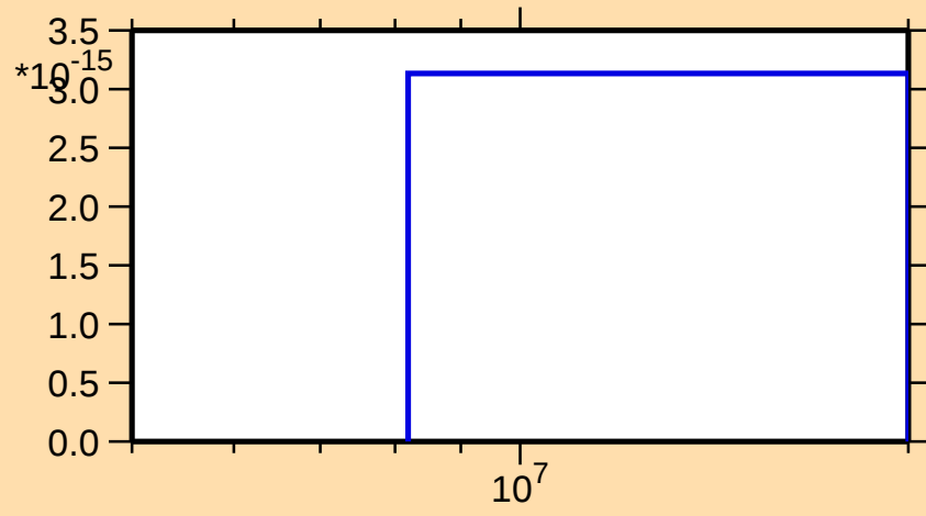
\sigma vs. E for ^{210}\text{Po}(\text{mt } 34)
