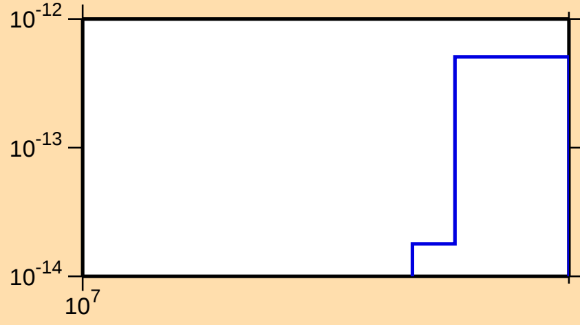
\sigma vs. E for ^{211}\text{Po}(n,\text{pd})
