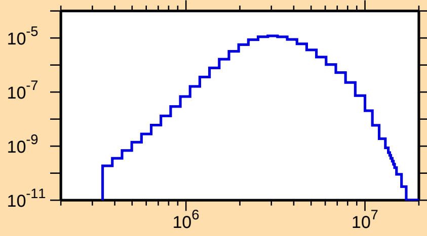
\sigma vs. E for ^{211}\text{Po}(n,n_3)
