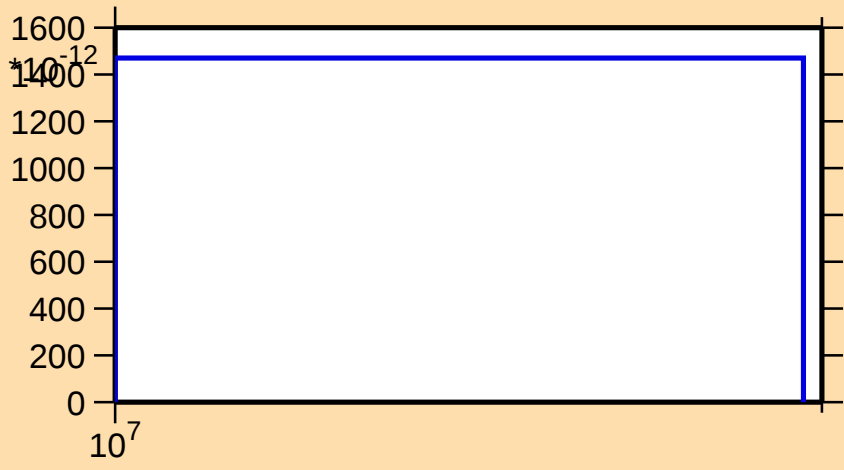
\sigma vs. E for ^{211}\text{Po}(\text{mt } 45)
