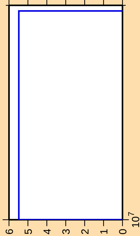
\Delta\sigma/\sigma vs. E for ^{211}\text{Po}(\text{mt } 11)
