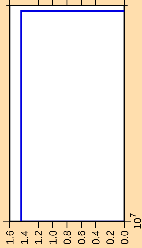
\Delta\sigma/\sigma vs. E for ^{211}\text{Po}(\text{mt } 42)
