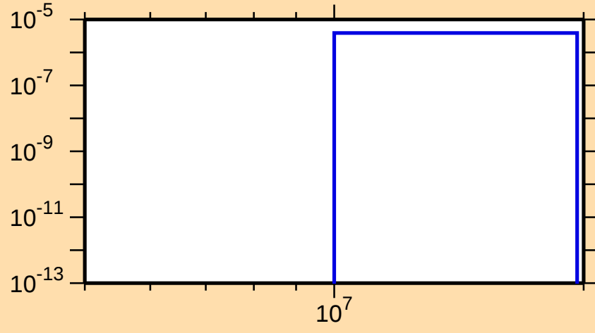
\sigma vs. E for ^{211}\text{Po}(n,nt)
