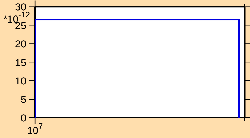
\sigma vs. E for ^{211}\text{Po}(\text{mt } 34)
