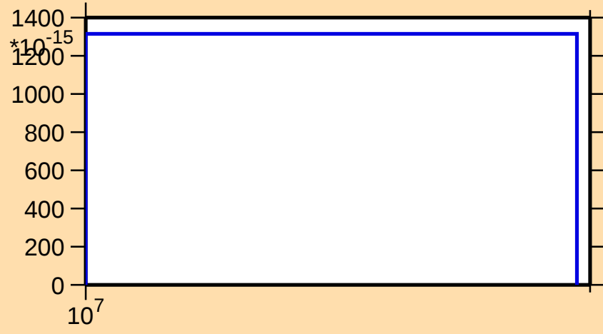
\sigma vs. E for ^{211}\text{Po}(\text{mt } 11)
