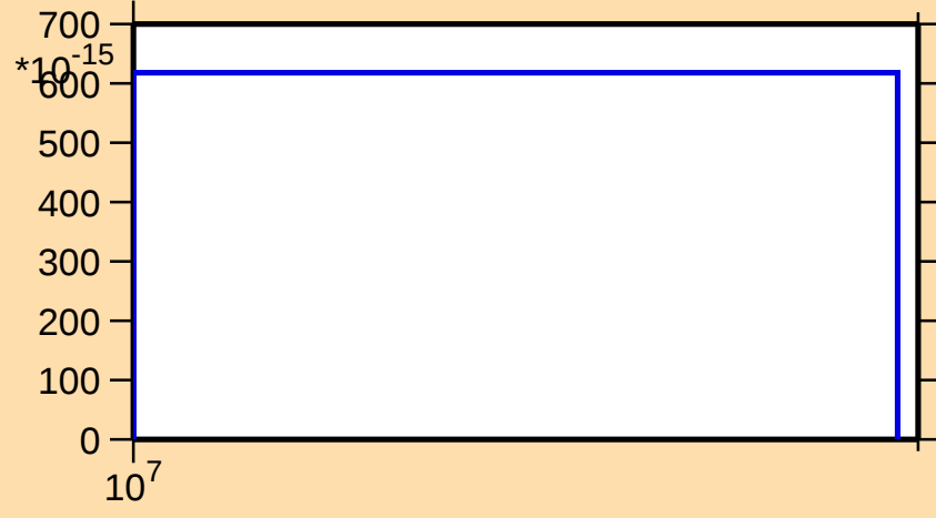
\sigma vs. E for ^{211}\text{Po}(\text{mt } 42)
