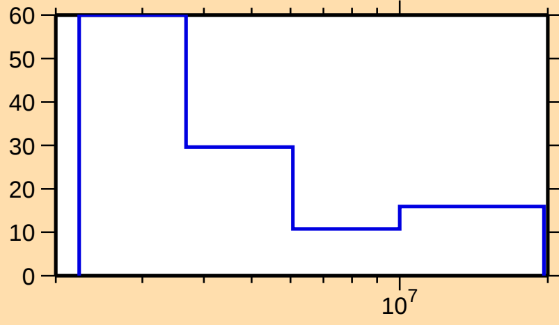
\Delta\sigma/\sigma vs. E for ^{211}\text{Po}(n,2n)
