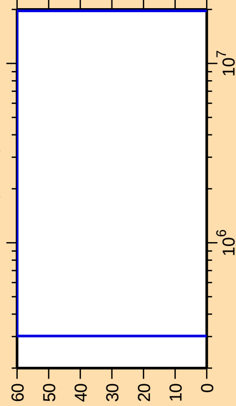
\Delta\sigma/\sigma vs. E for ^{211}\text{Po}(n,n\alpha)
