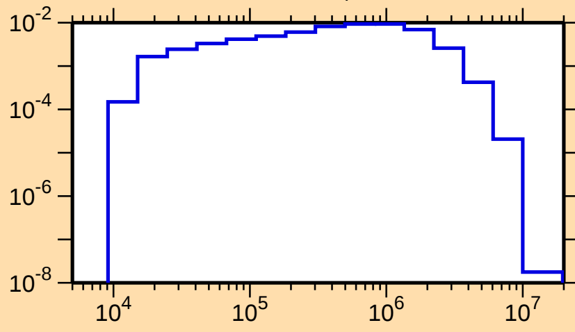
\sigma vs. E for ^{211}\text{Po}(n,n_4)
