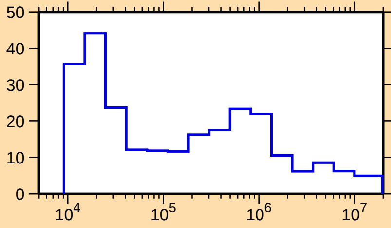
\Delta\sigma/\sigma vs. E for ^{211}\text{Po}(n,\text{tot.})
