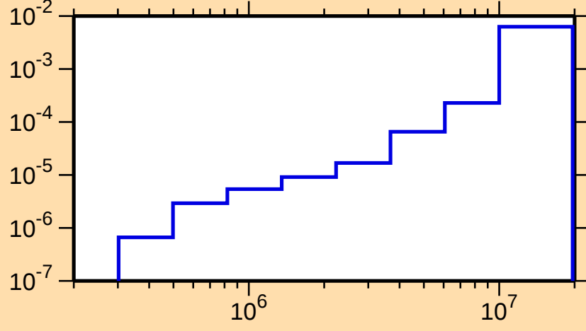
\sigma vs. E for ^{211}\text{Po}(n,n\alpha)
