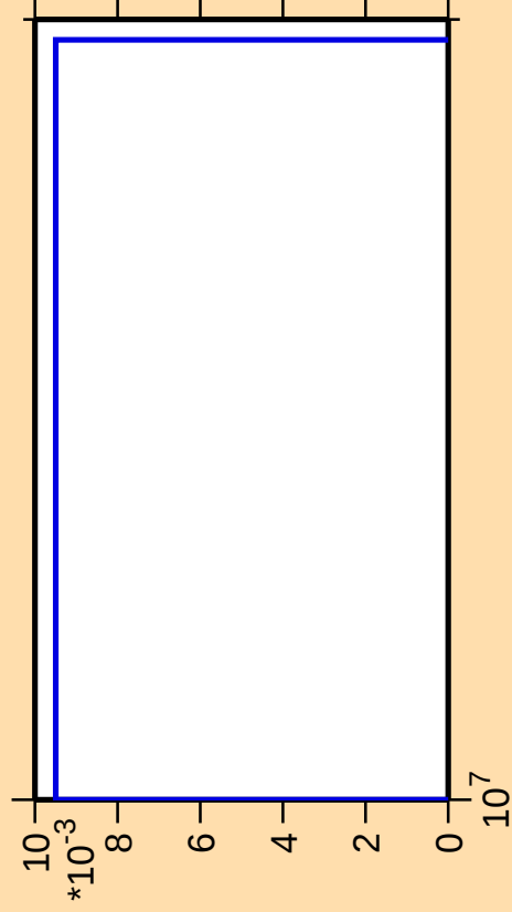
\Delta\sigma/\sigma vs. E for ^{211}\text{Po}(n,\text{pd})
