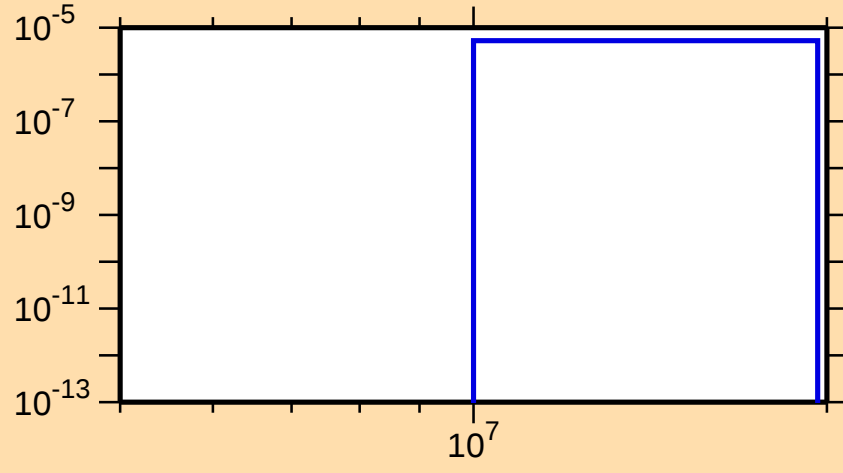
\sigma vs. E for ^{211}\text{Po}(n,2np)
