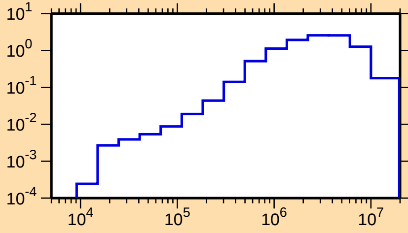
\sigma vs. E for ^{211}\text{Po}(n,\text{inel.})
