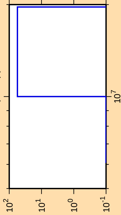
\Delta\sigma/\sigma vs. E for ^{211}\text{Po}(n,2np)
