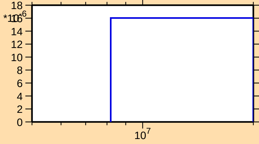
\sigma vs. E for ^{211}\text{Po}(n,\text{nd})
