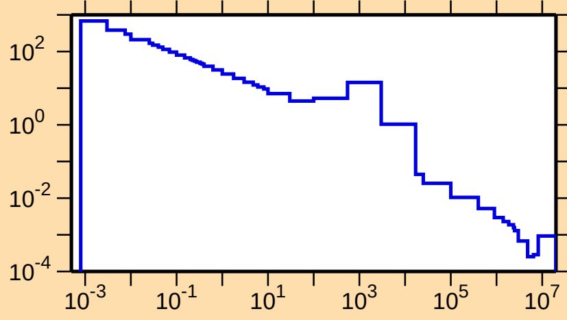
\sigma vs. E for ^{211}\text{Po}(n,\gamma)
