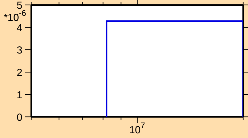
\sigma vs. E for ^{211}\text{Po}(n,2np)
