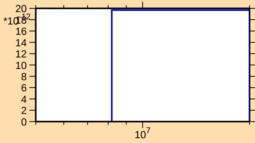
\sigma vs. E for ^{211}\text{Po}(n,\text{pt})
