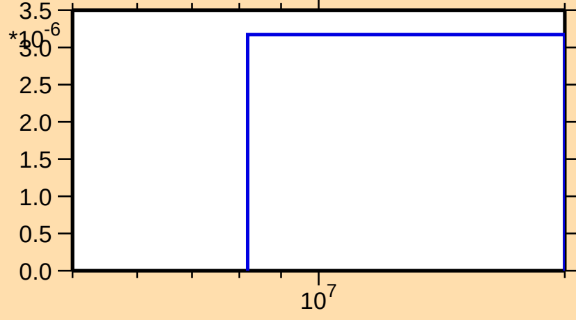
\sigma vs. E for ^{211}\text{Po}(n,nt)
