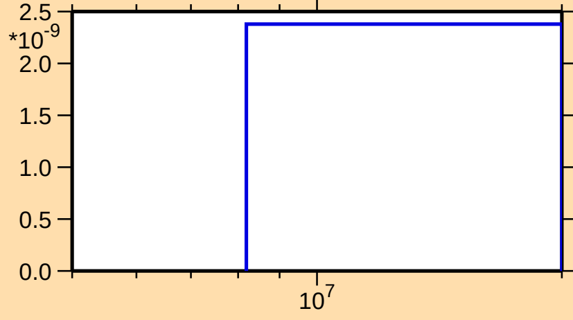
\sigma vs. E for ^{211}\text{Po}(n,\text{He}3)
