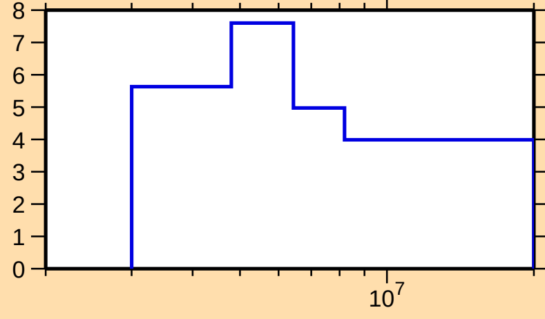
\Delta\sigma/\sigma vs. E for ^{211}\text{Po}(n,\text{nonel.})
