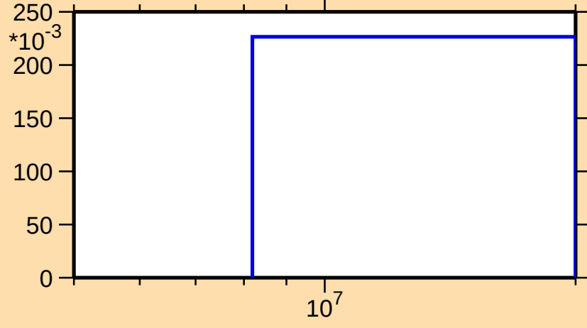
\sigma vs. E for ^{211}\text{Po}(n,3n)
