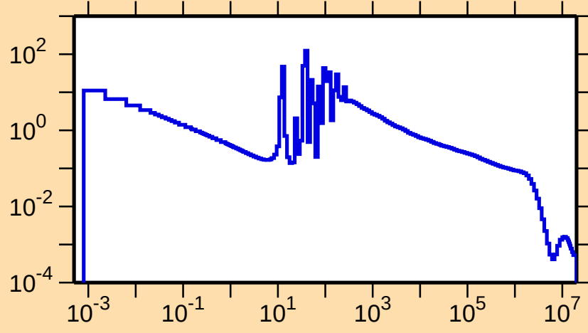
\sigma vs. E for ^{223}\text{Po}(n,\gamma)
