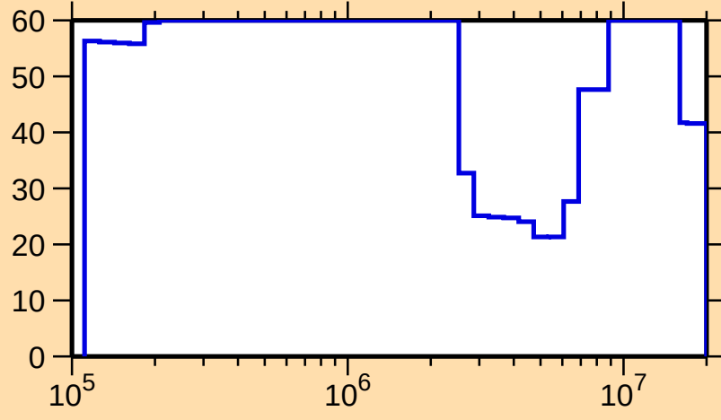
\Delta\sigma/\sigma vs. E for ^{223}\text{Po}(n,\text{el.})
