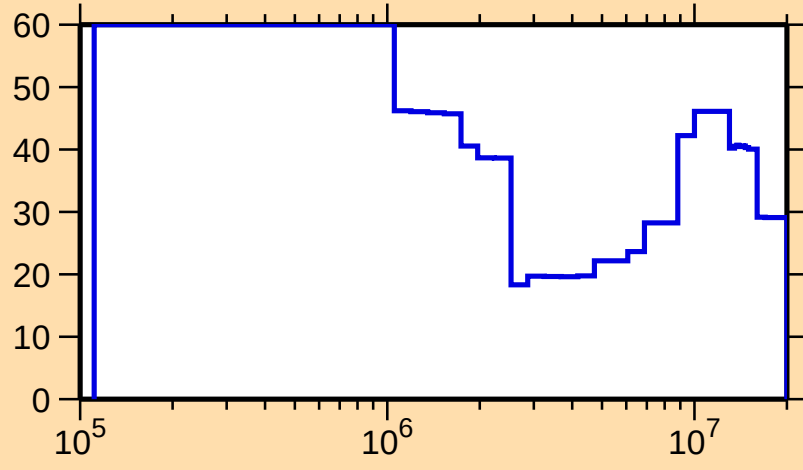
\Delta\sigma/\sigma vs. E for ^{223}\text{Po}(n,\text{tot.})
