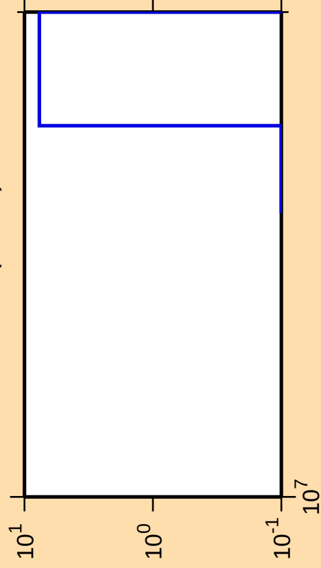
\Delta\sigma/\sigma vs. E for ^{223}\text{Po}(\text{mt 11})
