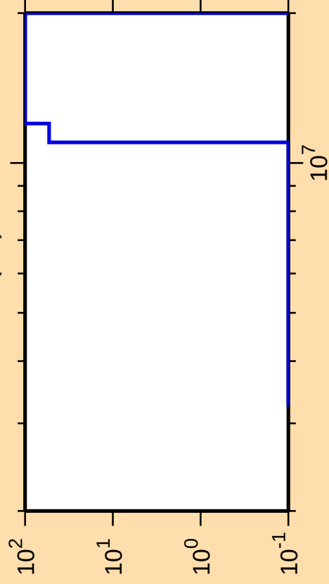
\Delta\sigma/\sigma vs. E for ^{223}\text{Po}(n,f)
