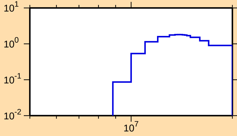
\sigma vs. E for ^{223}\text{Po}(n,3n)
