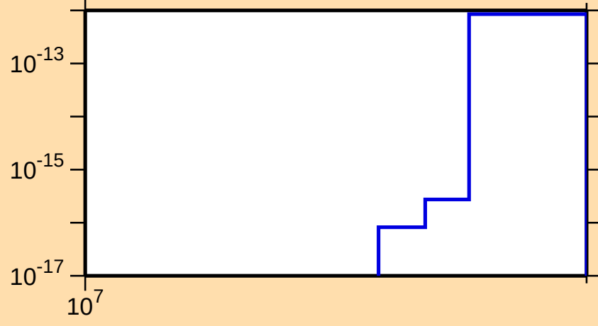
\sigma vs. E for ^{223}\text{Po}(\text{mt 11})
