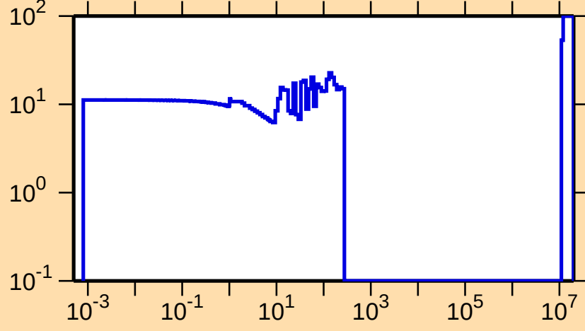
\Delta\sigma/\sigma vs. E for ^{223}\text{Po}(n,f)
