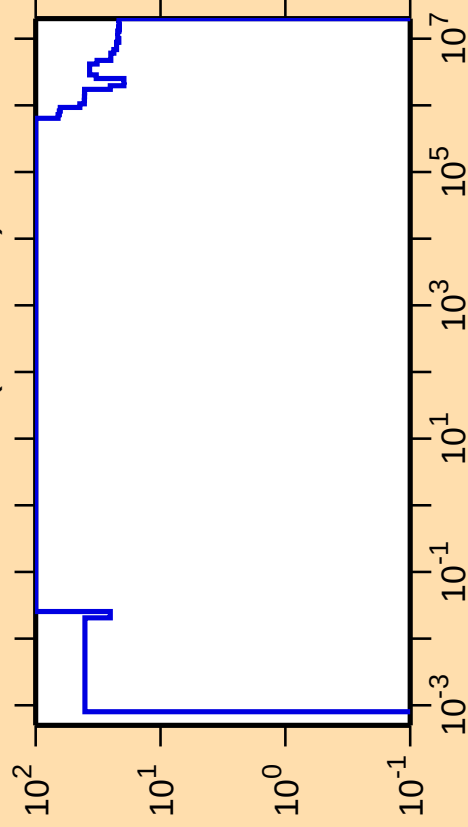
\Delta\sigma/\sigma vs. E for ^{223}\text{Po}(n,\text{nonel.})
