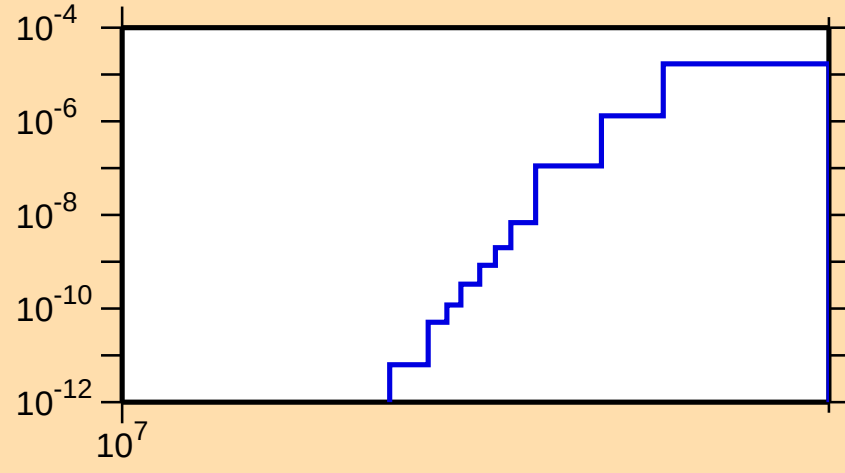
\sigma vs. E for ^{223}\text{Po}(n,nt)
