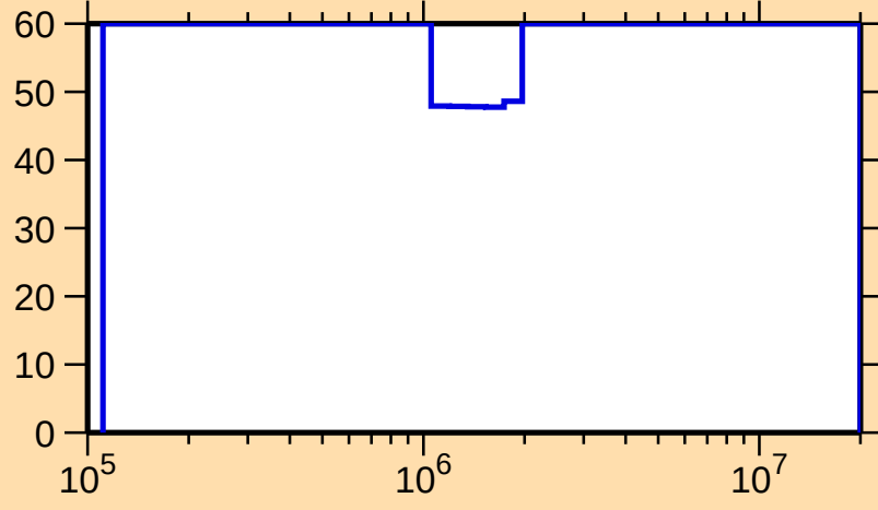
\Delta\sigma/\sigma vs. E for ^{223}\text{Po}(n,n_1)
