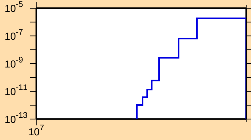
\sigma vs. E for ^{223}\text{Po}(n,\text{nd})
