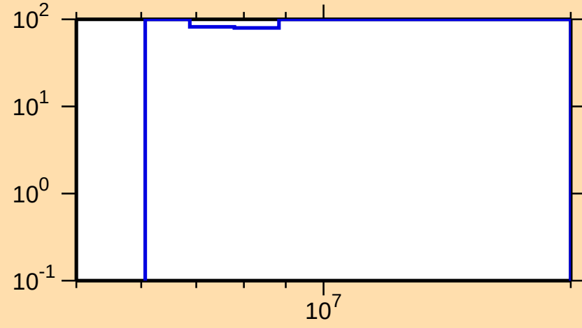
\Delta\sigma/\sigma vs. E for ^{223}\text{Po}(n,\gamma)
