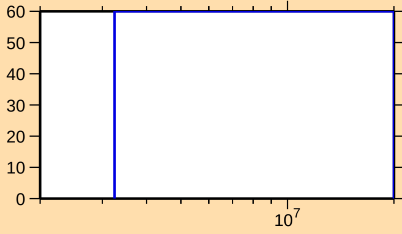
\Delta\sigma/\sigma vs. E for ^{223}\text{Po}(n,2n)
