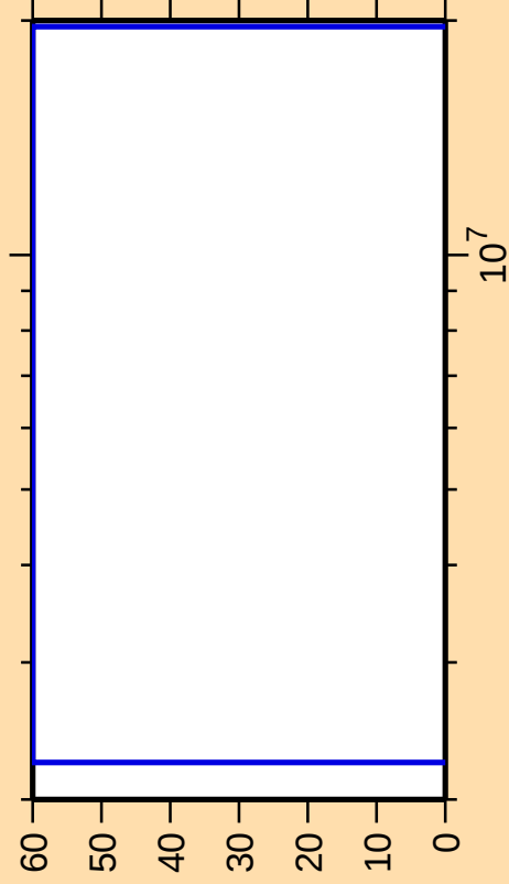
\Delta\sigma/\sigma vs. E for ^{223}\text{Po}(n,n_1)
