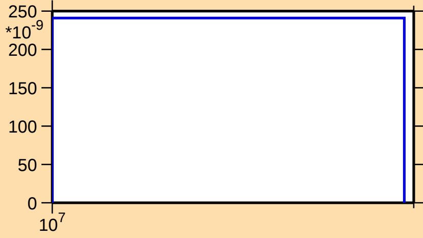
\sigma vs. E for ^{223}\text{Po}(n,nt)
