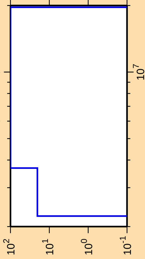
\Delta\sigma/\sigma vs. E for ^{223}\text{Po}(n,n\text{cont.})
