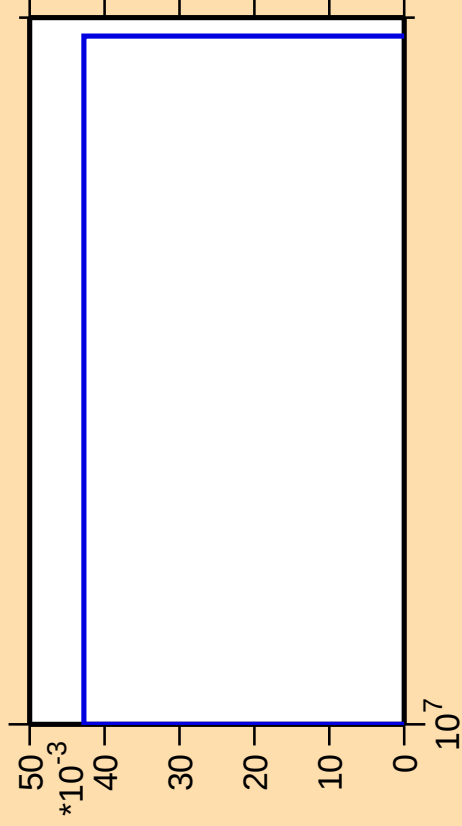
\Delta\sigma/\sigma vs. E for ^{223}\text{Po}(\text{mt } 11)
