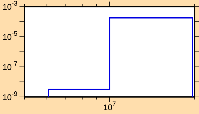
\sigma vs. E for ^{223}\text{Po}(n,p)
