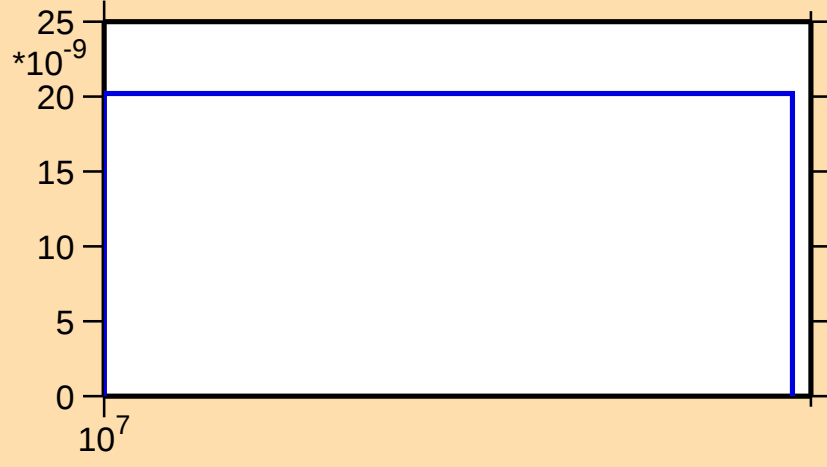
\sigma vs. E for ^{223}\text{Po}(n,\text{nd})
