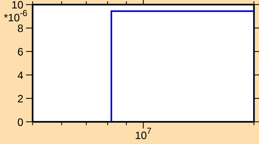
\sigma vs. E for ^{223}\text{Po}(n,d)
