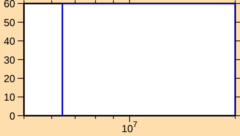
\Delta\sigma/\sigma vs. E for ^{223}\text{Po}(n,\text{ncont.})
