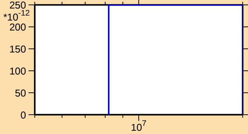
\sigma vs. E for ^{223}\text{Po}(n,3n\alpha)
