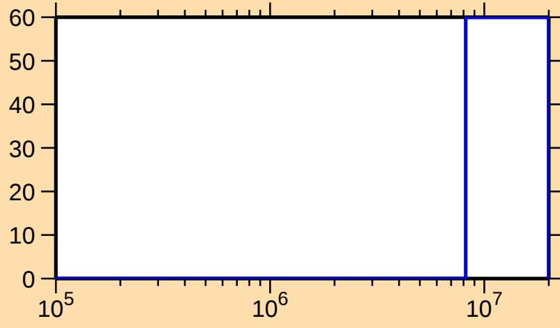
\Delta\sigma/\sigma vs. E for ^{223}\text{Po}(n,f)
