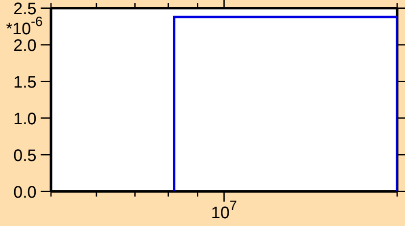
\sigma vs. E for ^{223}\text{Po}(n,np)
