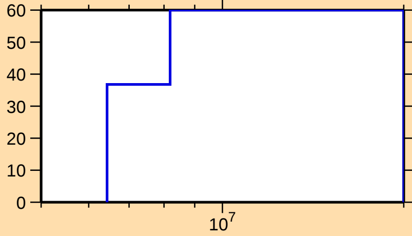
\Delta\sigma/\sigma vs. E for ^{223}\text{Po}(n,p)
