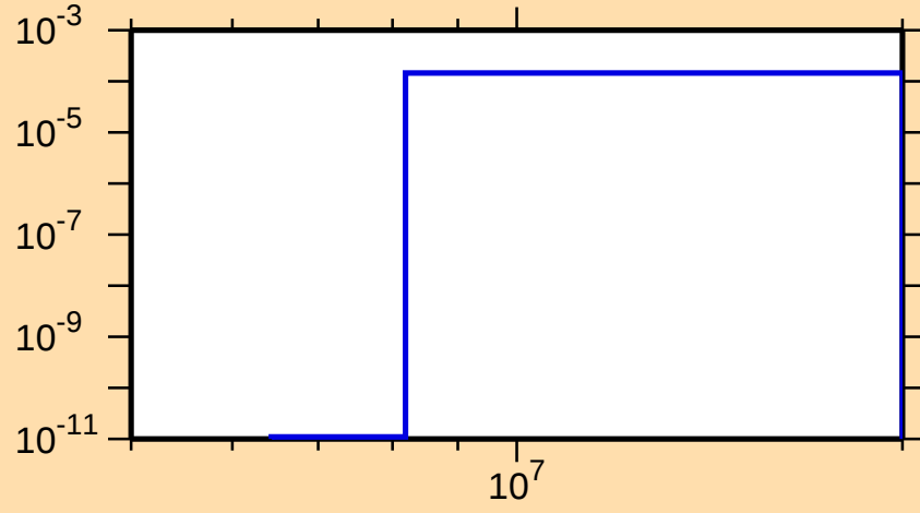
\sigma vs. E for ^{223}\text{Po}(n,p)
