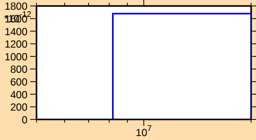
\sigma vs. E for ^{223}\text{Po}(n,2np)
