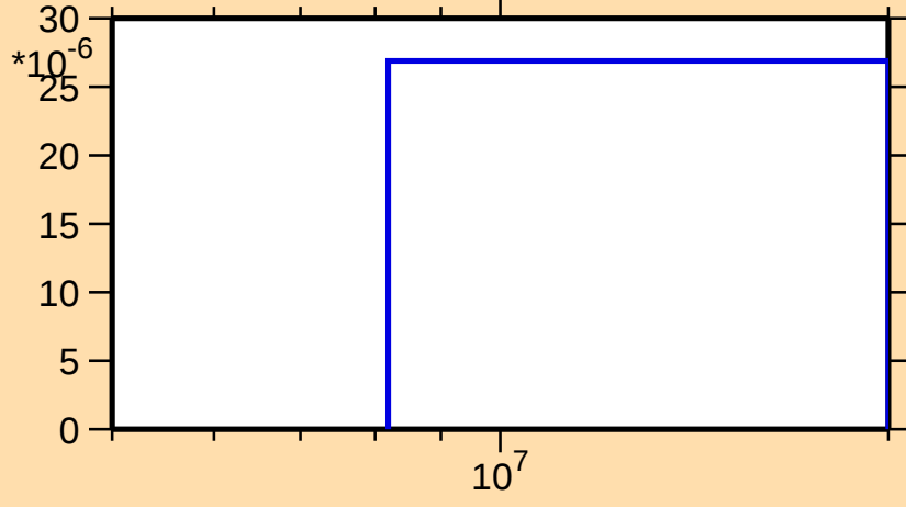
\sigma vs. E for ^{223}\text{Po}(n,t)
