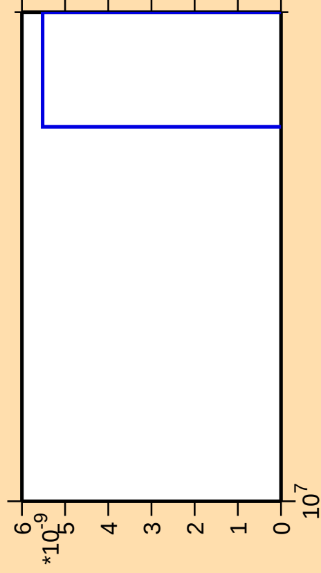
\Delta\sigma/\sigma vs. E for ^{226}\text{Po}(\text{mt } 42)
