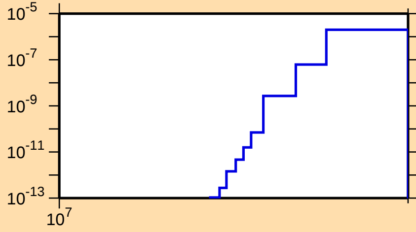
\sigma vs. E for ^{226}\text{Po}(n,nt)
