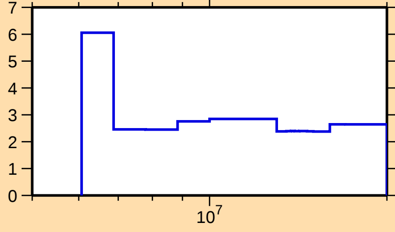
\Delta\sigma/\sigma vs. E for ^{226}\text{Po}(n,\text{nonel.})
