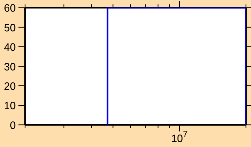
\Delta\sigma/\sigma vs. E for ^{226}\text{Po}(n,\text{inel.})
