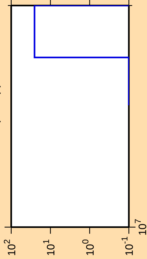
\Delta\sigma/\sigma vs. E for ^{226}\text{Po}(n,2np)
