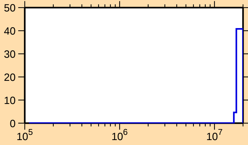
\Delta\sigma/\sigma vs. E for ^{226}\text{Po}(n,f)
