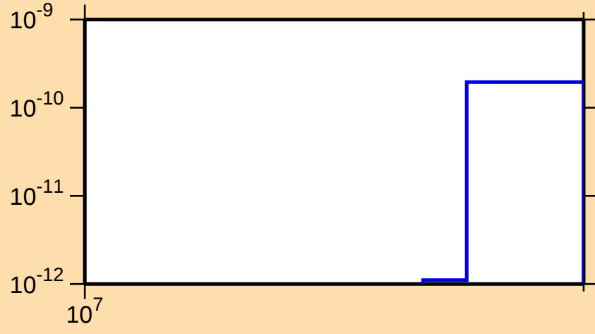
\sigma vs. E for ^{129}\text{Pr}(\text{mt 34})
