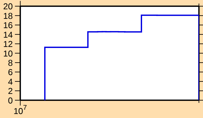
\Delta\sigma/\sigma vs. E for ^{129}\text{Pr}(n,\text{nonel.})
