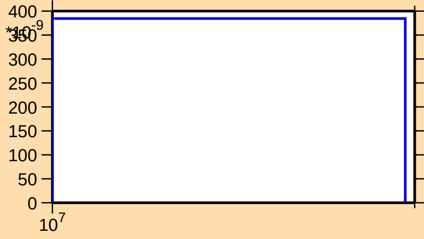
\sigma vs. E for ^{129}\text{Pr}(n,\text{nd})
