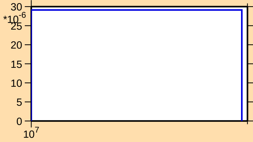
\sigma vs. E for ^{129}\text{Pr}(n,2np)
