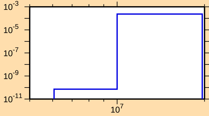
\sigma vs. E for ^{129}\text{Pr}(n,t)
