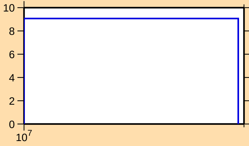
\Delta\sigma/\sigma vs. E for ^{129}\text{Pr}(n,\text{tot.})
