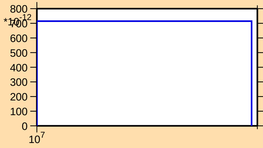
\sigma vs. E for ^{129}\text{Pr}(n,\text{pt})
