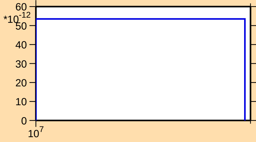
\sigma vs. E for ^{129}\text{Pr}(n,nt)
