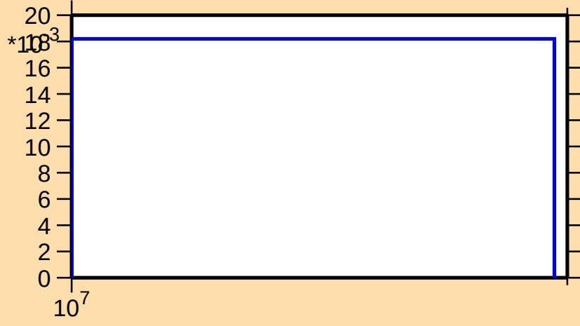
\sigma vs. E for ^{129}\text{Pr}(n,2n)
