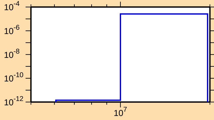
\sigma vs. E for ^{129}\text{Pr}(\text{mt 45})
