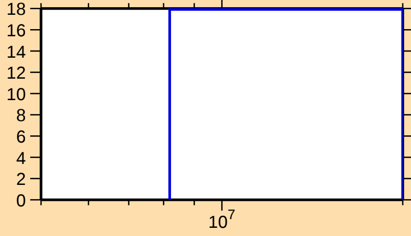
\Delta\sigma/\sigma vs. E for ^{129}\text{Pr}(n,\text{el.})
