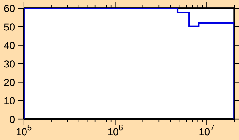
\Delta\sigma/\sigma vs. E for ^{129}\text{Pr}(n,n_1)
