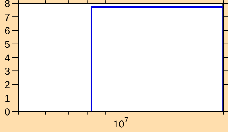
\Delta\sigma/\sigma vs. E for ^{129}\text{Pr}(n,\text{tot.})
