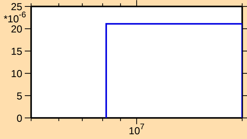
\sigma vs. E for ^{129}\text{Pr}(\text{mt } 45)
