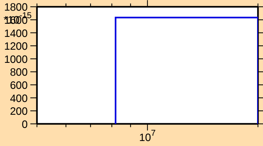
\sigma vs. E for ^{129}\text{Pr}(\text{mt } 34)
