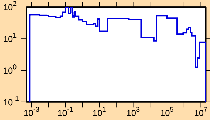
\Delta\sigma/\sigma vs. E for ^{129}\text{Pr}(n,\text{tot.})
