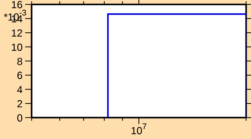
\sigma vs. E for ^{129}\text{Pr}(n,2n)
