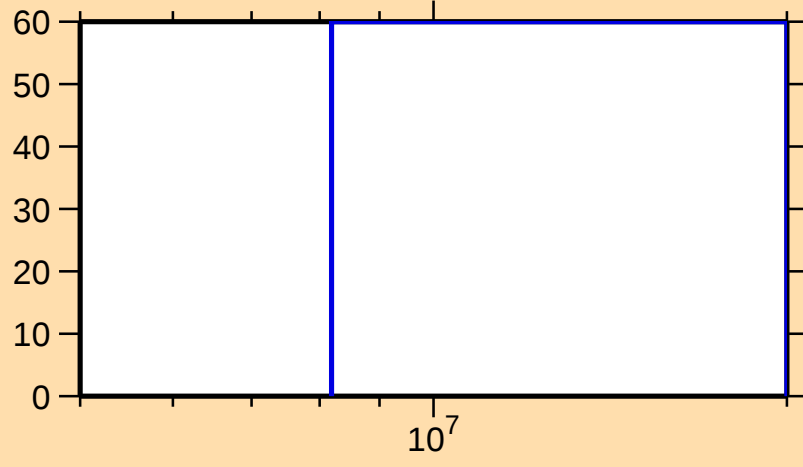
\Delta\sigma/\sigma vs. E for ^{129}\text{Pr}(n,\text{inel.})
