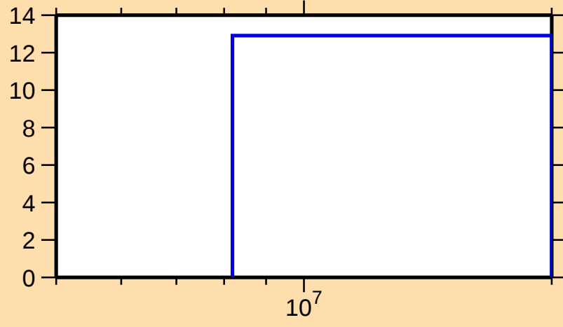
\Delta\sigma/\sigma vs. E for ^{129}\text{Pr}(n,\text{nonel.})
