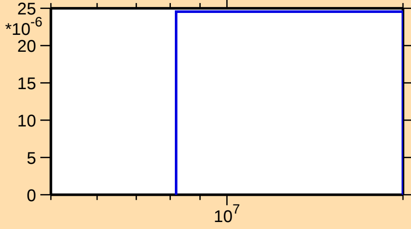
\sigma vs. E for ^{129}\text{Pr}(n,2np)
