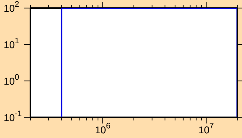
\Delta\sigma/\sigma vs. E for ^{129}\text{Pr}(n,\text{ncont.})
