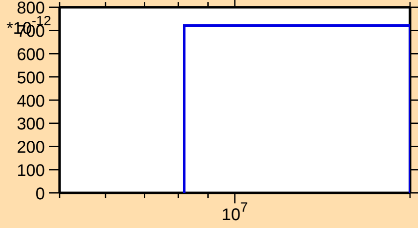
\sigma vs. E for ^{129}\text{Pr}(n,\text{pt})
