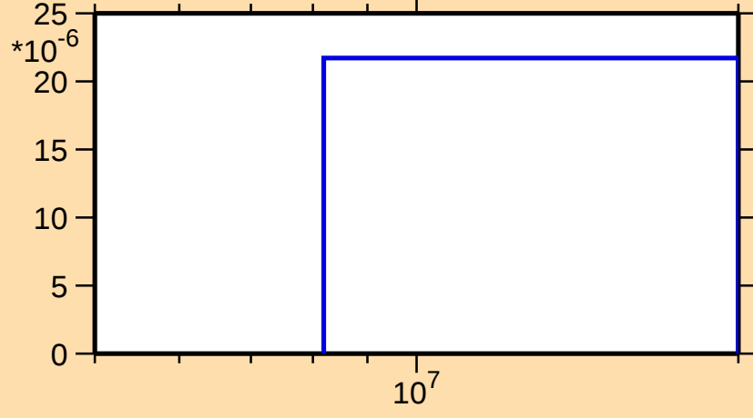
\sigma vs. E for ^{129}\text{Pr}(n,\text{pd})
