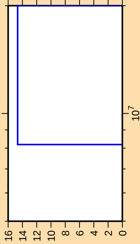
\Delta\sigma/\sigma vs. E for ^{129}\text{Pr}(\text{mt } 34)
