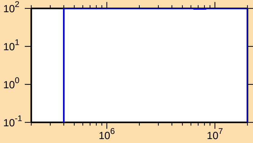
\Delta\sigma/\sigma vs. E for ^{129}\text{Pr}(n,n\text{cont.})
