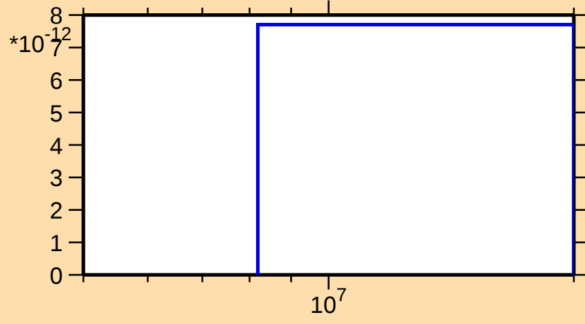
\sigma vs. E for ^{129}\text{Pr}(n,2n\alpha)
