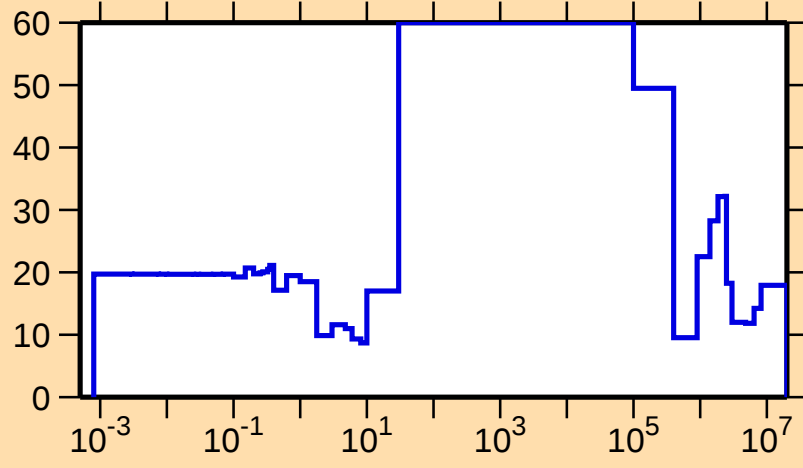
\Delta\sigma/\sigma vs. E for ^{129}\text{Pr}(n,\text{el.})
