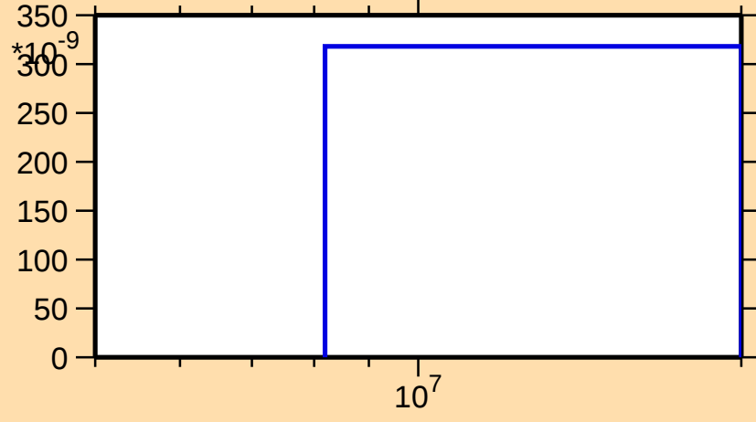
\sigma vs. E for ^{129}\text{Pr}(n,\text{nd})
