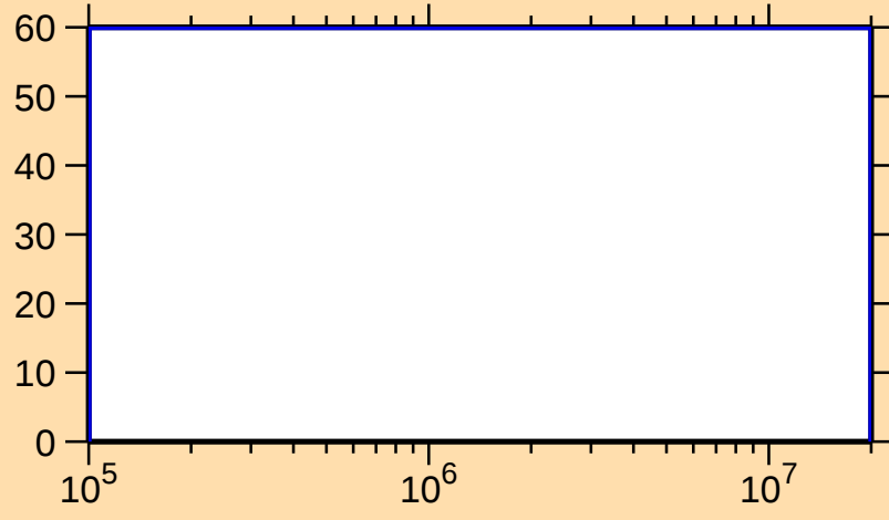
\Delta\sigma/\sigma vs. E for ^{129}\text{Pr}(n,\text{inel.})
