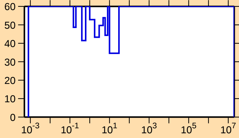
\Delta\sigma/\sigma vs. E for ^{129}\text{Pr}(n,\gamma)
