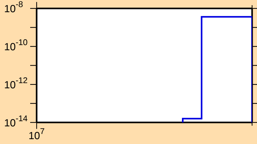
\sigma vs. E for ^{130}\text{Pr}(n,nt)
