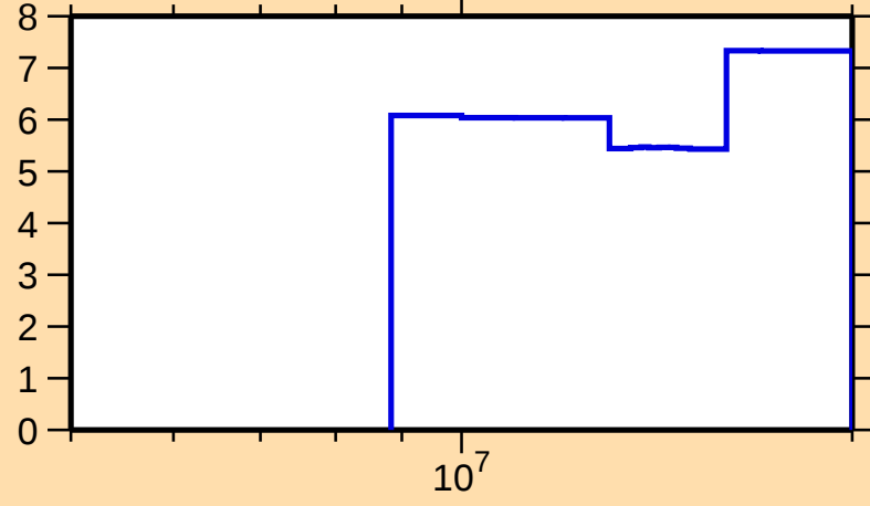
\Delta\sigma/\sigma vs. E for ^{130}\text{Pr}(n,\text{el.})
