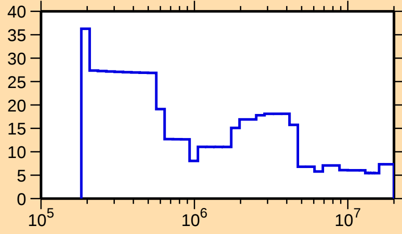
\Delta\sigma/\sigma vs. E for ^{130}\text{Pr}(n,\text{el.})
