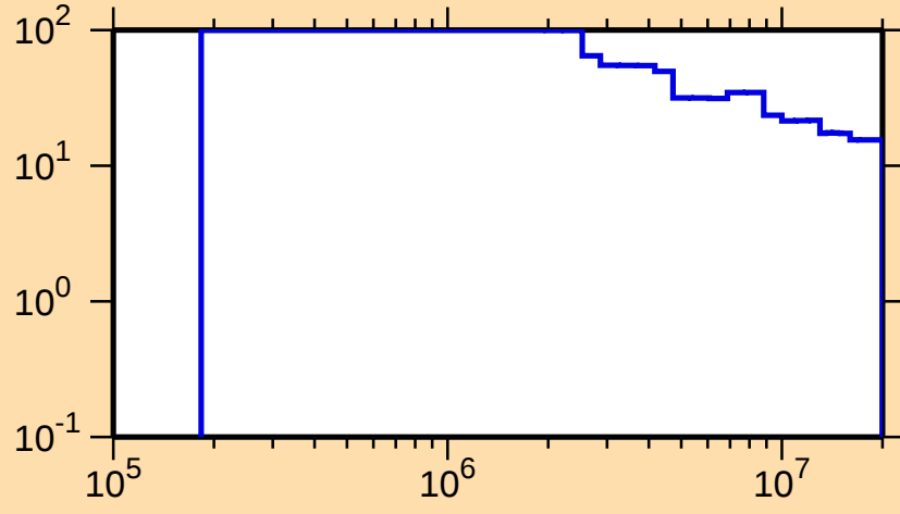
\Delta\sigma/\sigma vs. E for ^{130}\text{Pr}(n,n\text{cont.})
