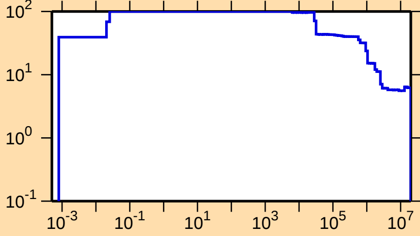
\Delta\sigma/\sigma vs. E for ^{130}\text{Pr}(n,\text{nonel.})
