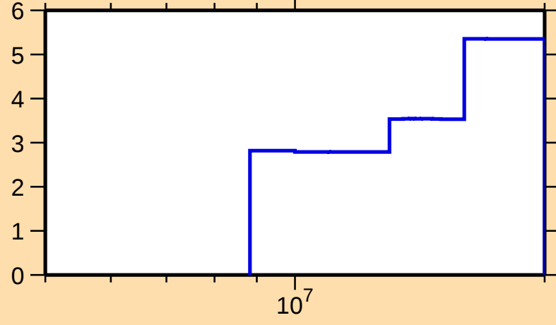
\Delta\sigma/\sigma vs. E for ^{130}\text{Pr}(n,\text{tot.})
