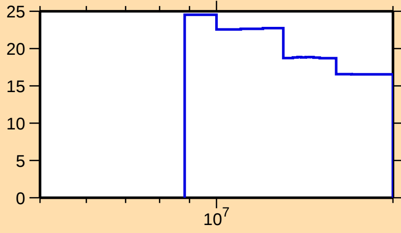
\Delta\sigma/\sigma vs. E for ^{130}\text{Pr}(n,\text{inel.})
