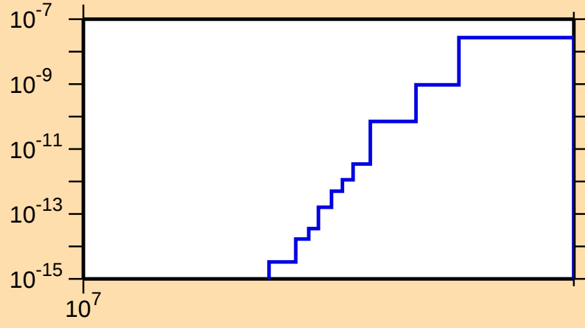
\sigma vs. E for ^{130}\text{Pr}(\text{mt } 34)
