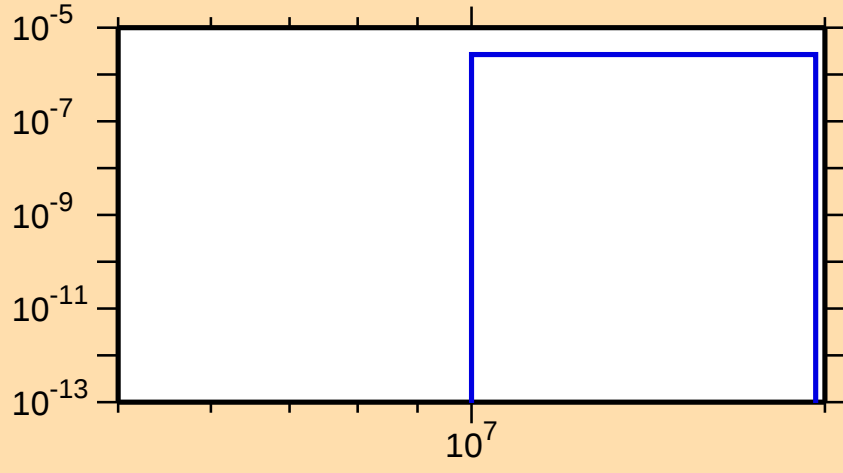
\sigma vs. E for ^{130}\text{Pr}(\text{mt 45})
