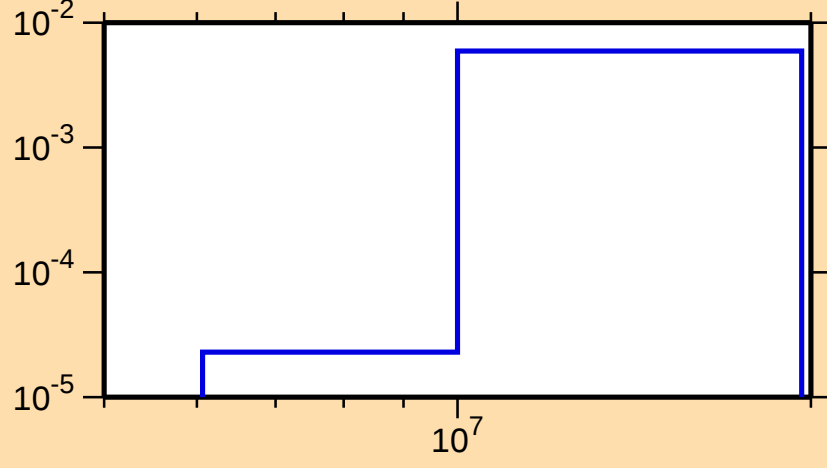
\sigma vs. E for ^{130}\text{Pr}(n,2n)
