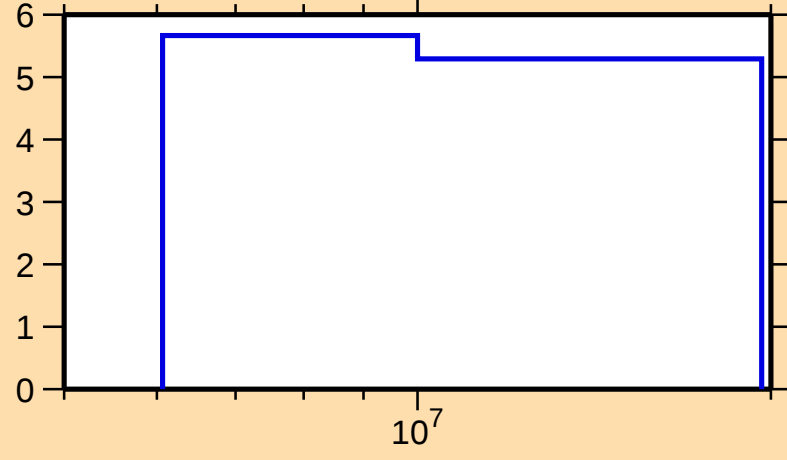
\Delta\sigma/\sigma vs. E for ^{130}\text{Pr}(n,\text{el.})
