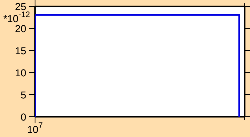
\sigma vs. E for ^{130}\text{Pr}(n,\text{nt})
