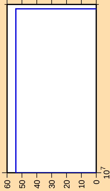
\Delta\sigma/\sigma vs. E for ^{130}\text{Pr}(n,2np)
