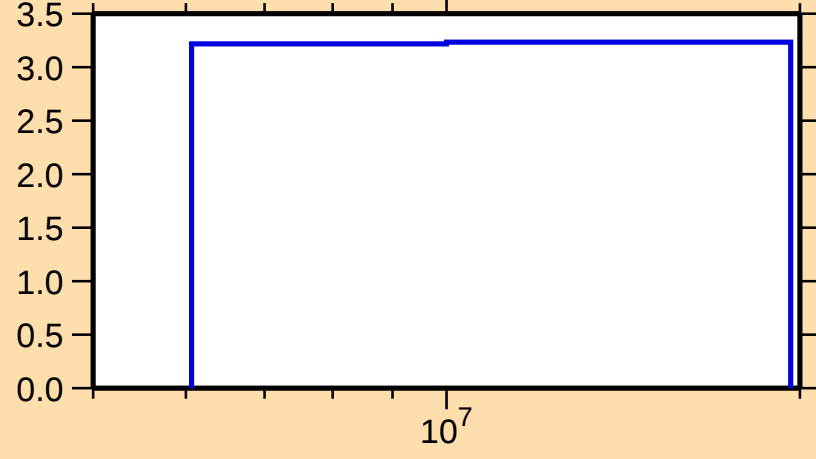
\Delta\sigma/\sigma vs. E for ^{130}\text{Pr}(n,\text{tot.})
