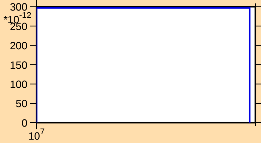
\sigma vs. E for ^{130}\text{Pr}(\text{mt } 34)
