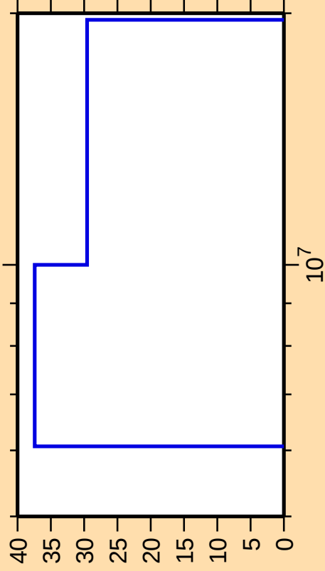
\Delta\sigma/\sigma vs. E for ^{130}\text{Pr}(n,n_1)
