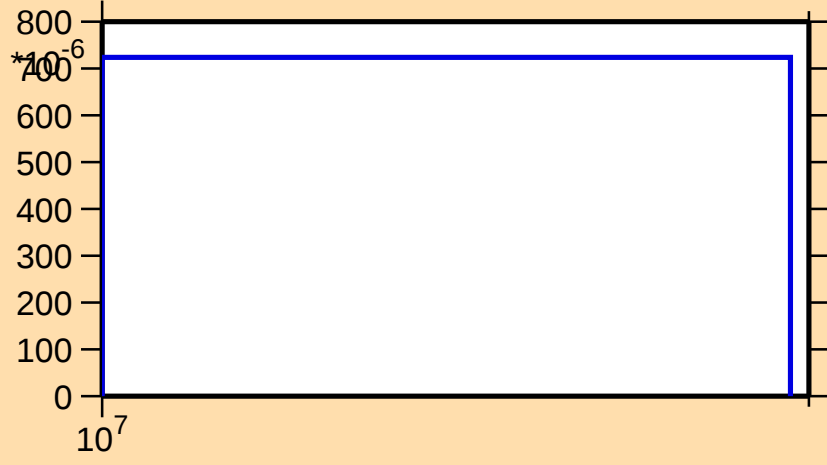
\sigma vs. E for ^{130}\text{Pr}(n,2np)
