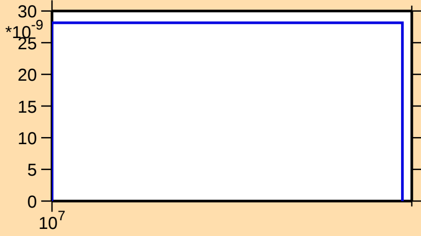
\sigma vs. E for ^{130}\text{Pr}(n,2n\alpha)
