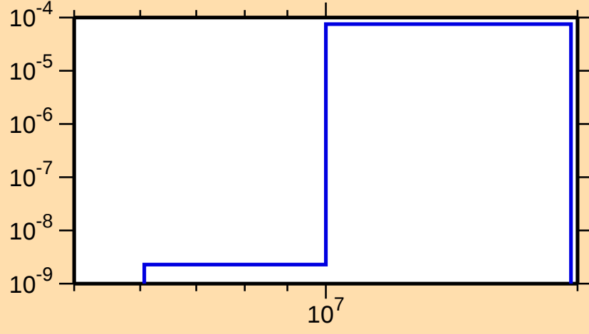
\sigma vs. E for ^{130}\text{Pr}(n,\text{He3})
