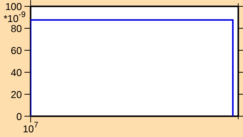
\sigma vs. E for ^{130}\text{Pr}(n,\text{pt})
