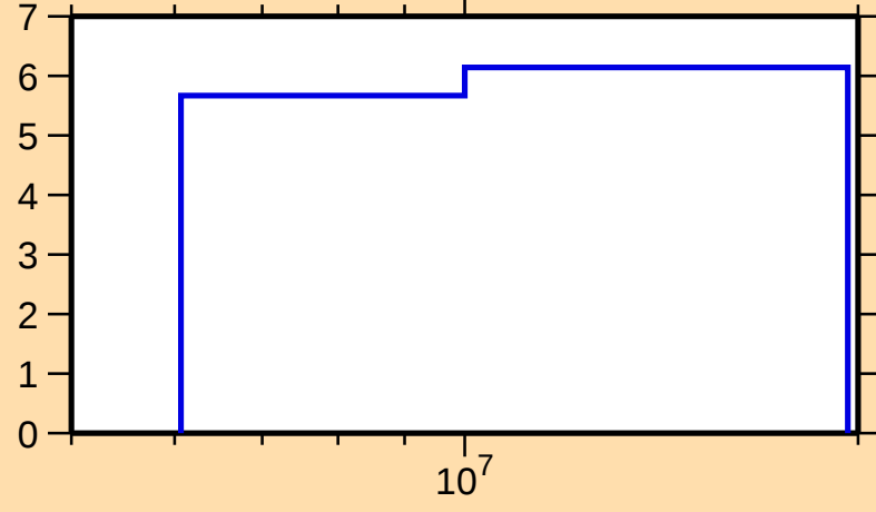
\Delta\sigma/\sigma vs. E for ^{130}\text{Pr}(n,\text{nonel.})
