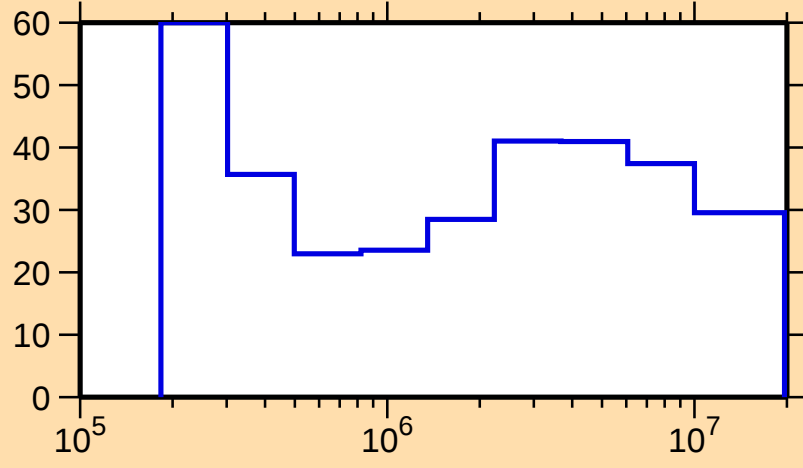
\Delta\sigma/\sigma vs. E for ^{130}\text{Pr}(n,n_1)
