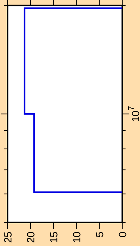
\Delta\sigma/\sigma vs. E for ^{130}\text{Pr}(n,p)
