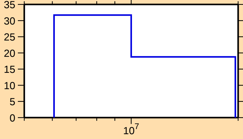
\Delta\sigma/\sigma vs. E for ^{130}\text{Pr}(n,\text{inel.})
