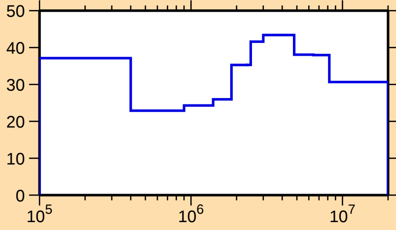
\Delta\sigma/\sigma vs. E for ^{130}\text{Pr}(n,n_1)
