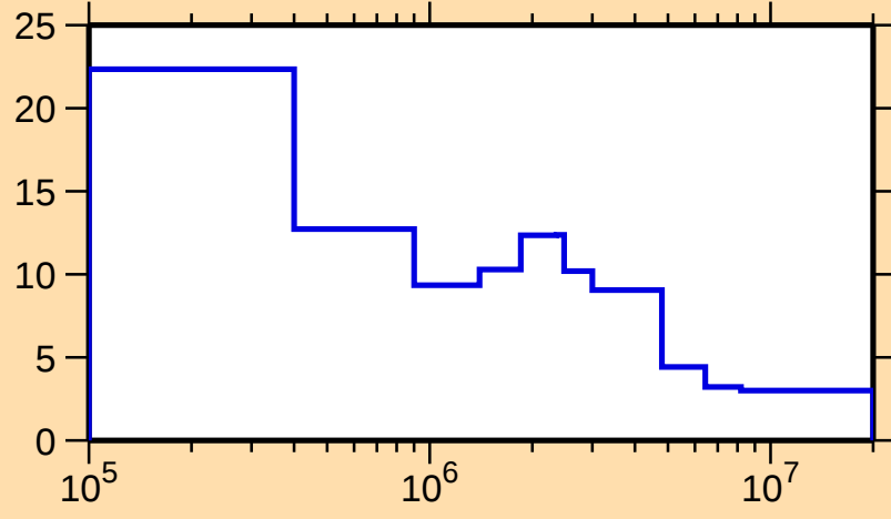
\Delta\sigma/\sigma vs. E for ^{130}\text{Pr}(n,\text{tot.})
