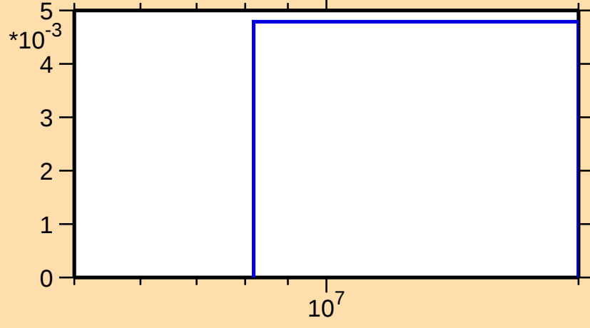
\sigma vs. E for ^{130}\text{Pr}(n,2n)
