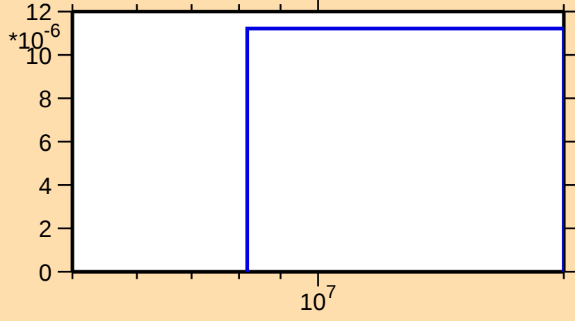
\sigma vs. E for ^{130}\text{Pr}(n,\text{nd})
