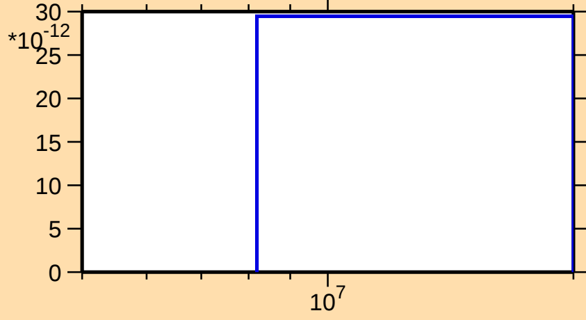
\sigma vs. E for ^{130}\text{Pr}(n,nt)
