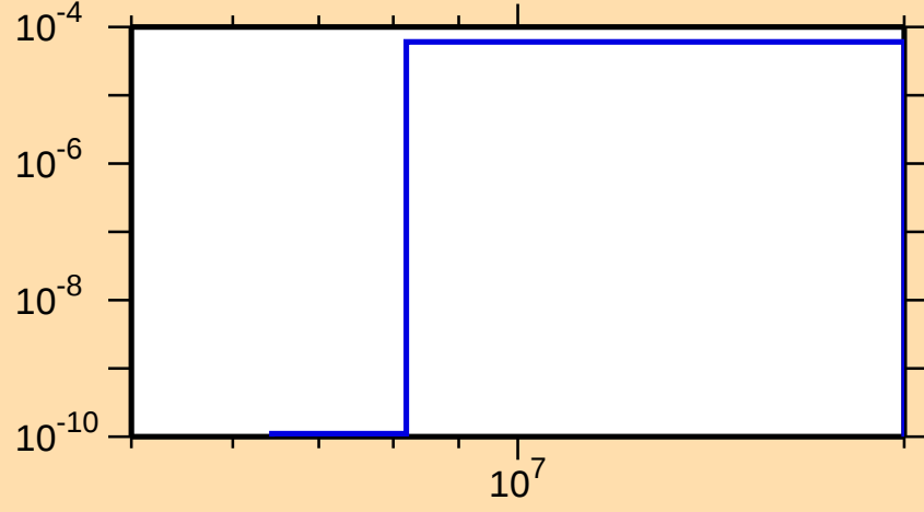
\sigma vs. E for ^{130}\text{Pr}(n,\text{He3})
