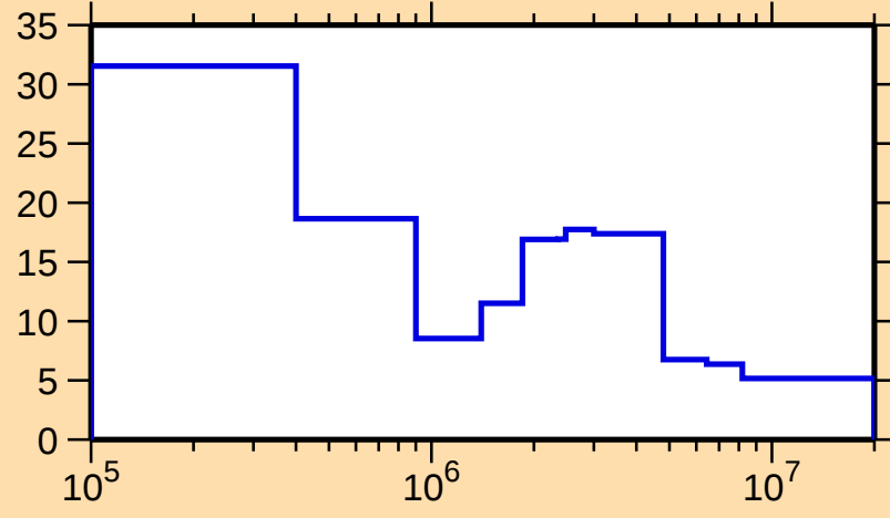
\Delta\sigma/\sigma vs. E for ^{130}\text{Pr}(n,\text{el.})
