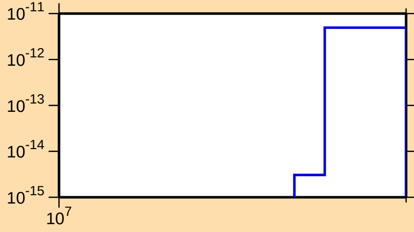
\sigma vs. E for ^{133}\text{Pr}(\text{mt } 34)
