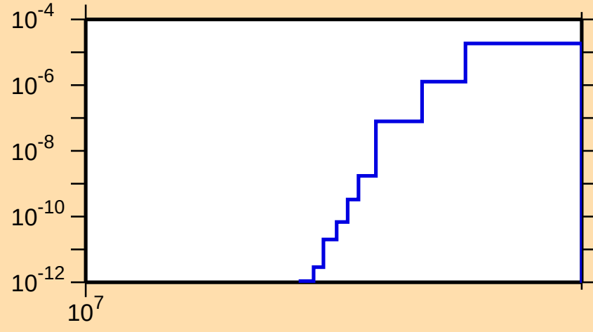
\sigma vs. E for ^{133}\text{Pr}(n,\text{nd})
