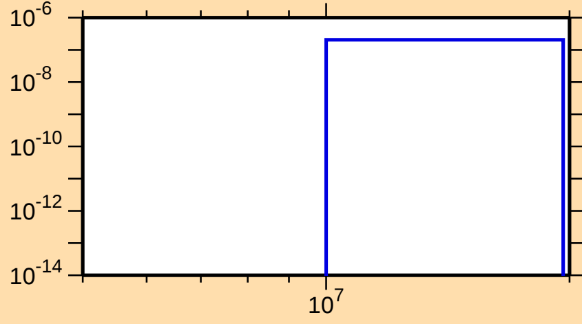
\sigma vs. E for ^{133}\text{Pr}(\text{mt 45})
