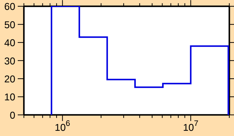
\Delta\sigma/\sigma vs. E for ^{133}\text{Pr}(n,n\text{cont.})
