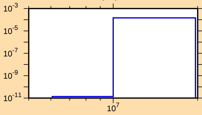
\sigma vs. E for ^{133}\text{Pr}(n,t)
