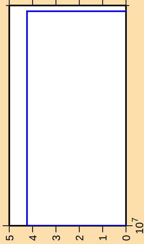
\Delta\sigma/\sigma vs. E for ^{133}\text{Pr}(n,\text{pt})
