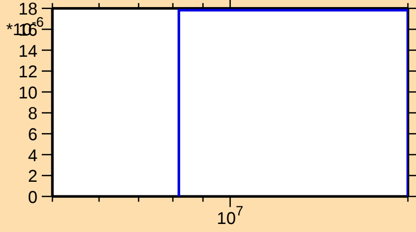
\sigma vs. E for ^{133}\text{Pr}(n,2np)
