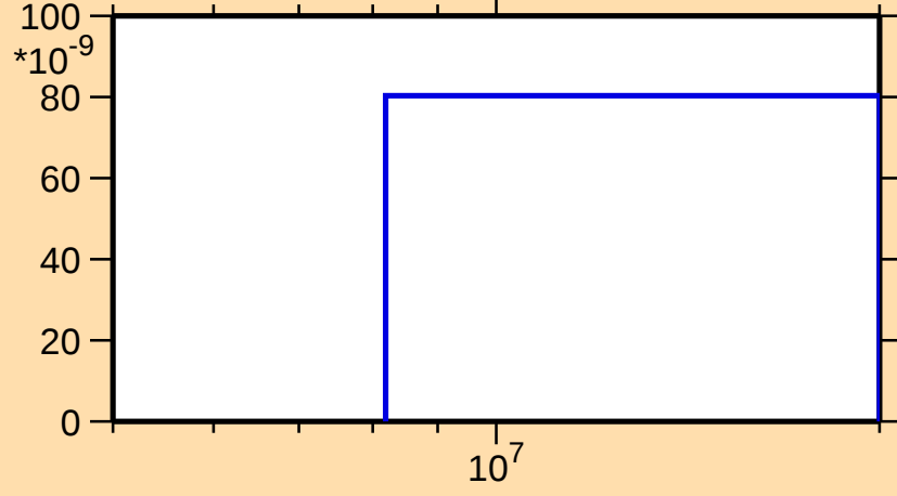
\sigma vs. E for ^{133}\text{Pr}(n,\text{pd})
