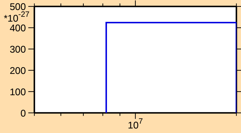
\sigma vs. E for ^{133}\text{Pr}(\text{mt } 11)
