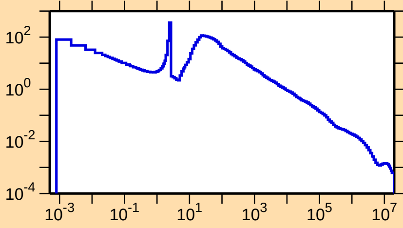
\sigma vs. E for ^{142}\text{Pr}(n,\gamma)
