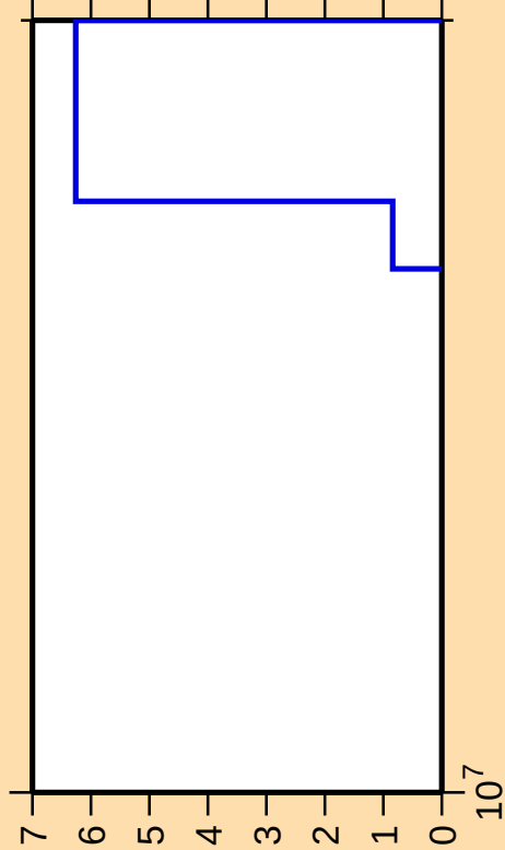
\Delta\sigma/\sigma vs. E for ^{142}\text{Pr}(\text{mt117})
