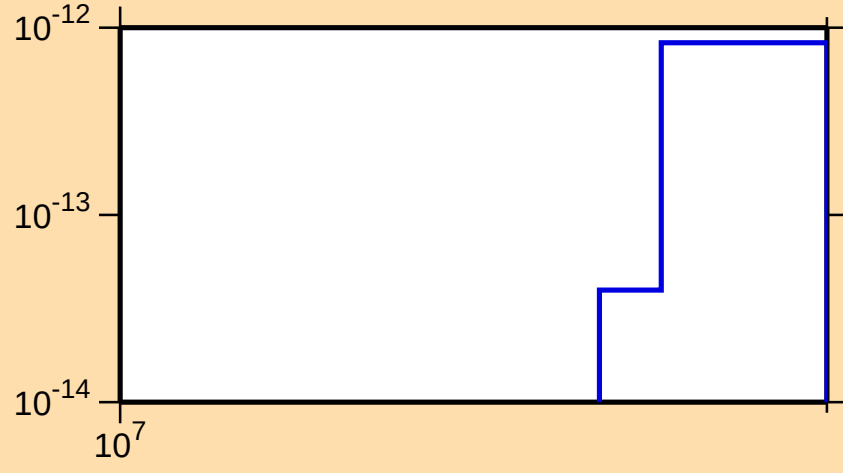
\sigma vs. E for ^{142}\text{Pr}(\text{mt 45})
