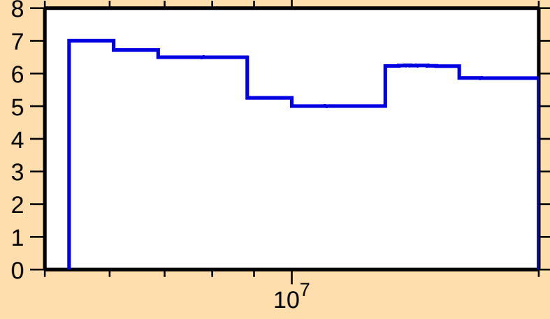
\Delta\sigma/\sigma vs. E for ^{142}\text{Pr}(n,\text{nonel.})
