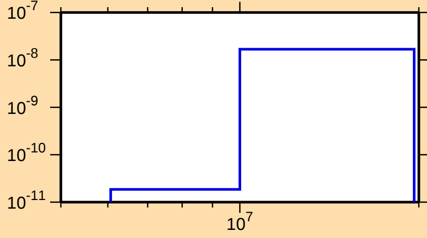
\sigma vs. E for ^{142}\text{Pr}(n,p\alpha)
