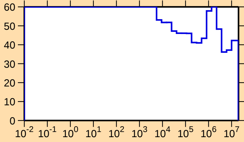
\Delta\sigma/\sigma vs. E for ^{142}\text{Pr}(n,p)
