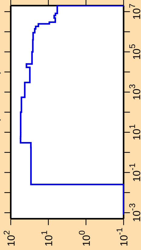
\Delta\sigma/\sigma vs. E for ^{142}\text{Pr}(n,\text{nonel.})
