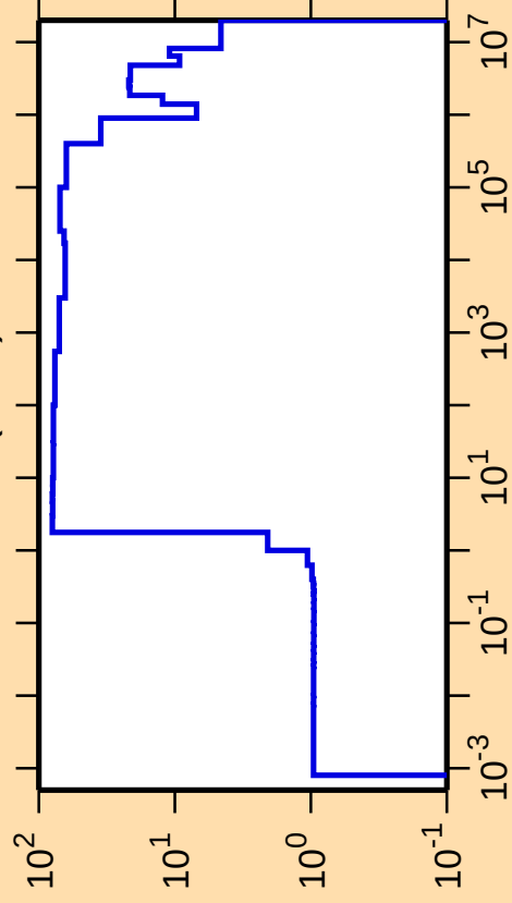
\Delta\sigma/\sigma vs. E for ^{142}\text{Pr}(n,\text{el.})
