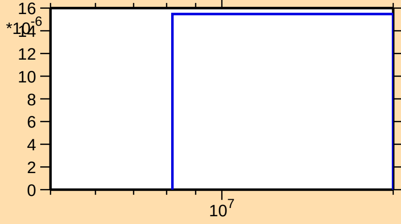
\sigma vs. E for ^{142}\text{Pr}(n,2np)
