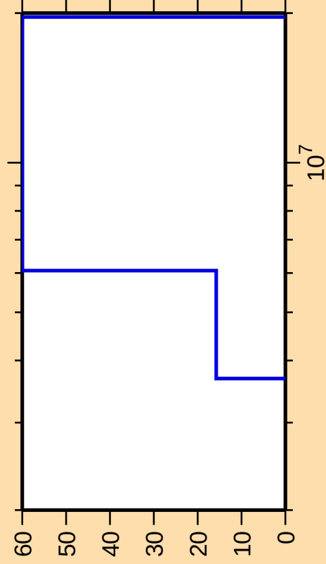
\Delta\sigma/\sigma vs. E for ^{142}\text{Pr}(n,n\alpha)
