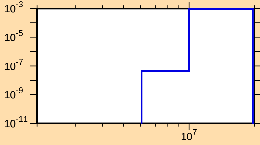
\sigma vs. E for ^{142}\text{Pr}(n,n\alpha)
