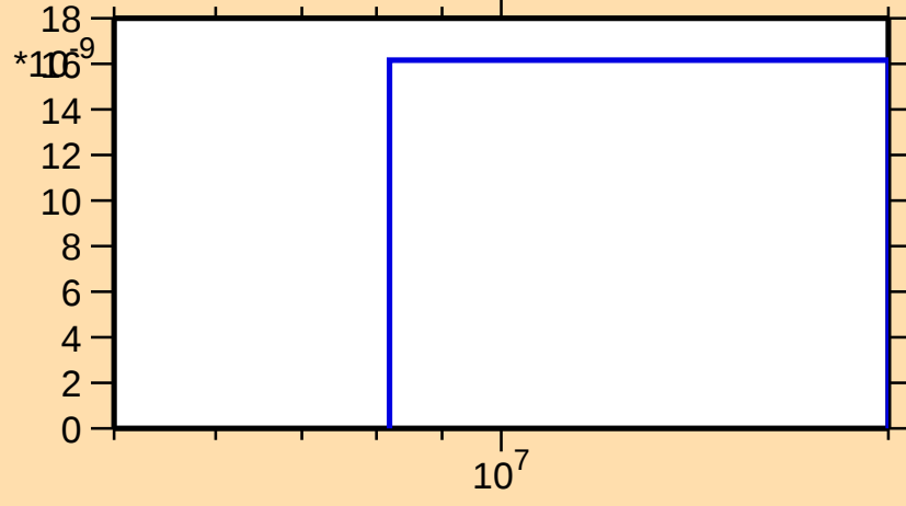
\sigma vs. E for ^{142}\text{Pr}(n,nt)
