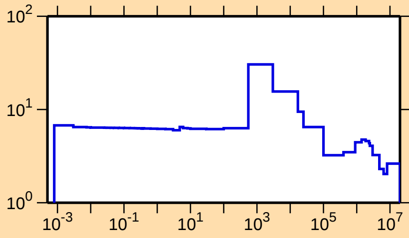
\sigma vs. E for ^{142}\text{Pr}(n,\text{el.})
