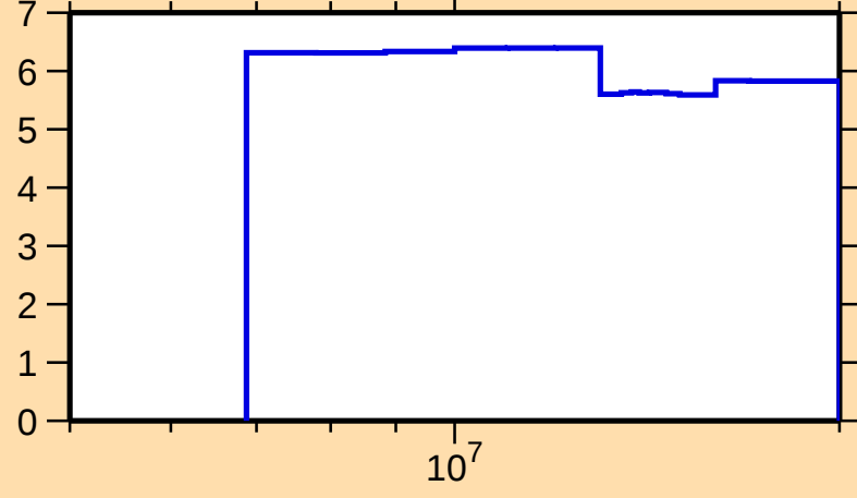
\Delta\sigma/\sigma vs. E for ^{143}\text{Pr}(n,\text{nonel.})
