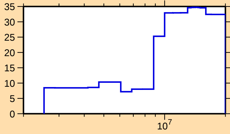
\Delta\sigma/\sigma vs. E for ^{143}\text{Pr}(n,n\text{cont.})
