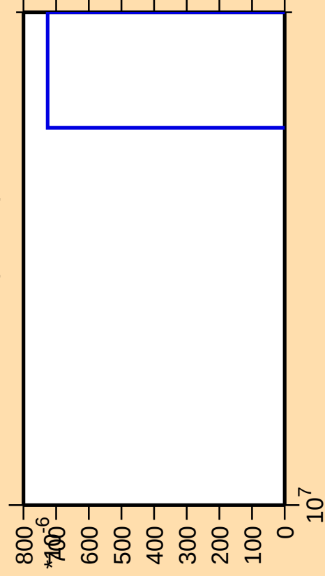
\Delta\sigma/\sigma vs. E for ^{143}\text{Pr}(\text{mt } 42)
