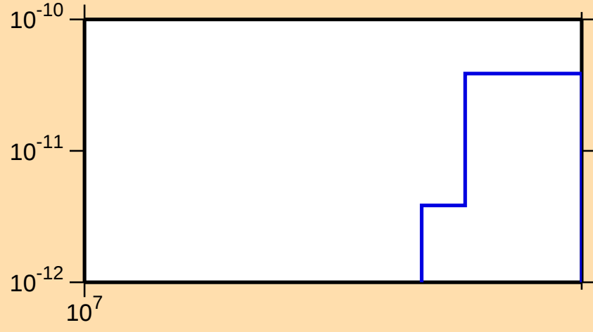
\sigma vs. E for ^{143}\text{Pr}(\text{mt 45})
