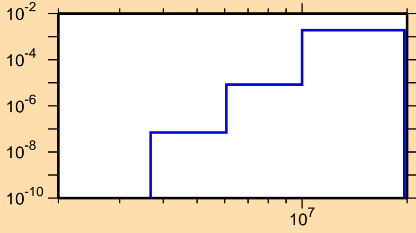
\sigma vs. E for ^{143}\text{Pr}(n,n\alpha)
