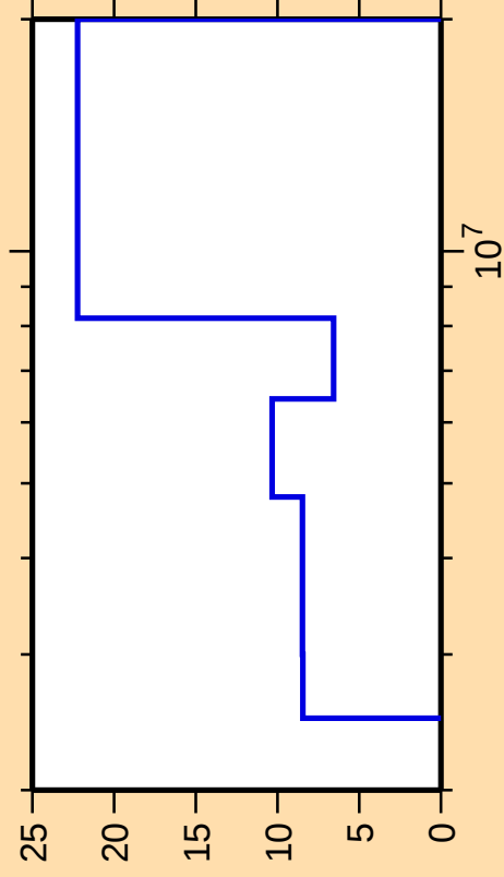
\Delta\sigma/\sigma vs. E for ^{143}\text{Pr}(\text{n},\text{ncont.})
