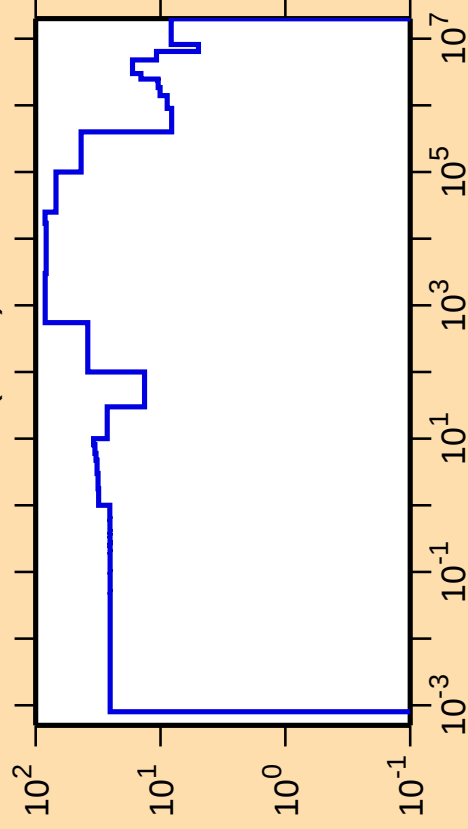
\Delta\sigma/\sigma vs. E for ^{143}\text{Pr}(n,\text{el.})
