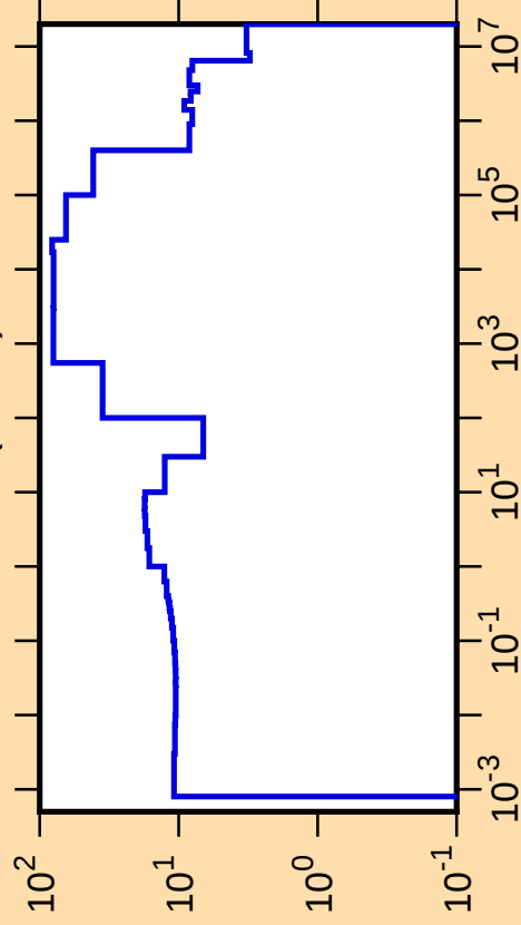
\Delta\sigma/\sigma vs. E for ^{143}\text{Pr}(n,\text{tot.})
