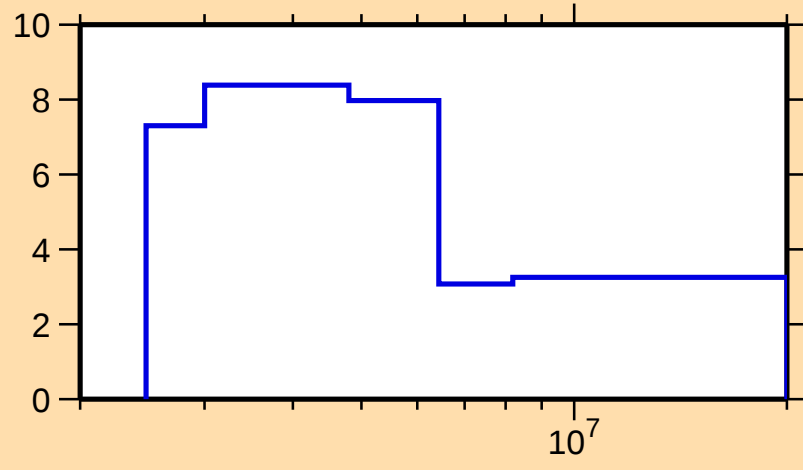
\Delta\sigma/\sigma vs. E for ^{143}\text{Pr}(n,\text{tot.})
