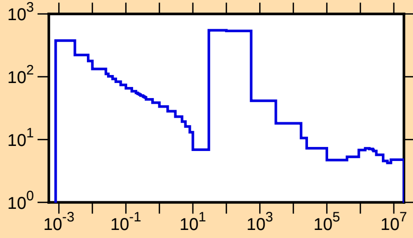
\sigma vs. E for ^{143}\text{Pr}(n,\text{tot.})
