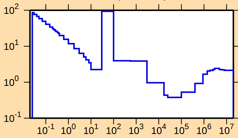
\sigma vs. E for ^{143}\text{Pr}(n,\text{nonel.})
