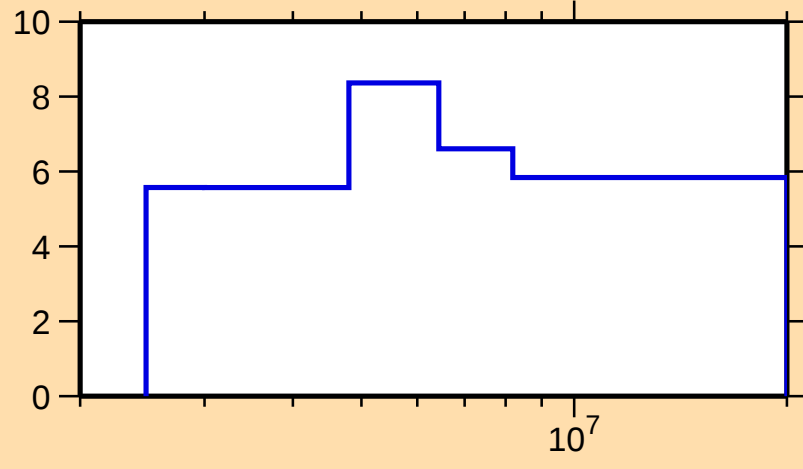
\Delta\sigma/\sigma vs. E for ^{143}\text{Pr}(\text{n},\text{nonel.})
