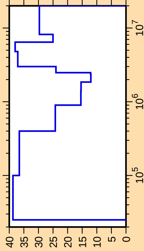
\Delta\sigma/\sigma vs. E for ^{143}\text{Pr}(n,n_1)
