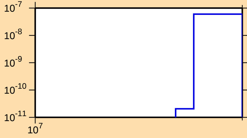
\sigma vs. E for ^{152}\text{Pr}(n,2np)
