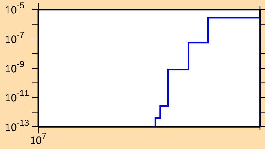
\sigma vs. E for ^{152}\text{Pr}(n,\text{nd})
