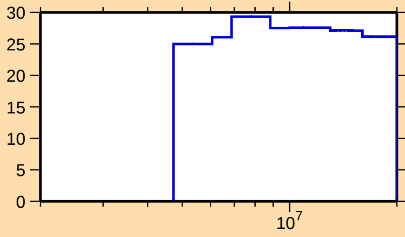
\Delta\sigma/\sigma vs. E for ^{152}\text{Pr}(n,\text{nonel.})
