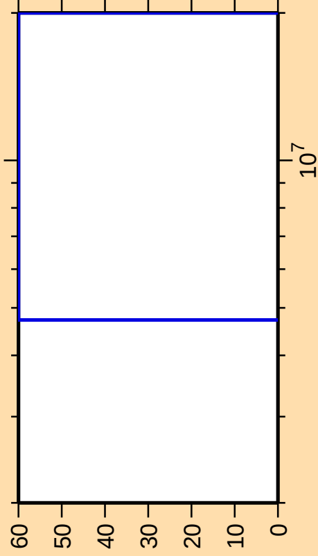
\Delta\sigma/\sigma vs. E for ^{152}\text{Pr}(n,n\text{cont.})
