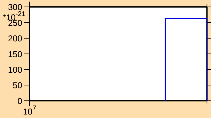
\sigma vs. E for ^{152}\text{Pr}(\text{mt 11})
