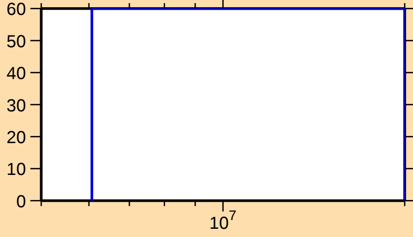
\Delta\sigma/\sigma vs. E for ^{152}\text{Pr}(n,\gamma)
