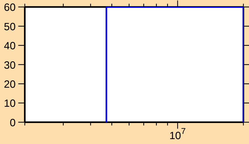
\Delta\sigma/\sigma vs. E for ^{152}\text{Pr}(n,2n)
