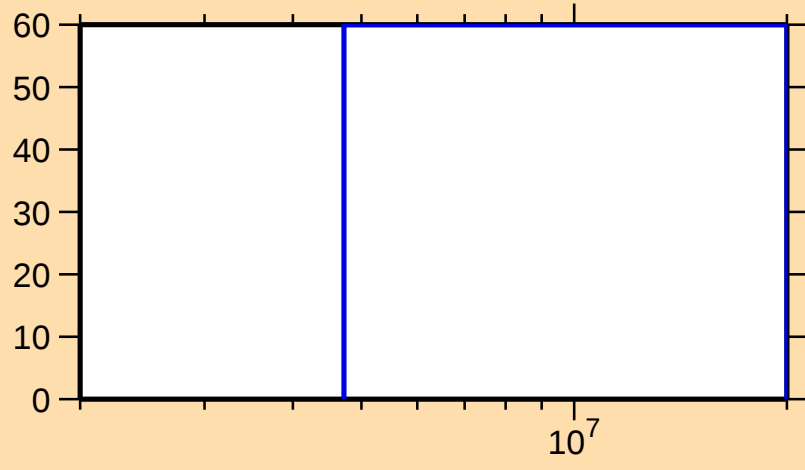
\Delta\sigma/\sigma vs. E for ^{152}\text{Pr}(n,\text{inel.})
