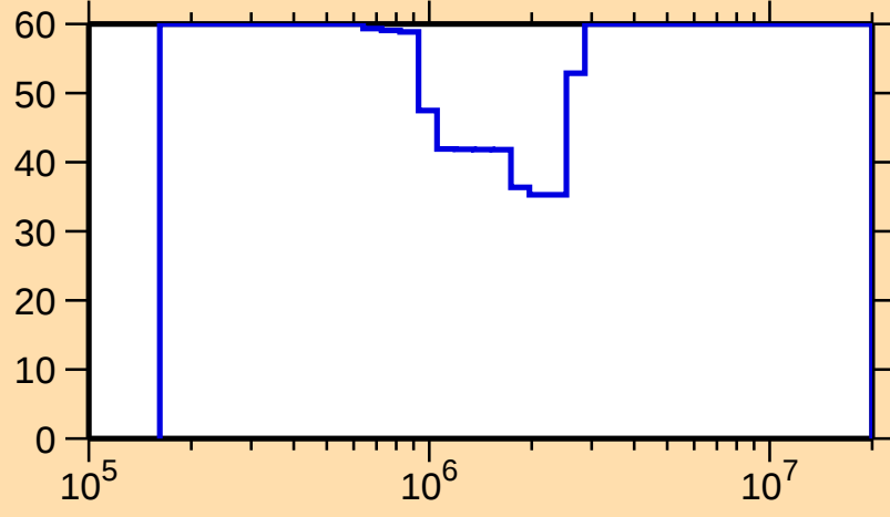
\Delta\sigma/\sigma vs. E for ^{152}\text{Pr}(n,\text{el.})
