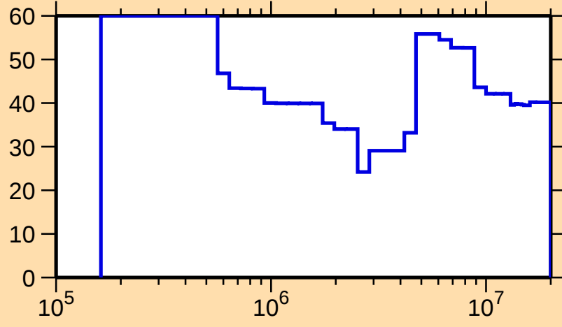
\Delta\sigma/\sigma vs. E for ^{152}\text{Pr}(n,\text{tot.})
