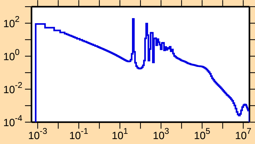
\sigma vs. E for ^{152}\text{Pr}(n,\gamma)
