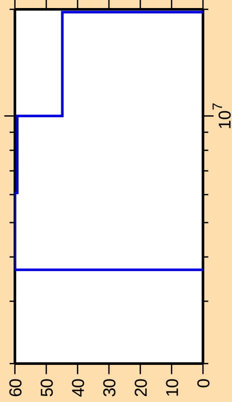
\Delta\sigma/\sigma vs. E for ^{152}\text{Pr}(n,n_1)
