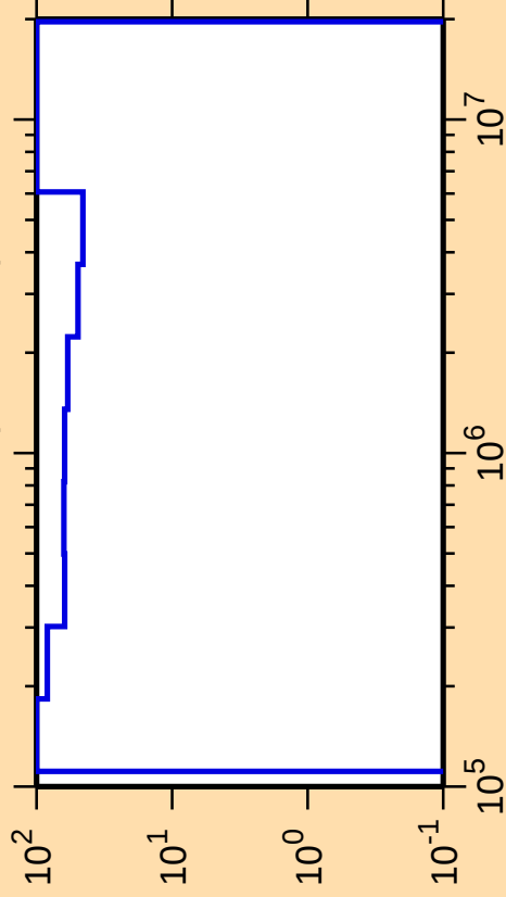
\Delta\sigma/\sigma vs. E for ^{152}\text{Pr}(n,\text{ncont.})
