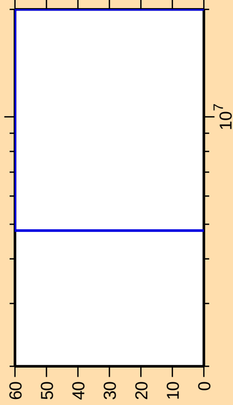
\Delta\sigma/\sigma vs. E for ^{152}\text{Pr}(n,\gamma)
