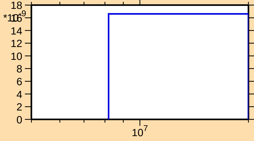
\sigma vs. E for ^{152}\text{Pr}(n,\text{nt})
