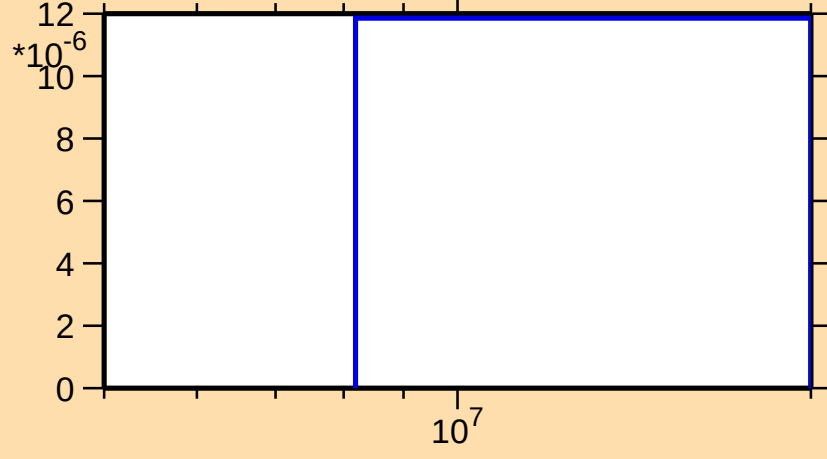
\sigma vs. E for ^{152}\text{Pr}(n,np)
