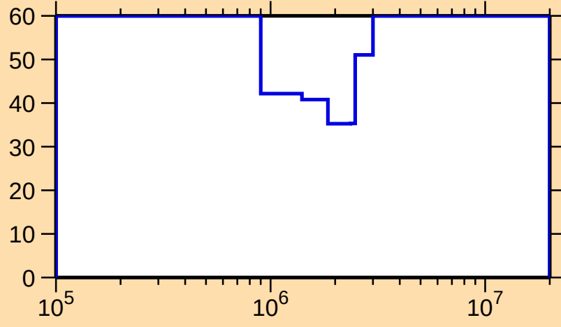
\Delta\sigma/\sigma vs. E for ^{152}\text{Pr}(n,\text{el.})
