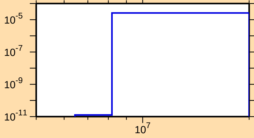
\sigma vs. E for ^{152}\text{Pr}(n,\alpha)
