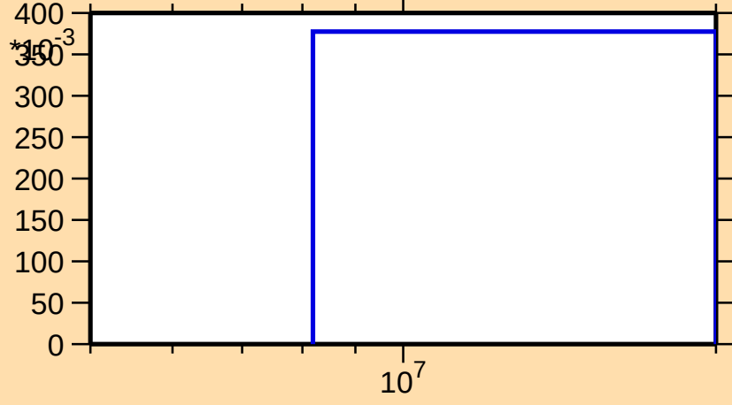
\sigma vs. E for ^{152}\text{Pr}(n,3n)
