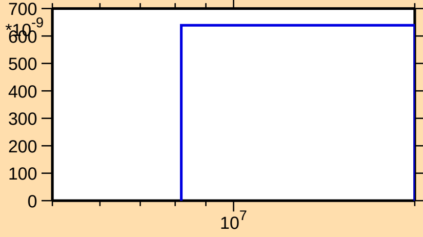
\sigma vs. E for ^{152}\text{Pr}(n,n\alpha)
