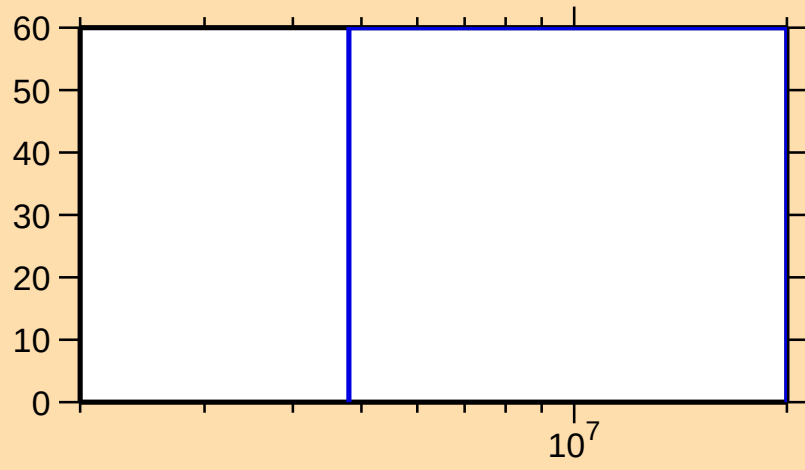
\Delta\sigma/\sigma vs. E for ^{152}\text{Pr}(n,2n)
