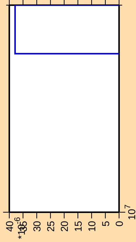
\Delta\sigma/\sigma vs. E for ^{153}\text{Pr}(\text{mt 11})
