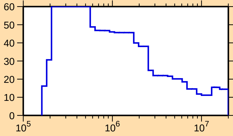
\Delta\sigma/\sigma vs. E for ^{153}\text{Pr}(n,n\text{onel.})
