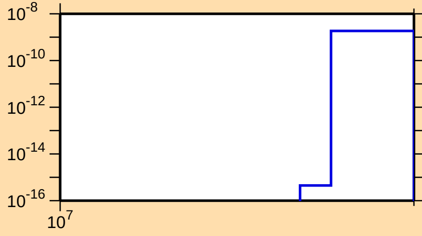
\sigma vs. E for ^{153}\text{Pr}(n,2np)
