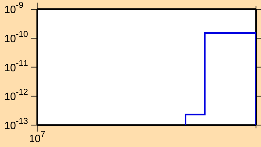
\sigma vs. E for ^{153}\text{Pr}(n,2n\alpha)
