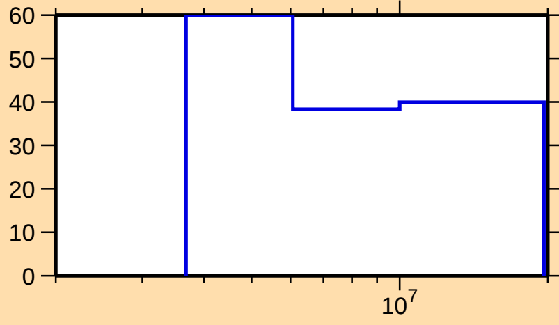
\Delta\sigma/\sigma vs. E for ^{153}\text{Pr}(n,2n)
