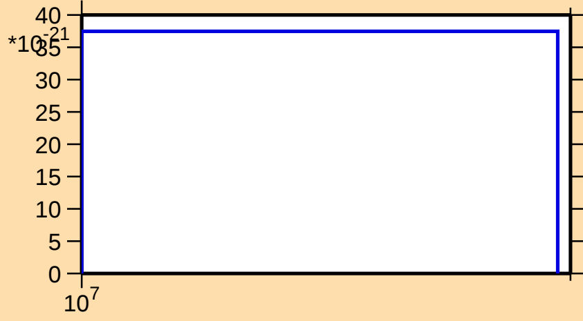
\sigma vs. E for ^{153}\text{Pr}(\text{mt 11})
