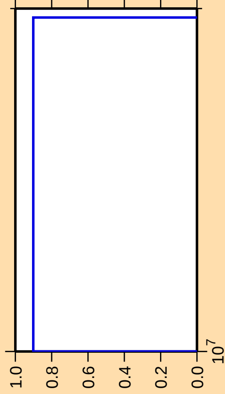
\Delta\sigma/\sigma vs. E for ^{153}\text{Pr}(n,2n\alpha)
