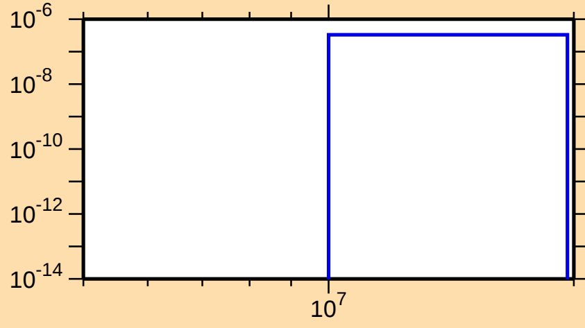
\sigma vs. E for ^{153}\text{Pr}(n,n\alpha)
