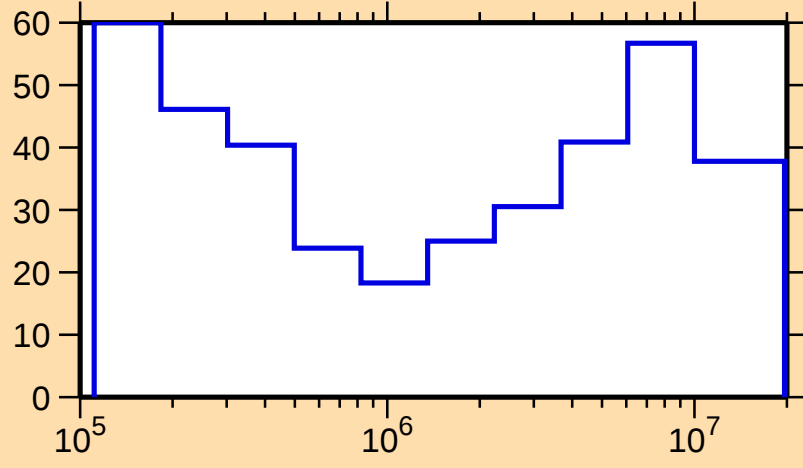
\Delta\sigma/\sigma vs. E for ^{153}\text{Pr}(n,\text{el.})
