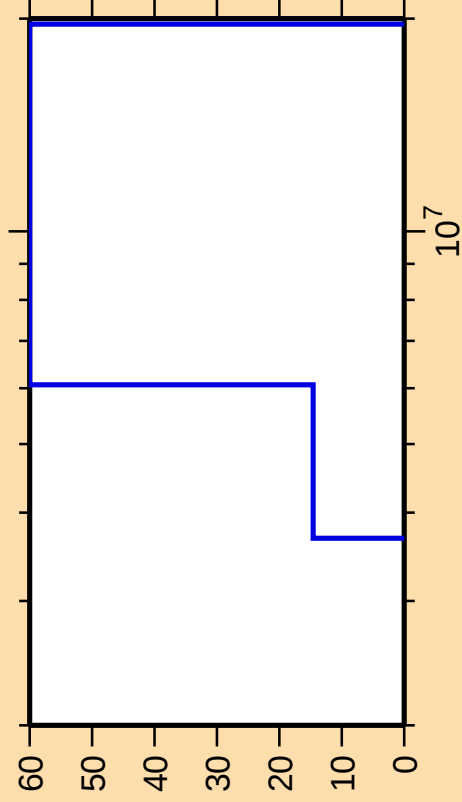
\Delta\sigma/\sigma vs. E for ^{153}\text{Pr}(n,n\text{cont.})
