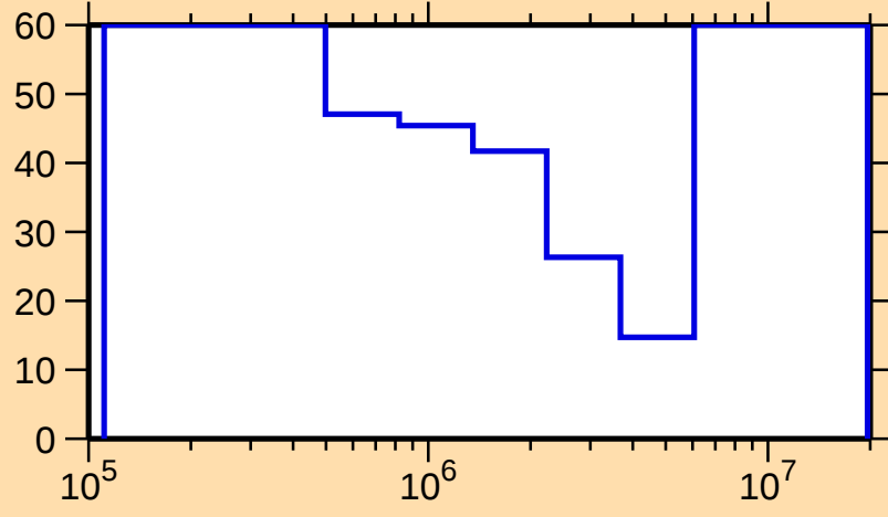
\Delta\sigma/\sigma vs. E for ^{153}\text{Pr}(n,\text{inel.})
