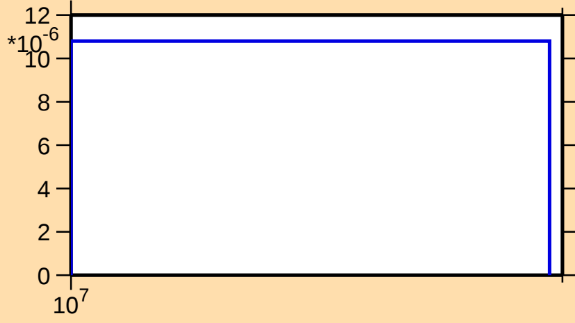
\sigma vs. E for ^{153}\text{Pr}(n,np)
