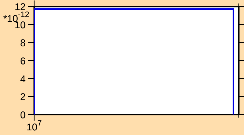
\sigma vs. E for ^{153}\text{Pr}(n,2np)
