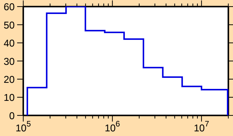
\Delta\sigma/\sigma vs. E for ^{153}\text{Pr}(n,\text{nonel.})
