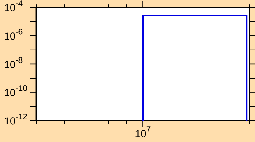
\sigma vs. E for ^{153}\text{Pr}(n,d)
